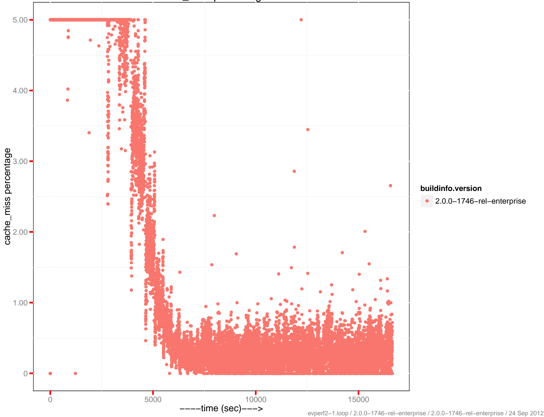
cache_miss percentage 0-5
