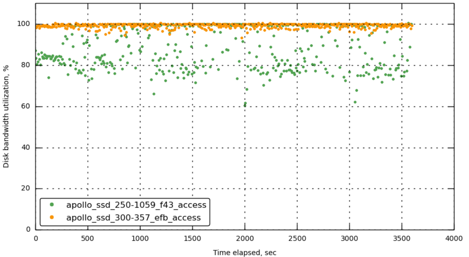
[172.23.96.15] data_util
