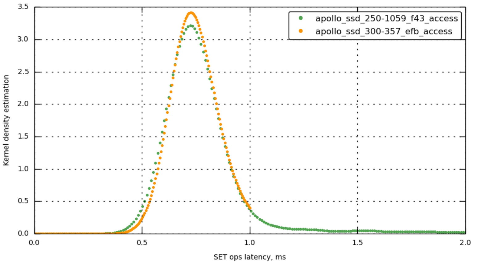
[bucket-1] latency_set
