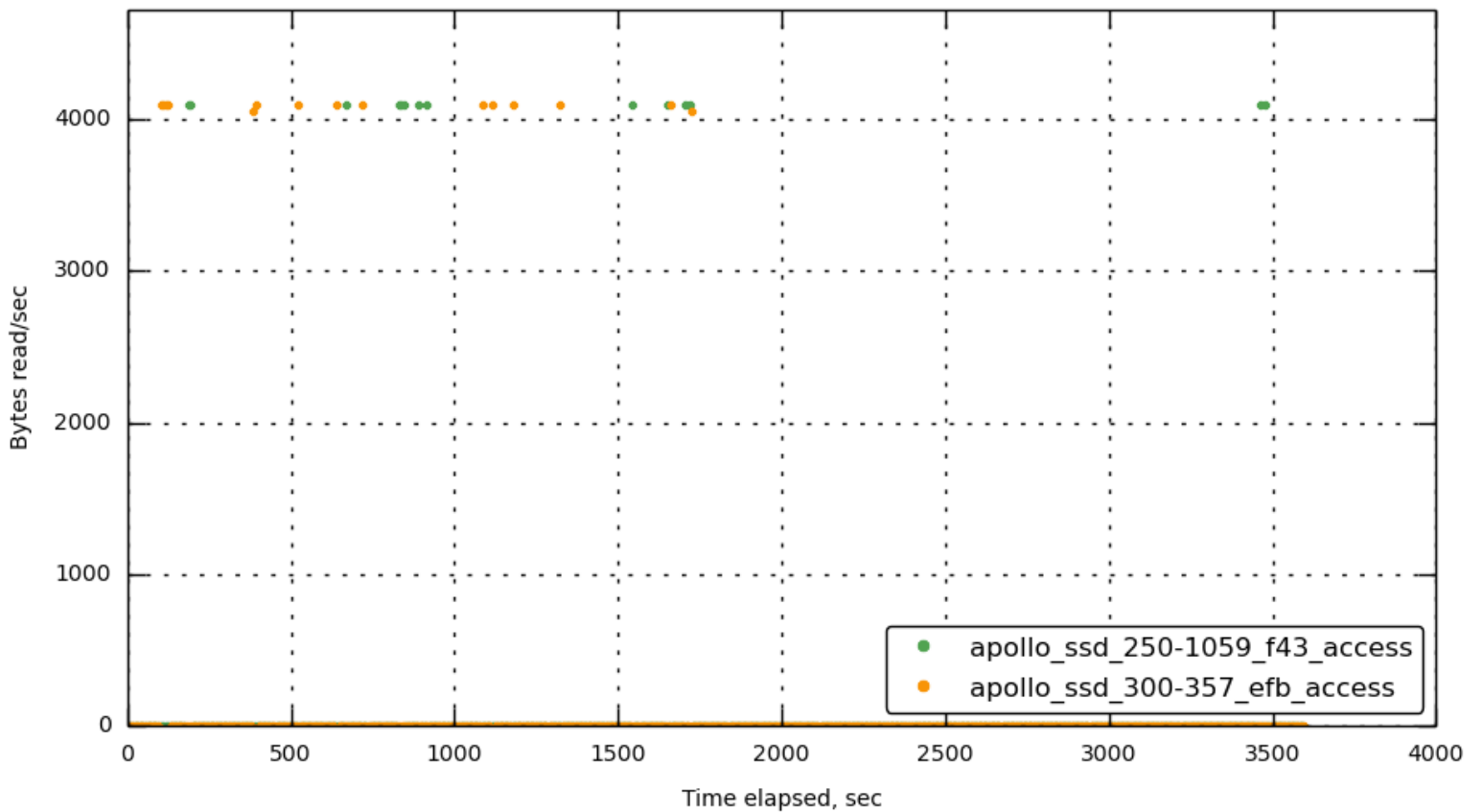
[172.23.96.16] data_rbps
