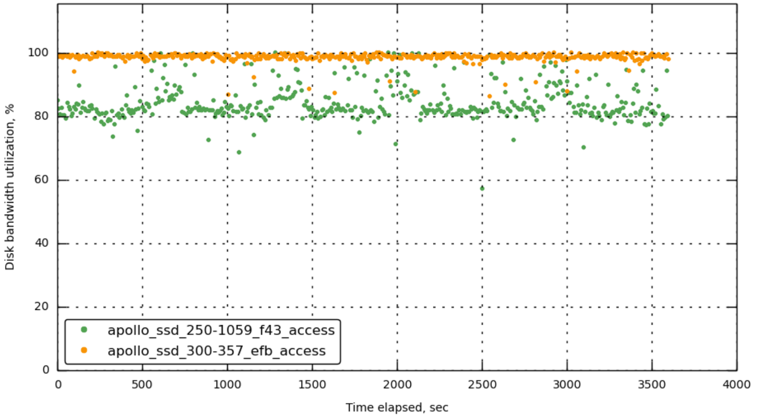
[172.23.96.18] data_util
