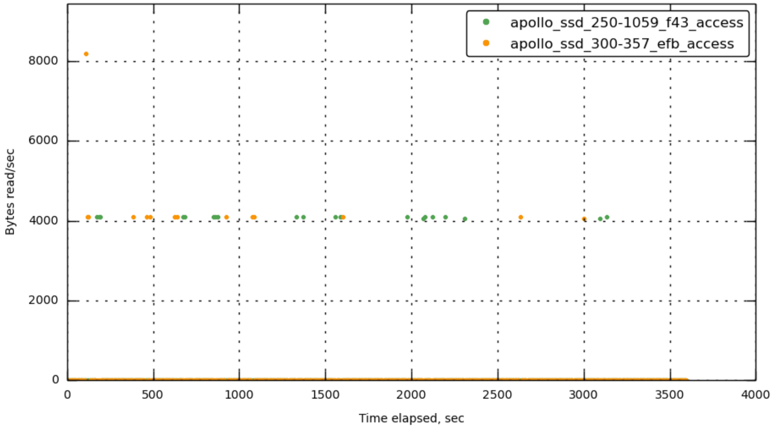
[172.23.96.18] data_rbps
