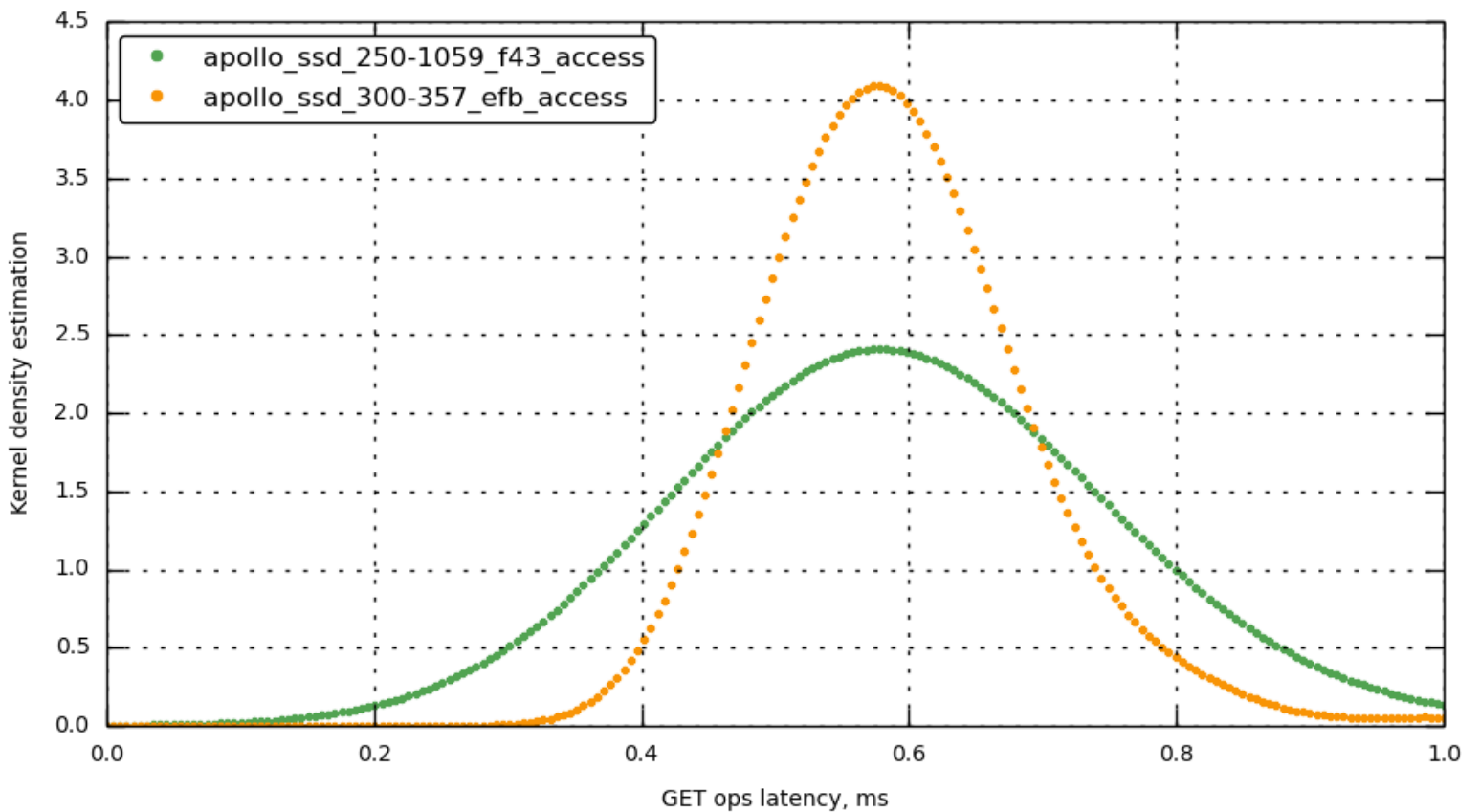
[bucket-1] latency_get
