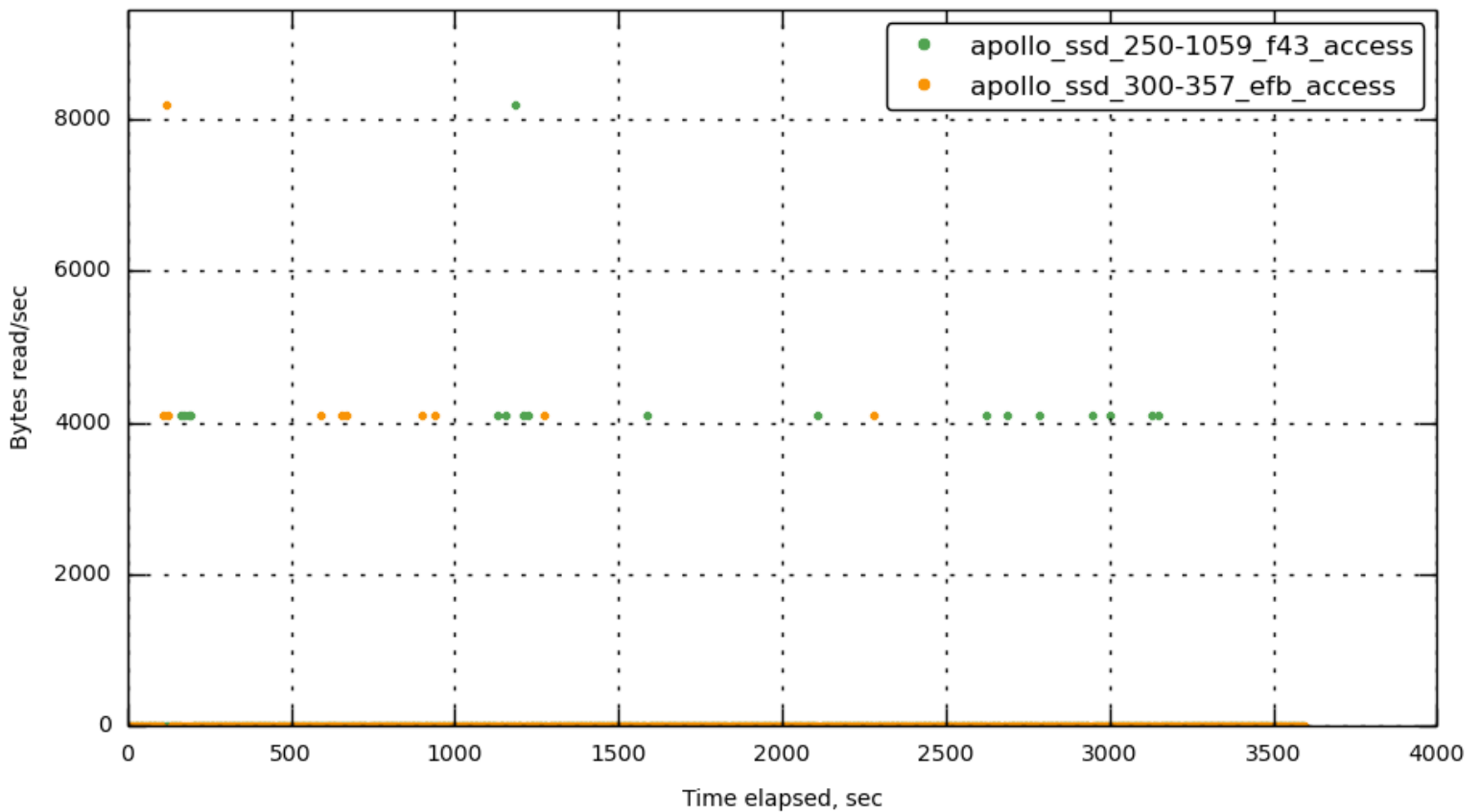
[172.23.96.15] data_rbps
