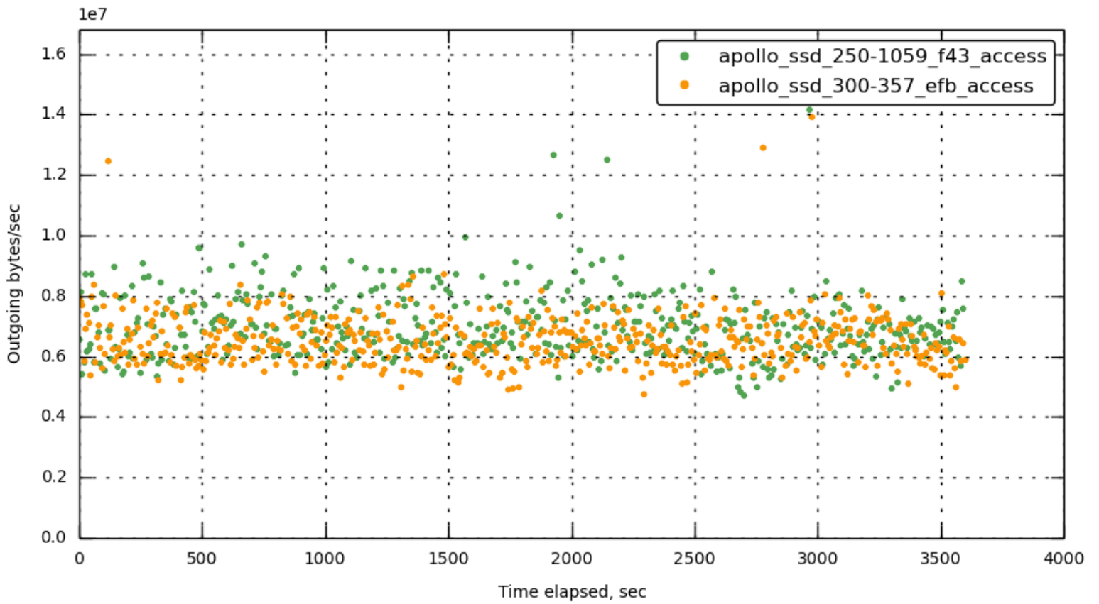
[172.23.96.17] out_bytes_per_sec
