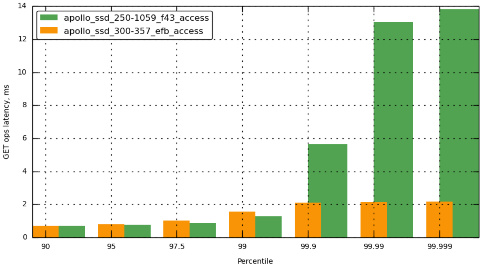
[bucket-1] latency_get
