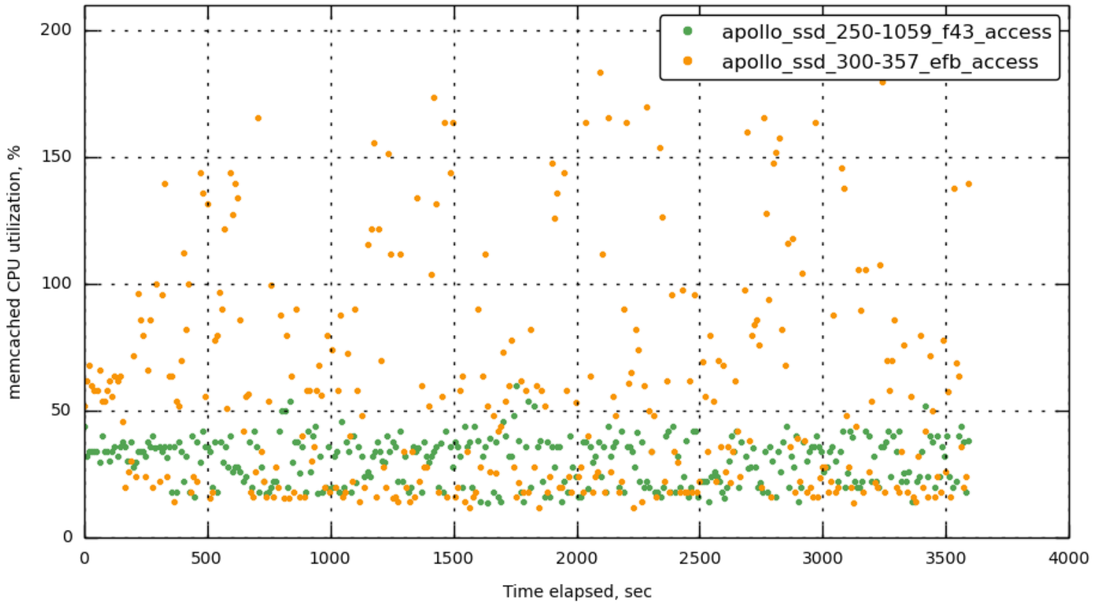
[172.23.96.17] memcached_cpu
