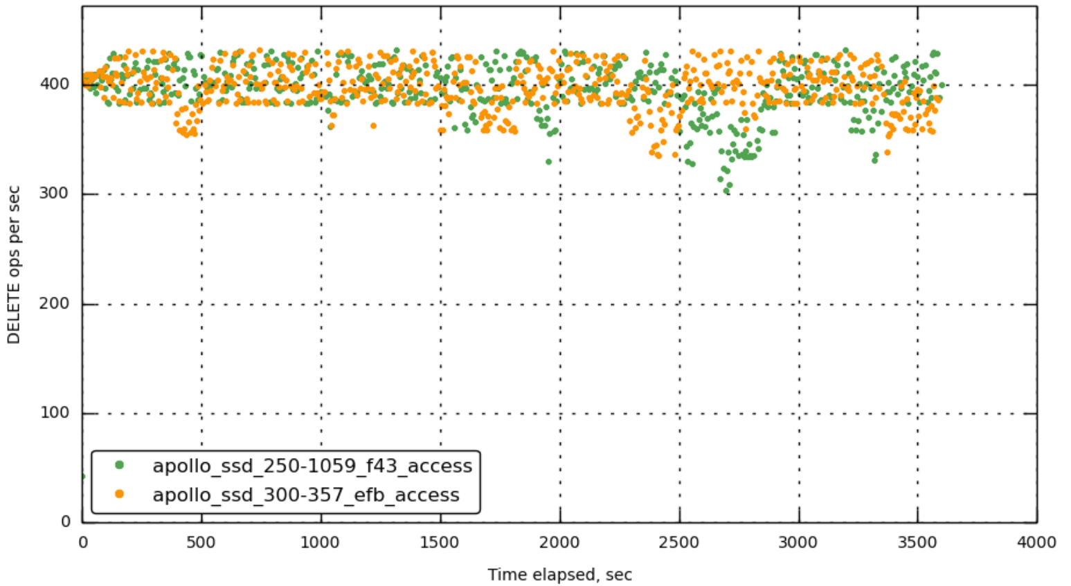
[bucket-1] delete_hits
