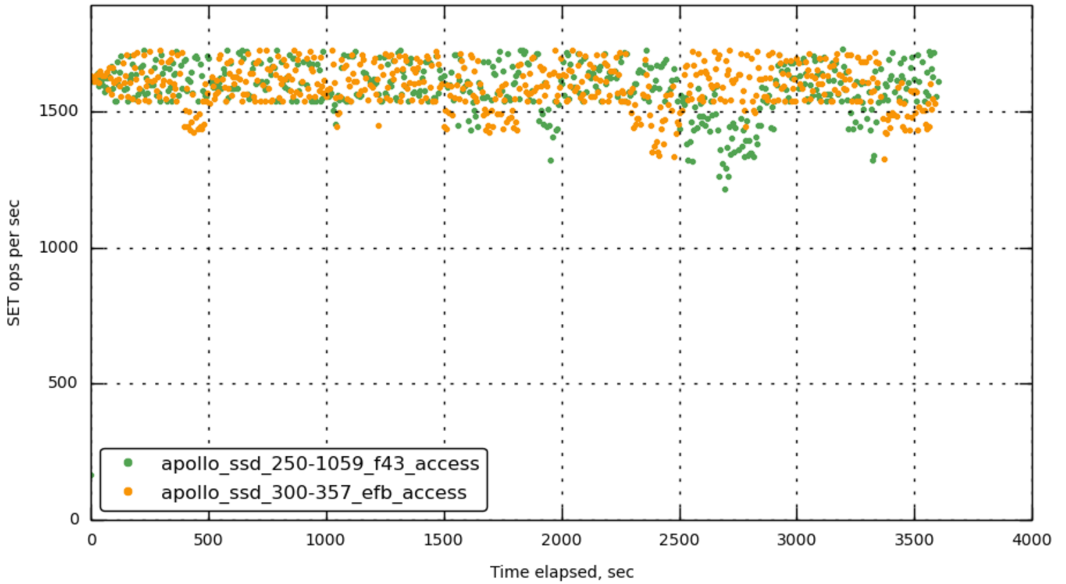
[bucket-1] cmd_set
