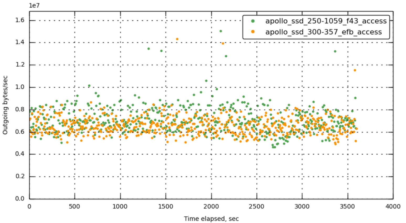
[172.23.96.16] out_bytes_per_sec
