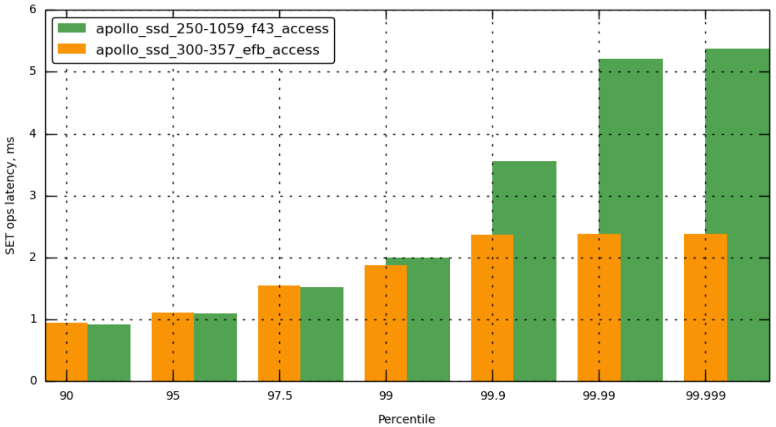
[bucket-1] latency_set
