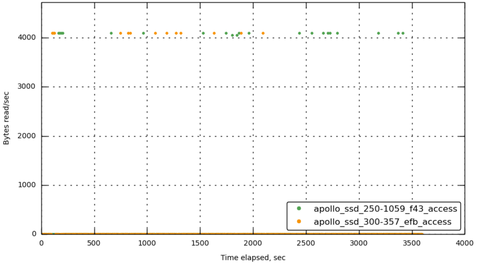
[172.23.96.17] data_rbps
