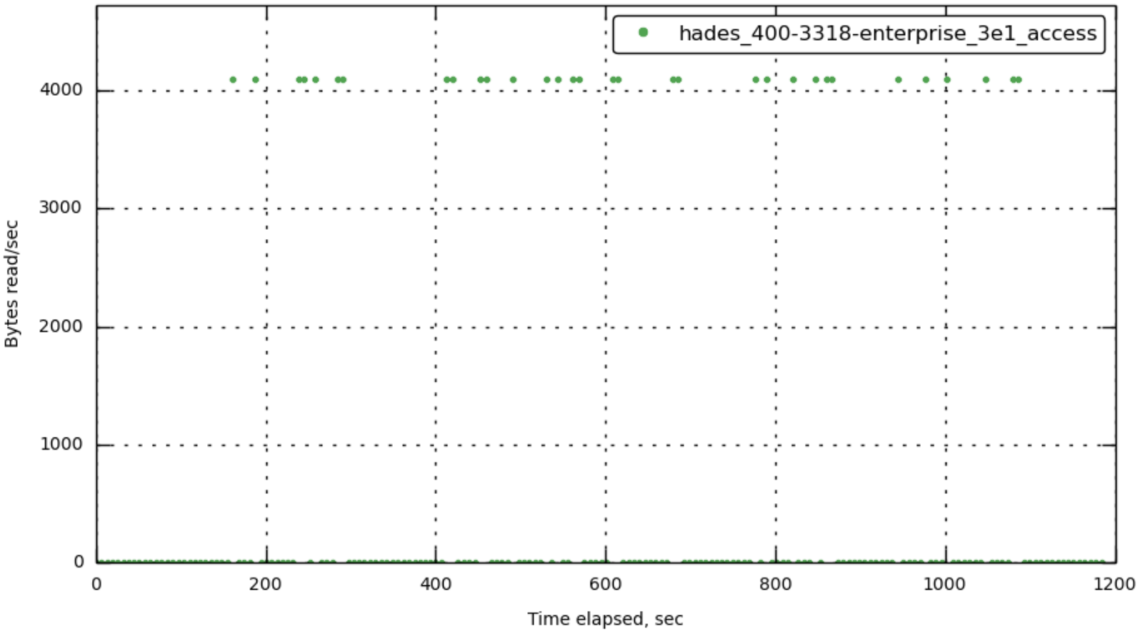
[172.23.100.73] data_rbps
