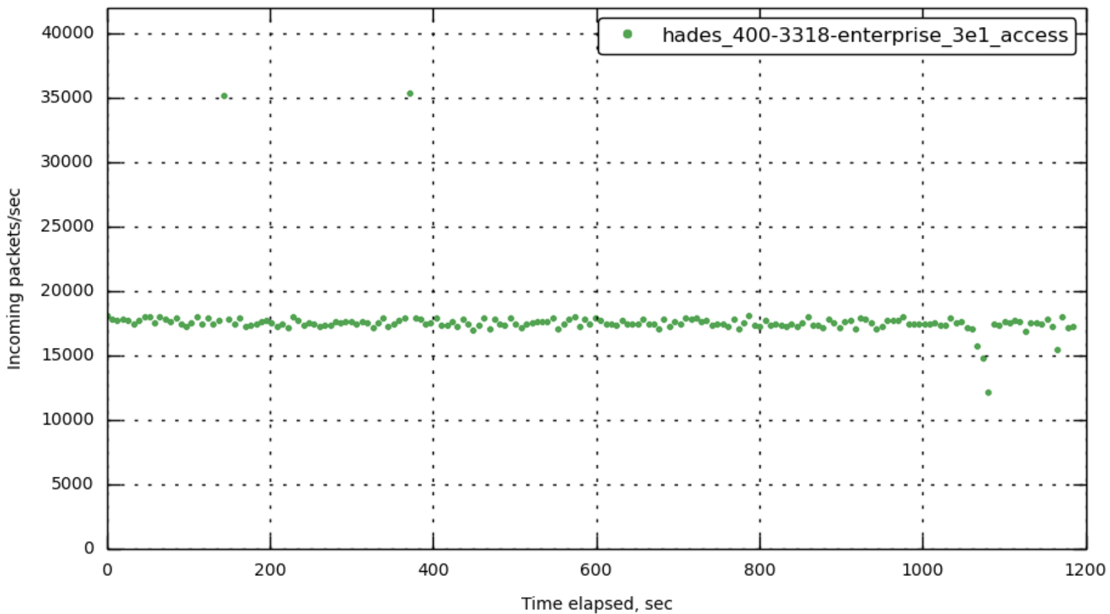
[172.23.100.55] in_packets_per_sec
