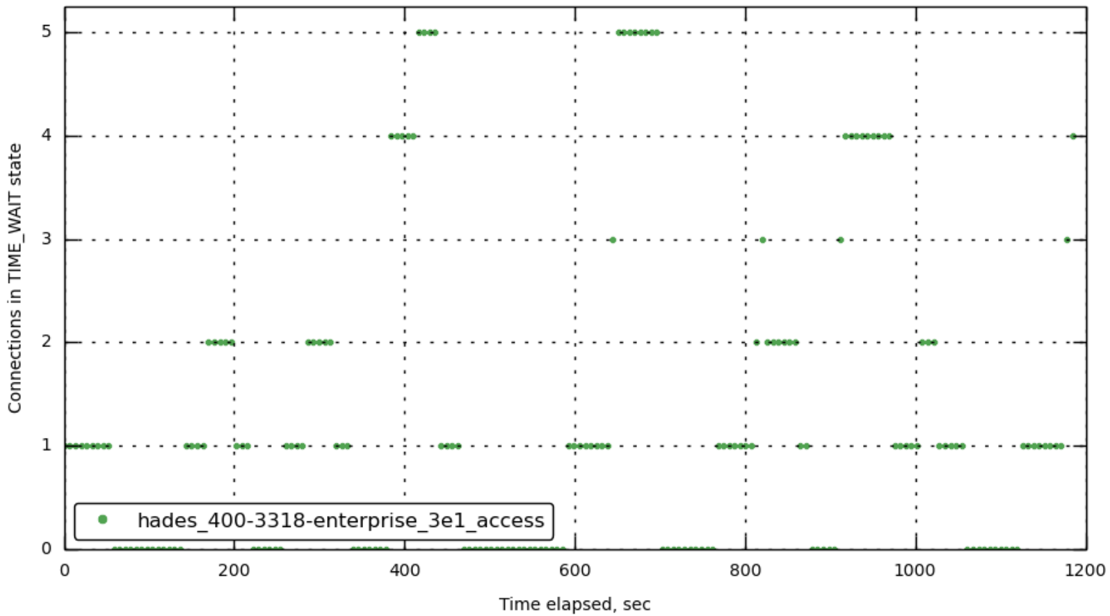
[172.23.100.73] TIME_WAIT
