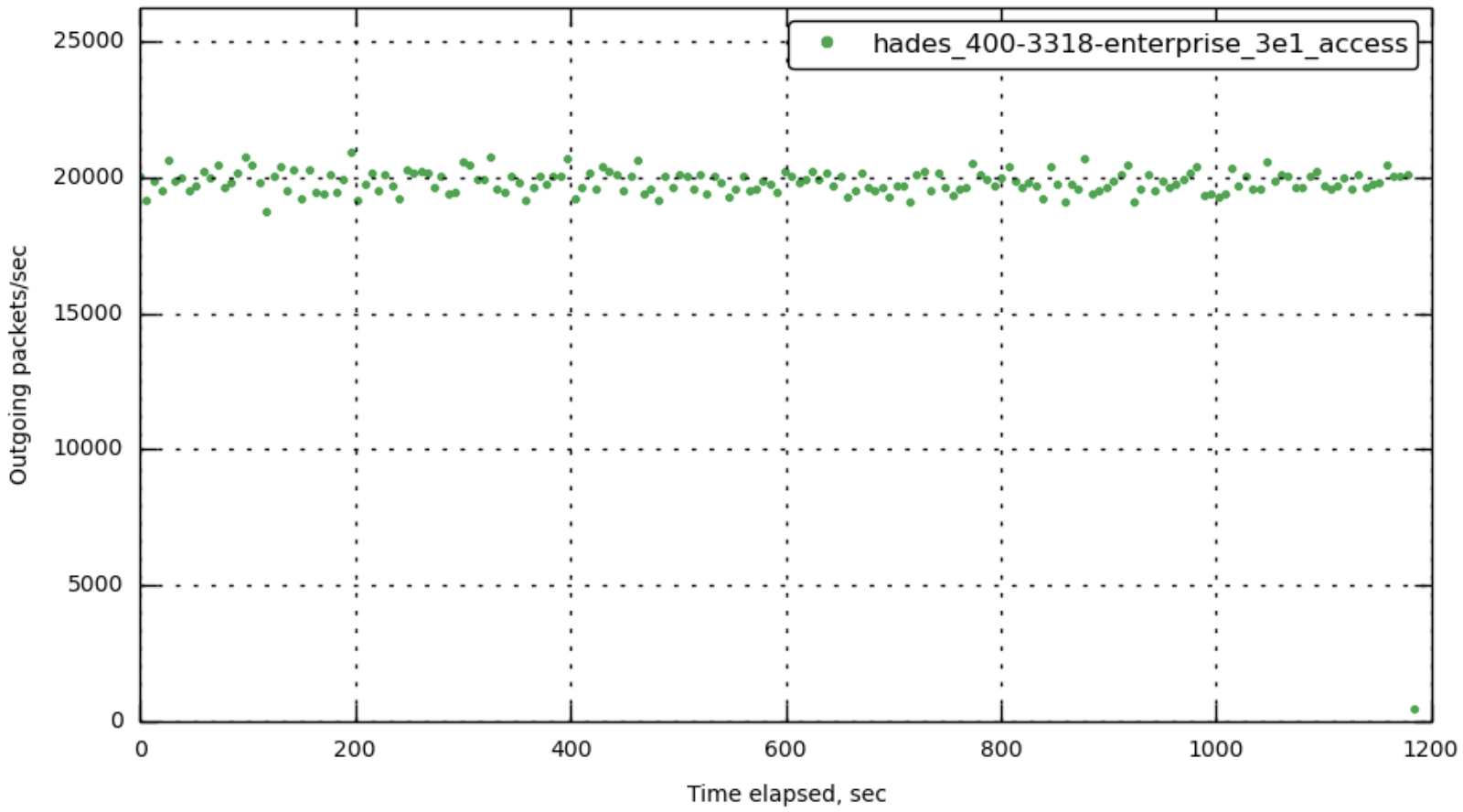
[172.23.100.70] out_packets_per_sec
