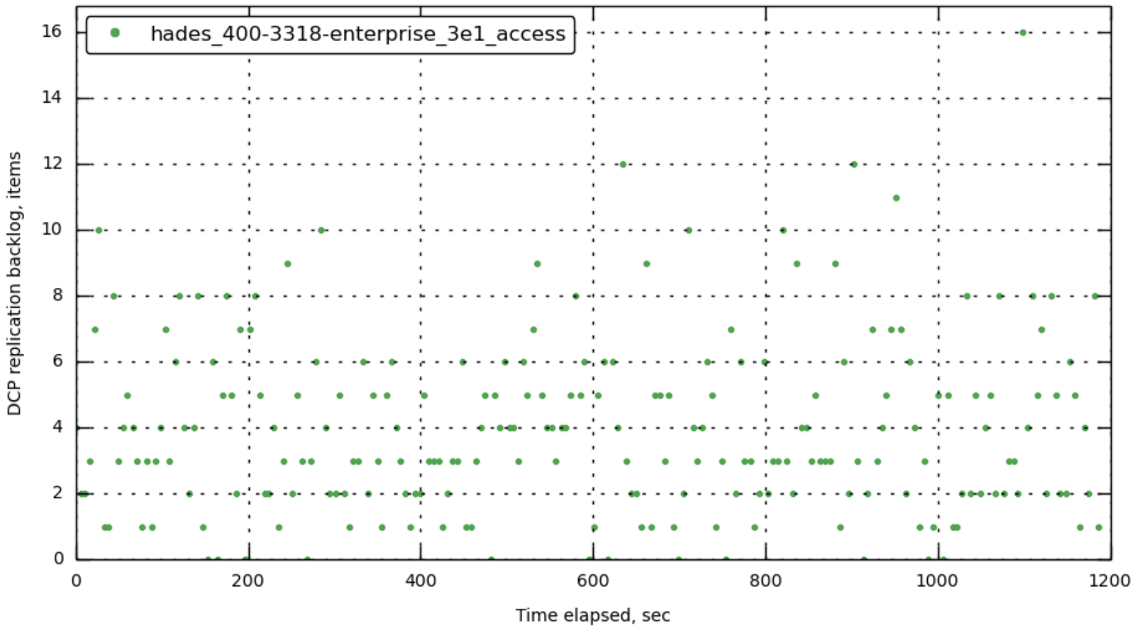
[bucket-1] ep_dcp_replica_items_remaining
