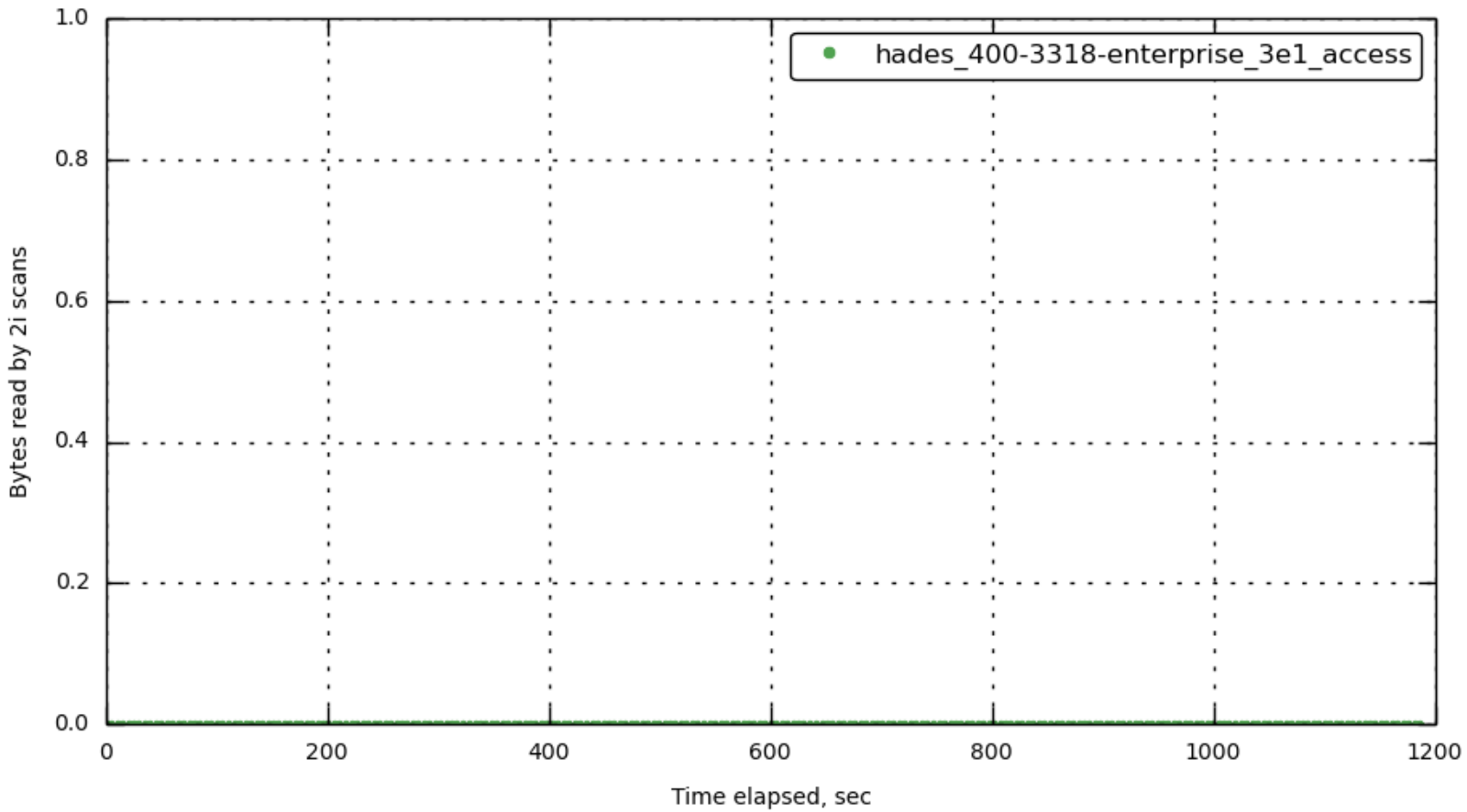
[bucket-1] index_scan_bytes_read
