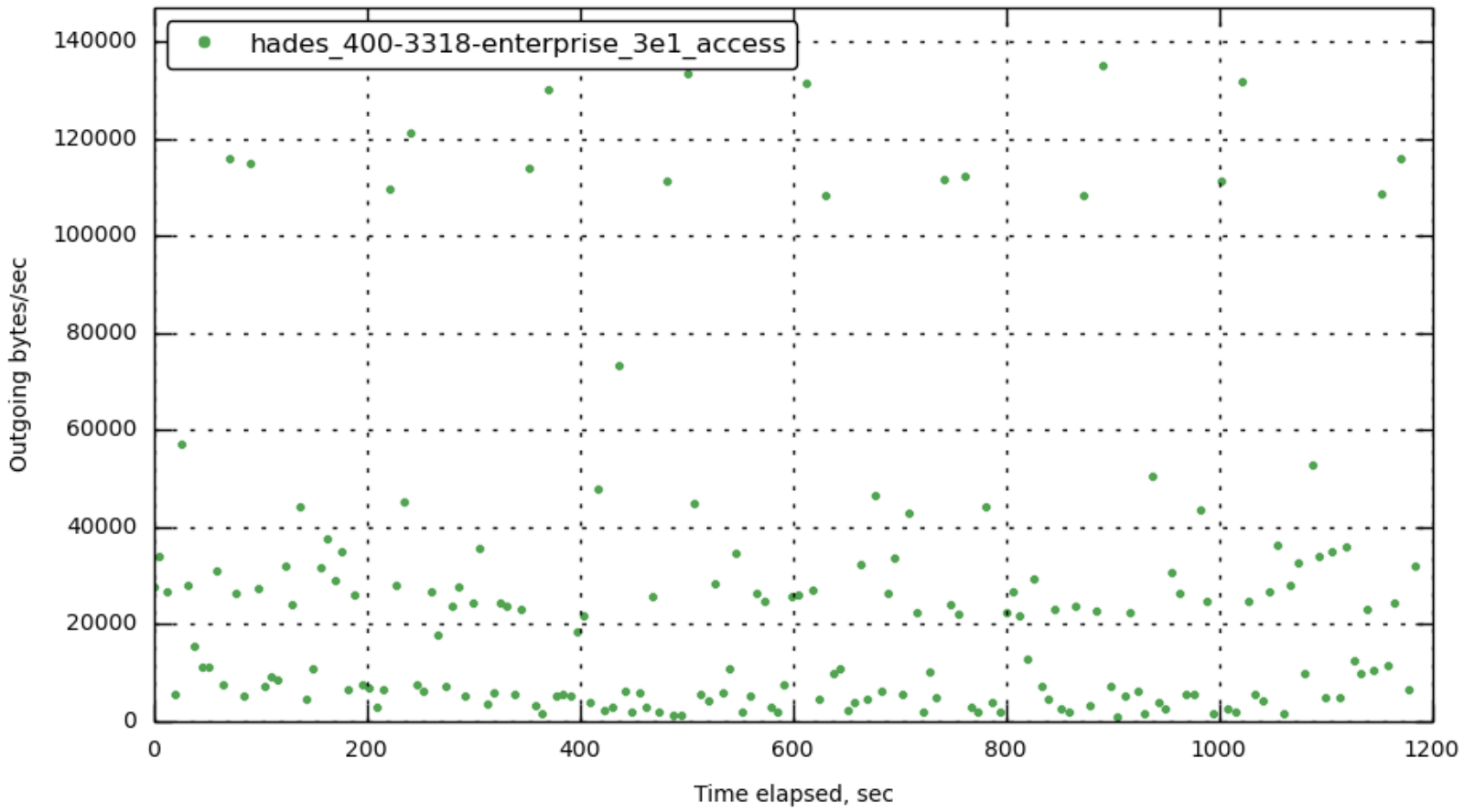
[172.23.100.45] out_bytes_per_sec
