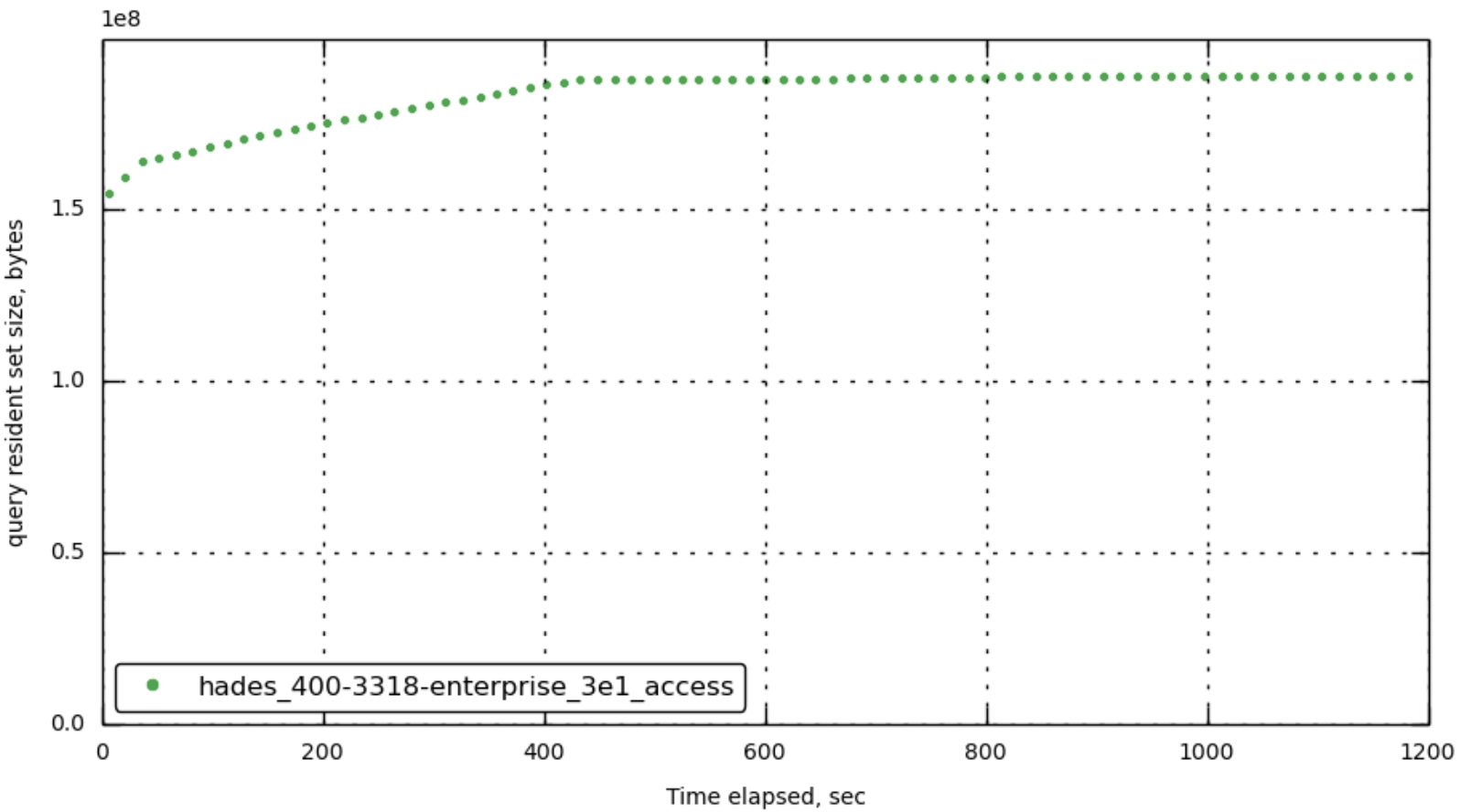
[172.23.100.55] cbq-engine_rss
