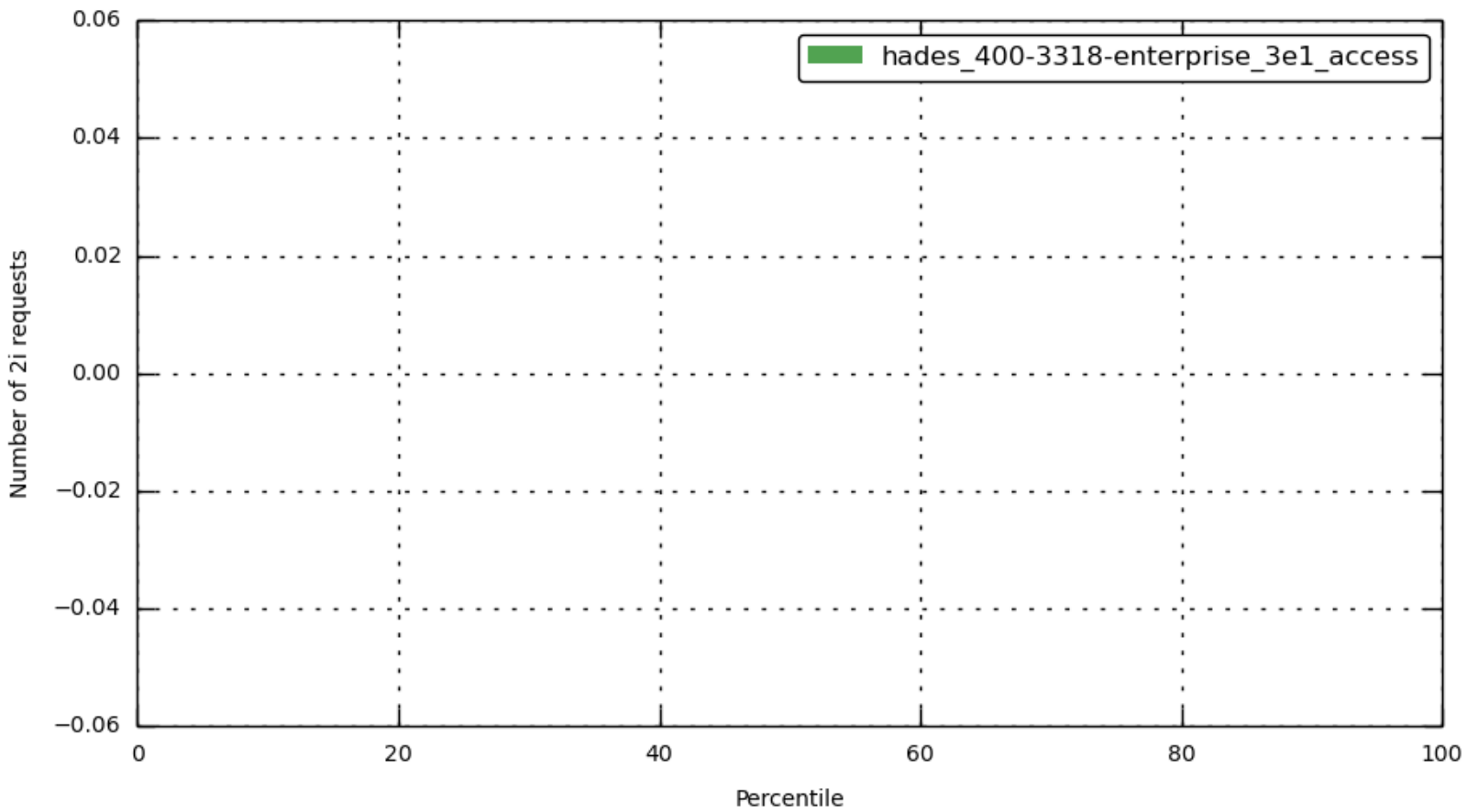
[bucket-1] index_num_requests
