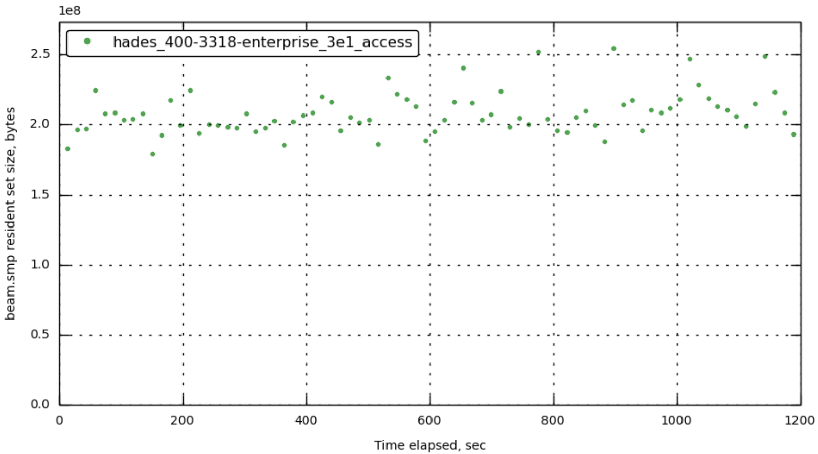
[172.23.100.70] beam.smp_rss
