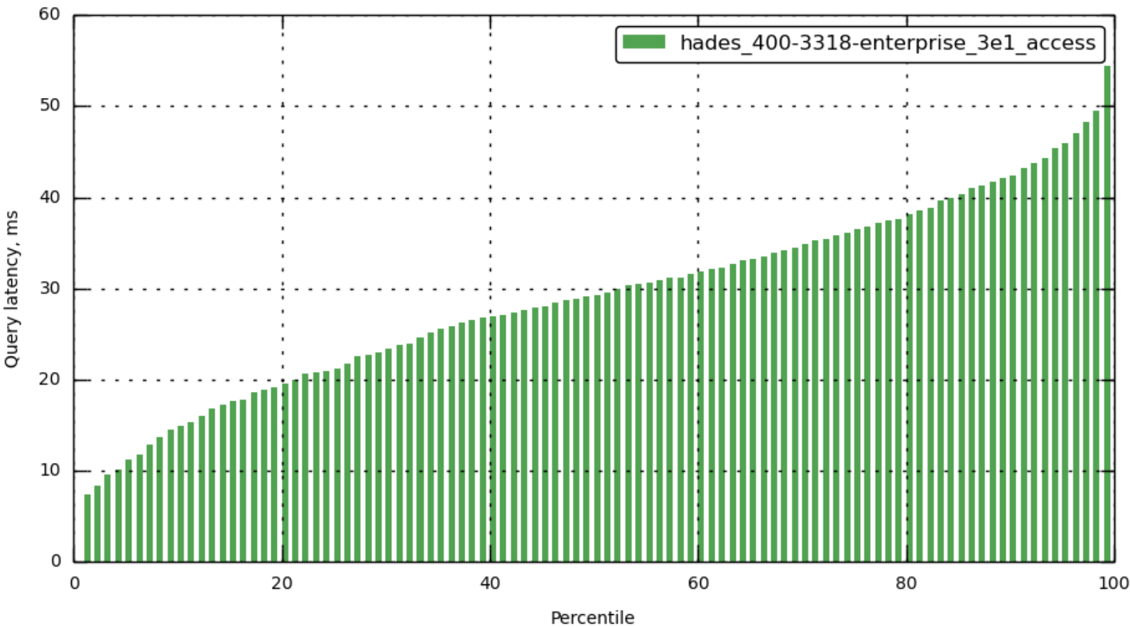
[bucket-1] latency_query
