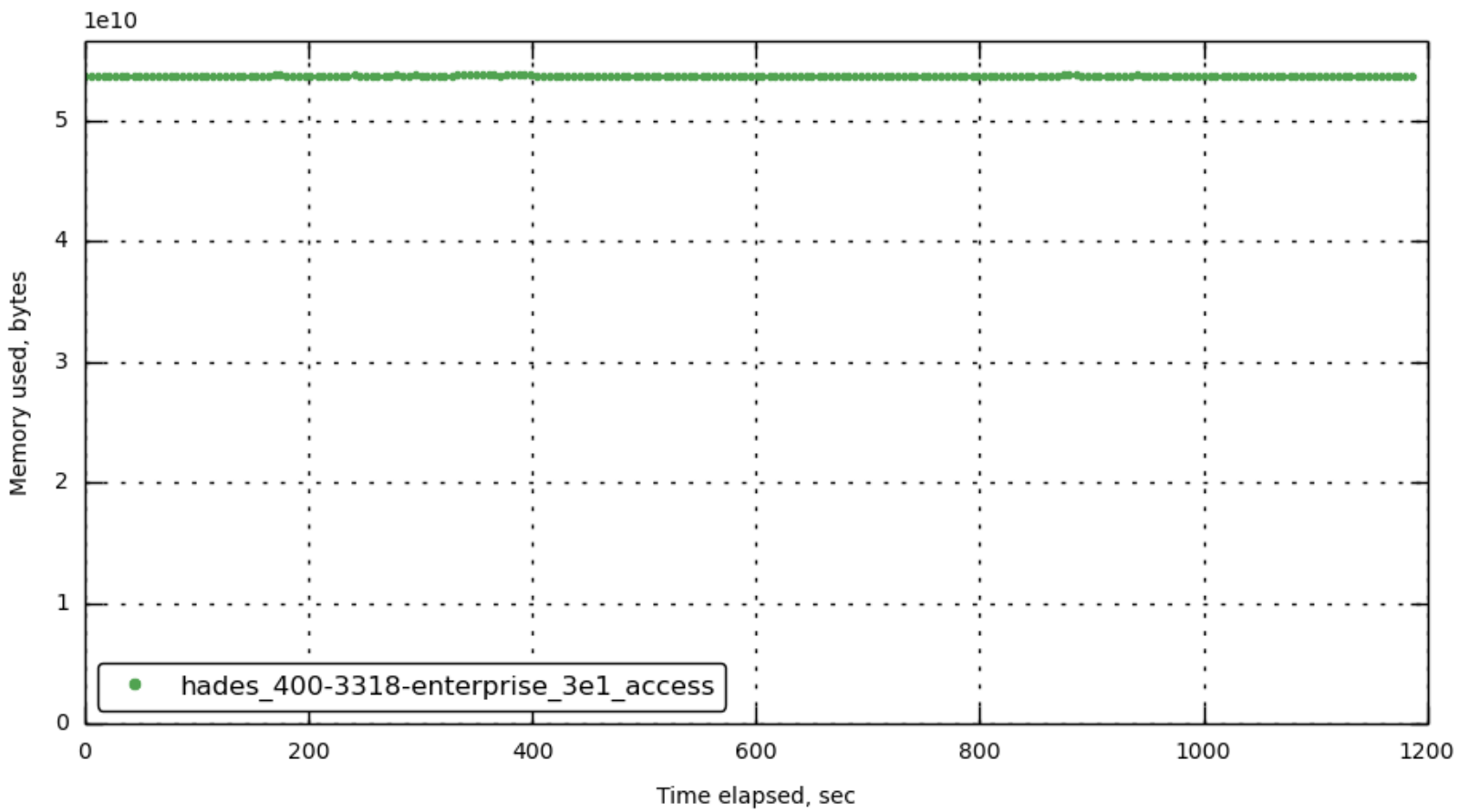
[bucket-1] mem_used
