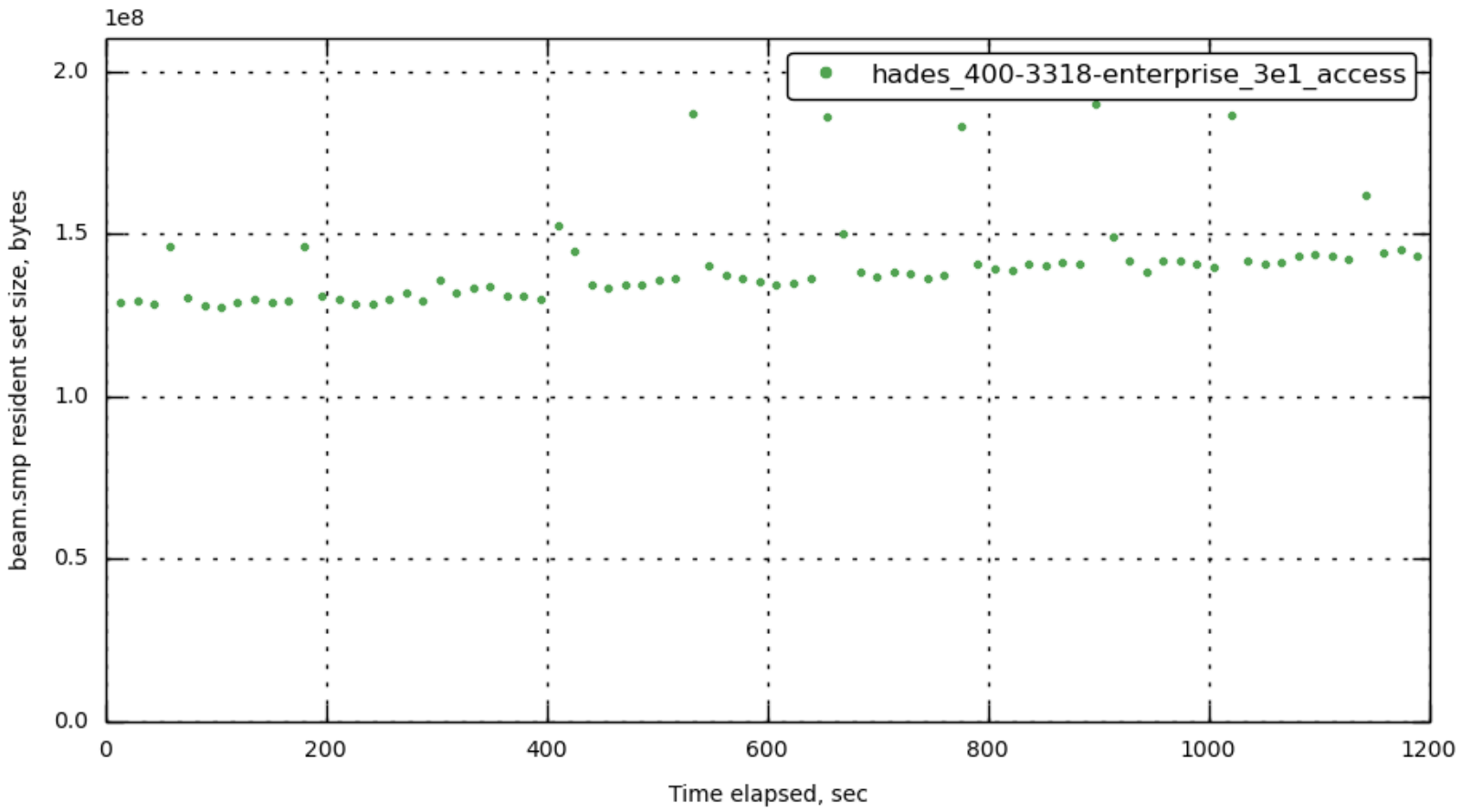
[172.23.100.73] beam.smp_rss
