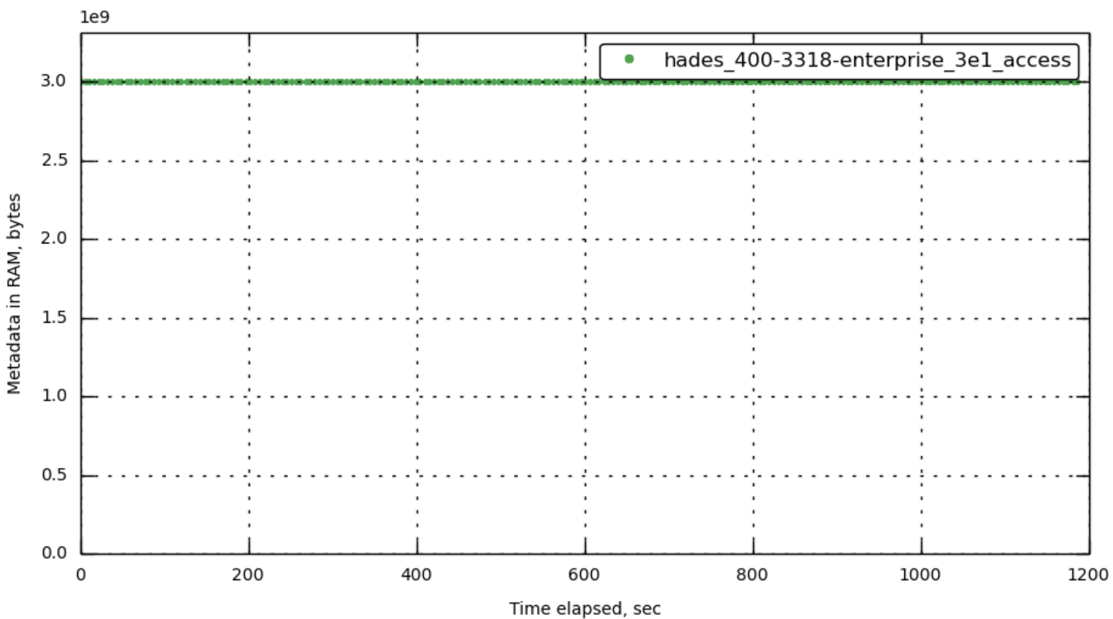
[bucket-1] ep_meta_data_memory
