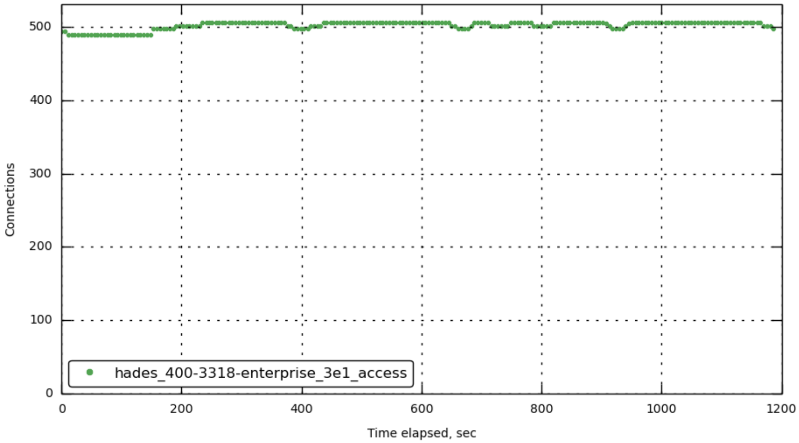
[bucket-1] curr_connections
