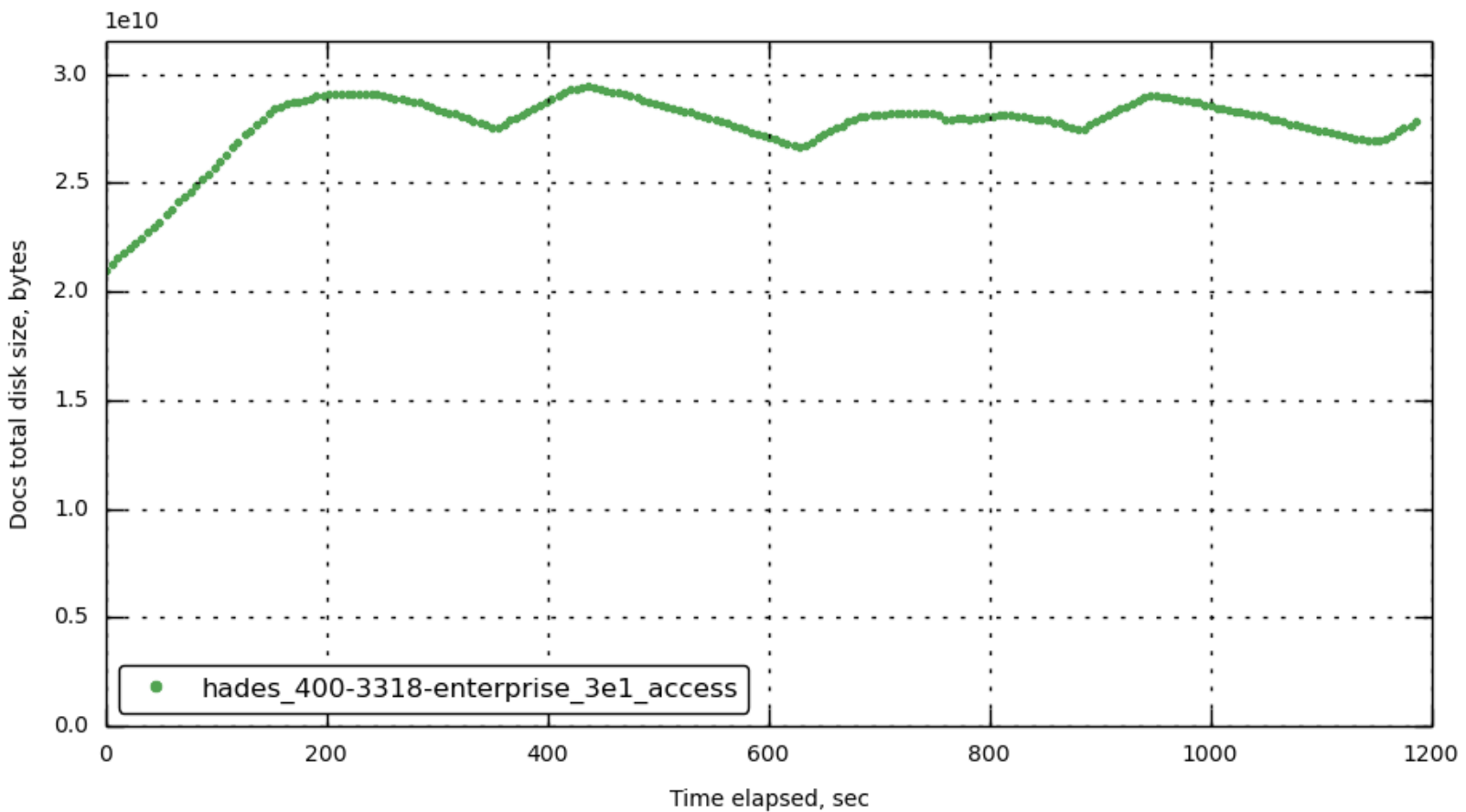
[bucket-1] couch_docs_actual_disk_size
