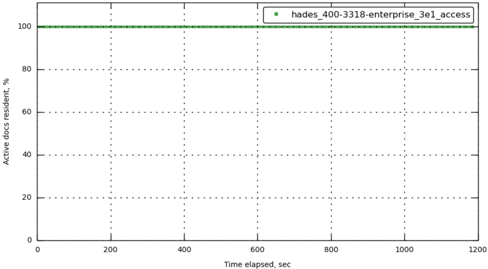
[bucket-1] vb_active_resident_items_ratio
