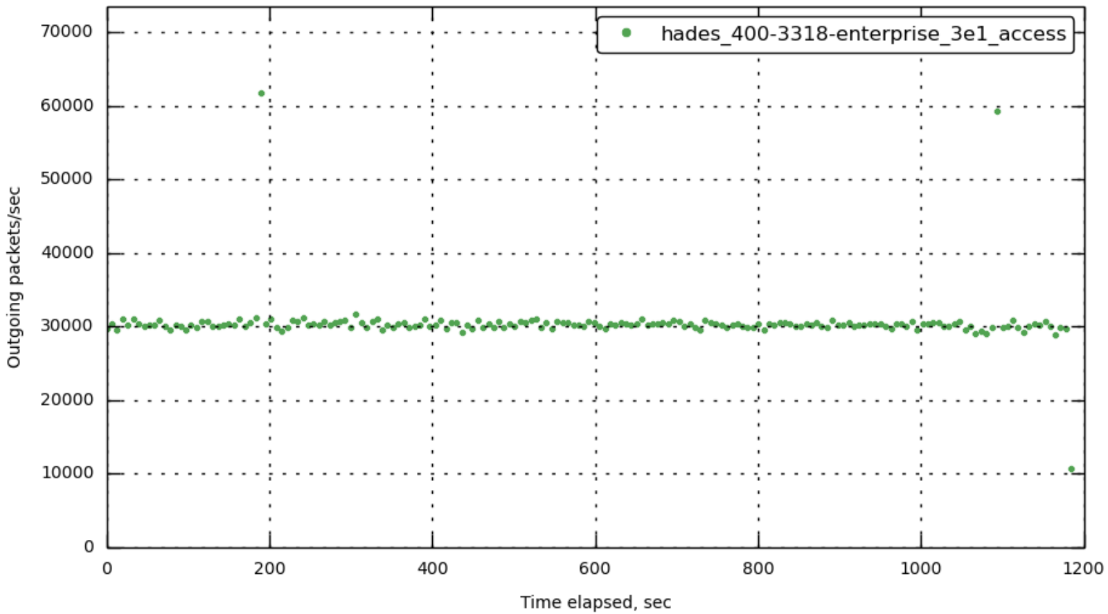
[172.23.100.71] out_packets_per_sec
