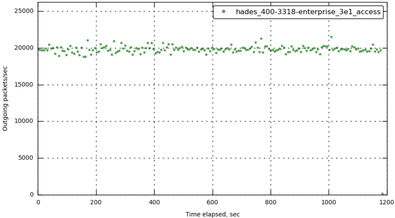
[172.23.100.72] out_packets_per_sec
