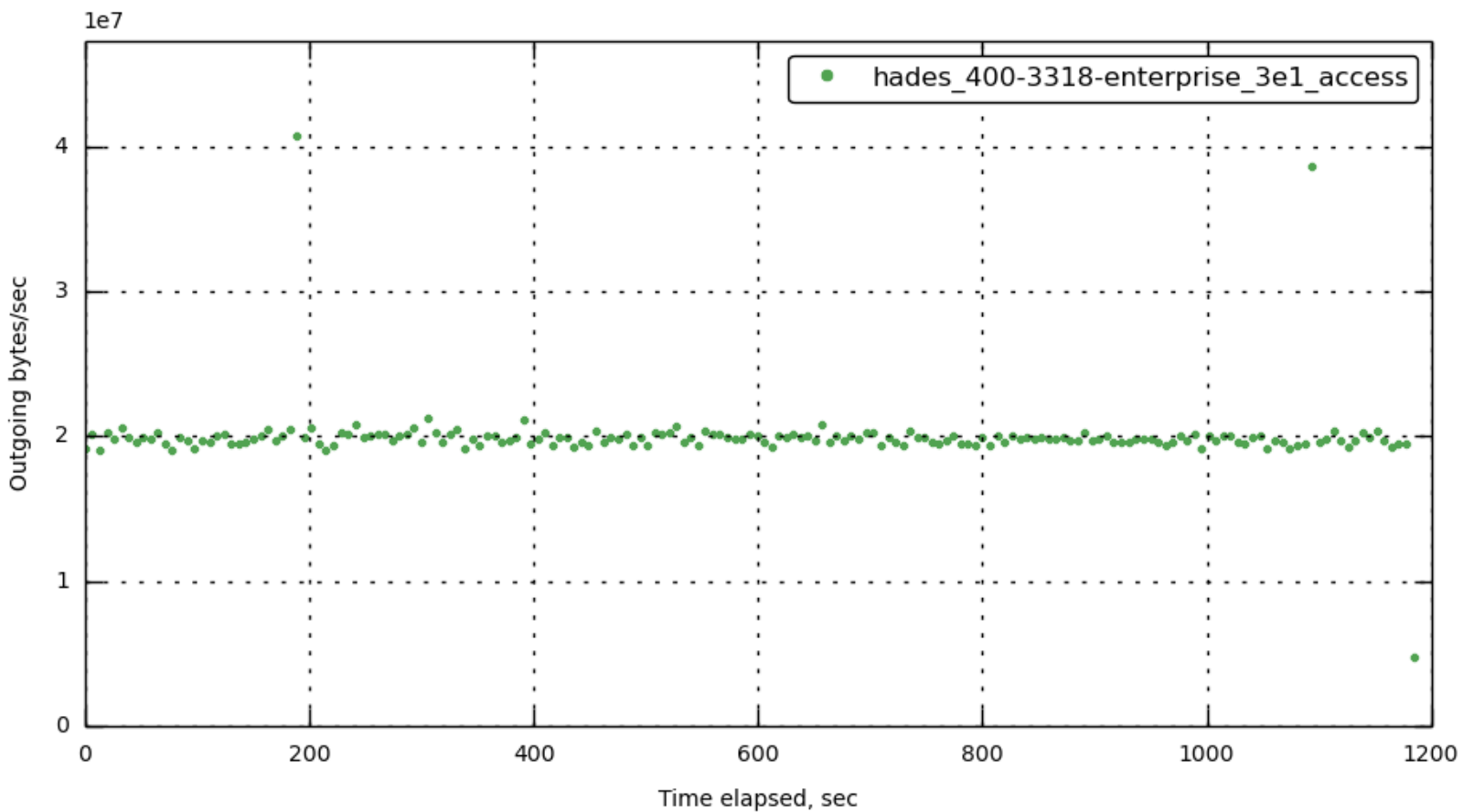
[172.23.100.71] out_bytes_per_sec
