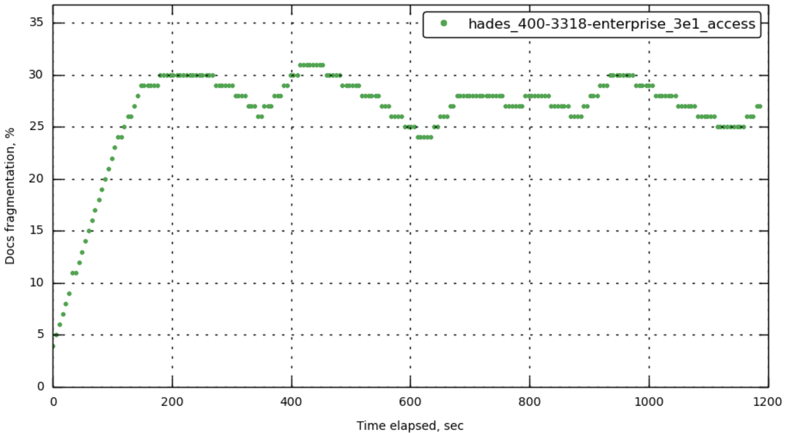
[bucket-1] couch_docs_fragmentation
