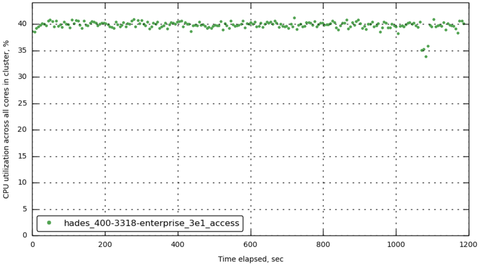
[bucket-1] cpu_utilization_rate
