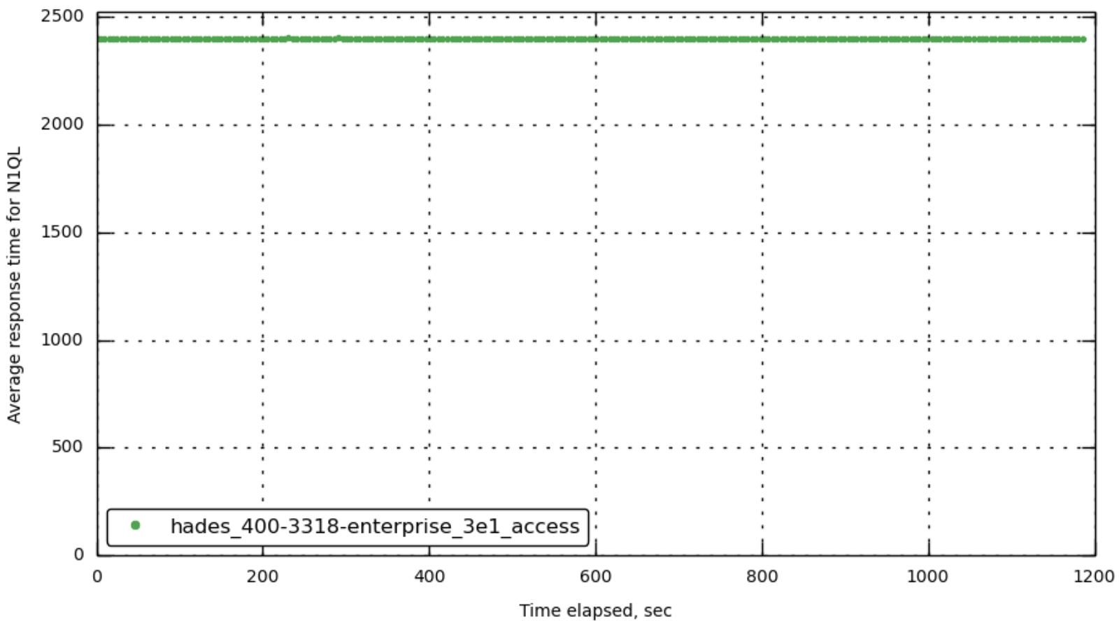
query_avg_response_size
