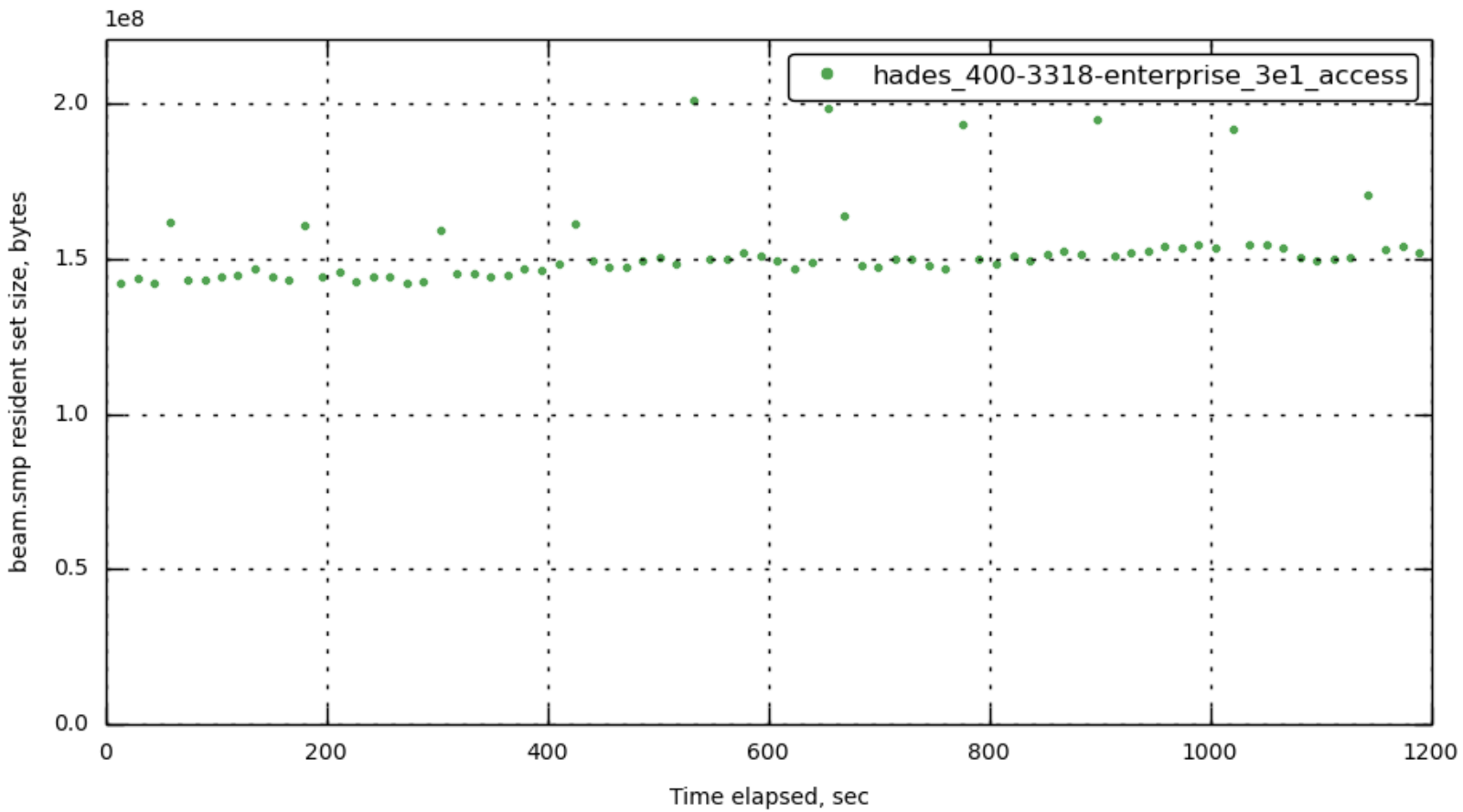
[172.23.100.72] beam.smp_rss
