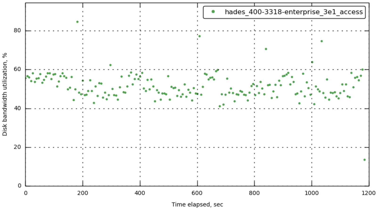
[172.23.100.73] data_util
