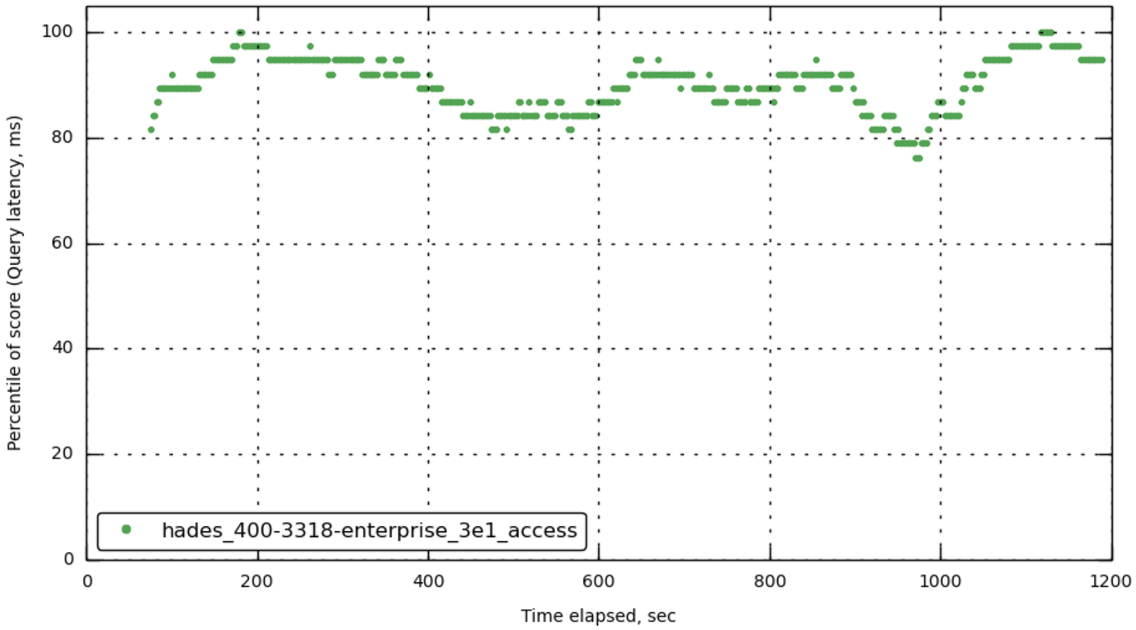
[bucket-1] latency_query
