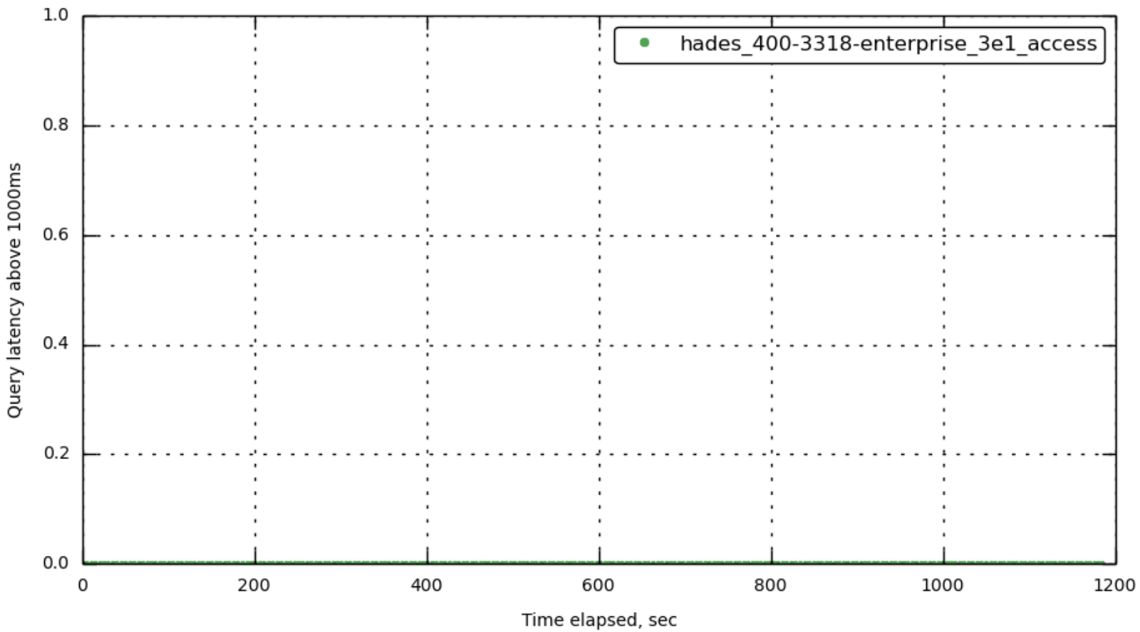
query_requests_1000ms
