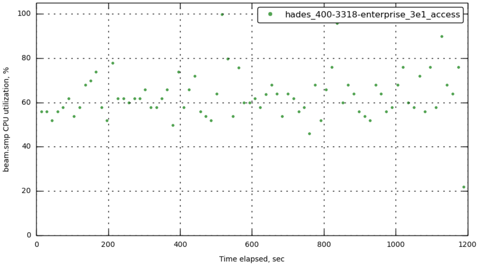
[172.23.100.72] beam.smp_cpu
