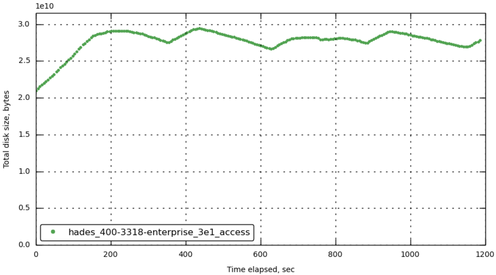
[bucket-1] couch_total_disk_size
