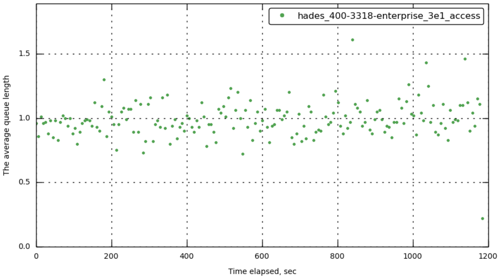
[172.23.100.73] data_avgqusz
