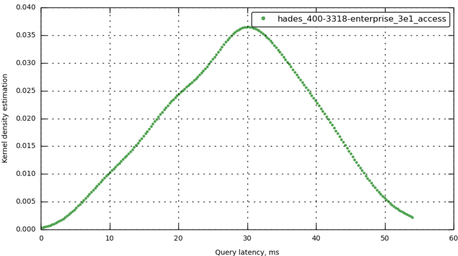
[bucket-1] latency_query
