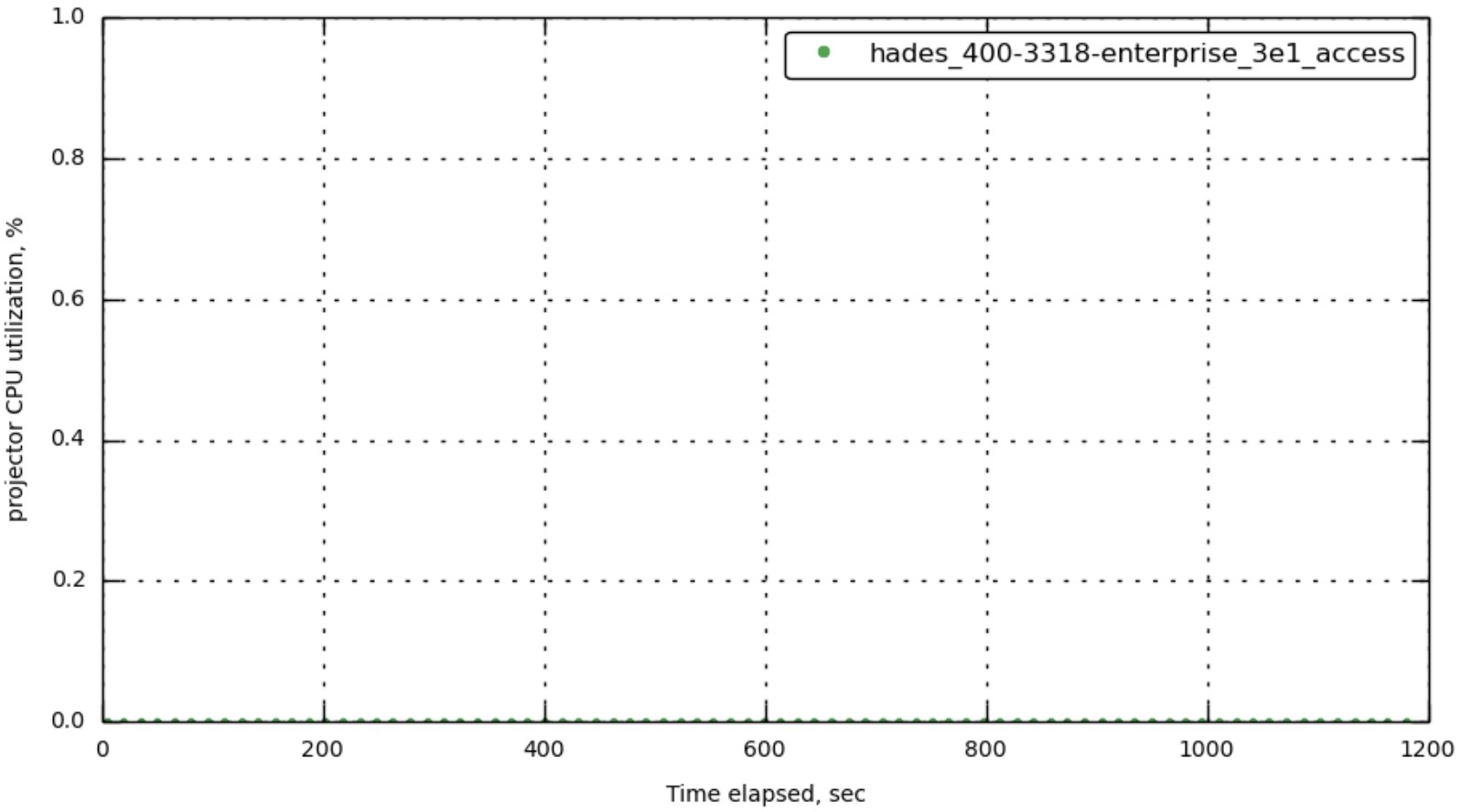
[172.23.100.73] projector_cpu
