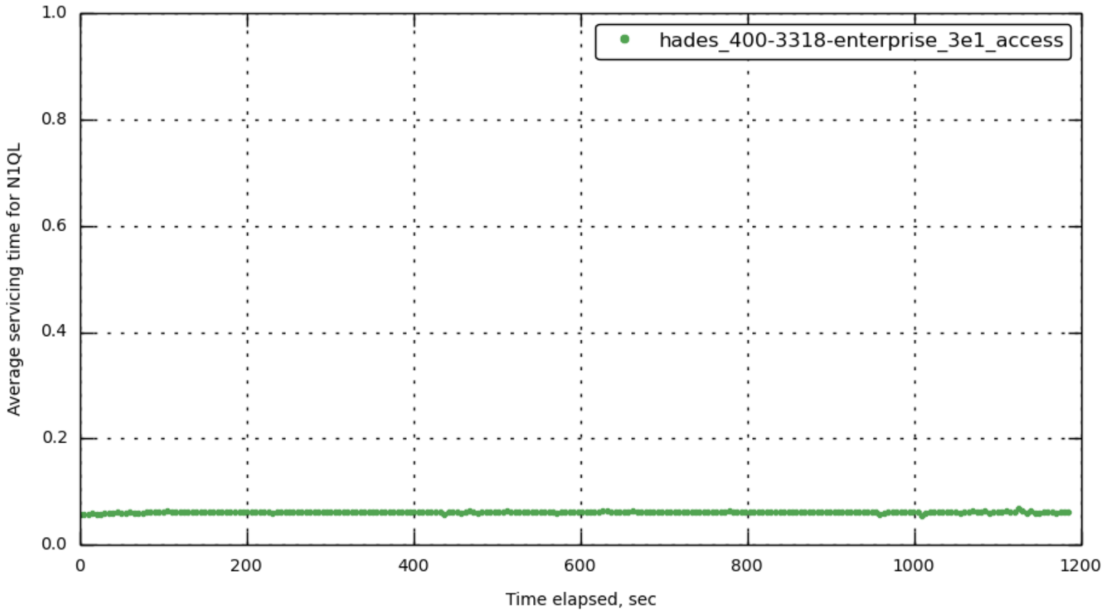
query_avg_svc_time
