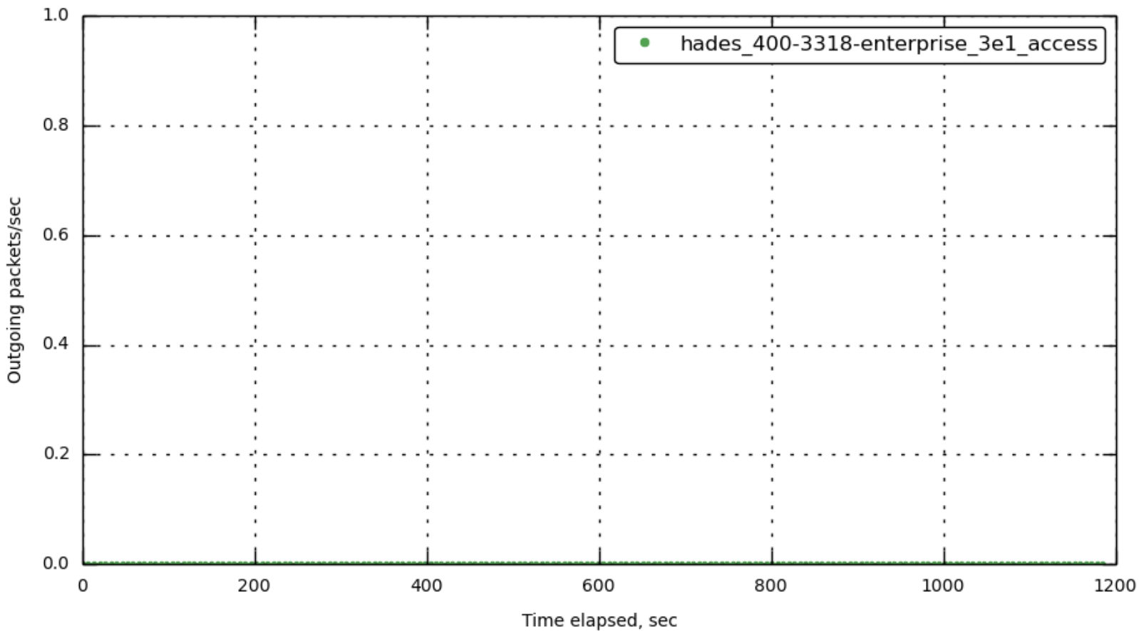
[172.23.100.73] out_packets_per_sec
