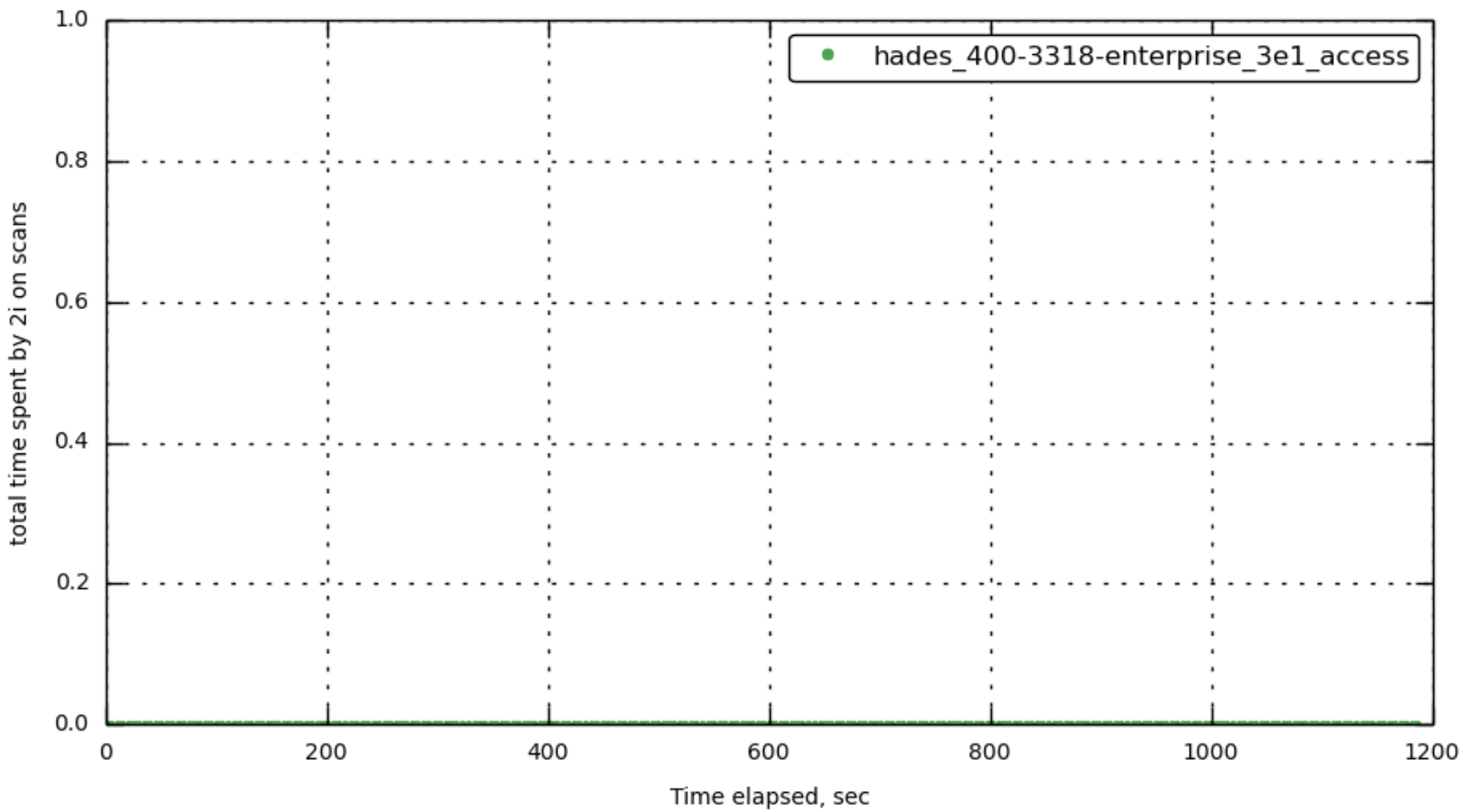
[bucket-1] index_total_scan_duration
