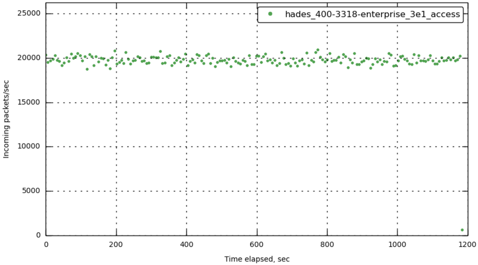
[172.23.100.70] in_packets_per_sec
