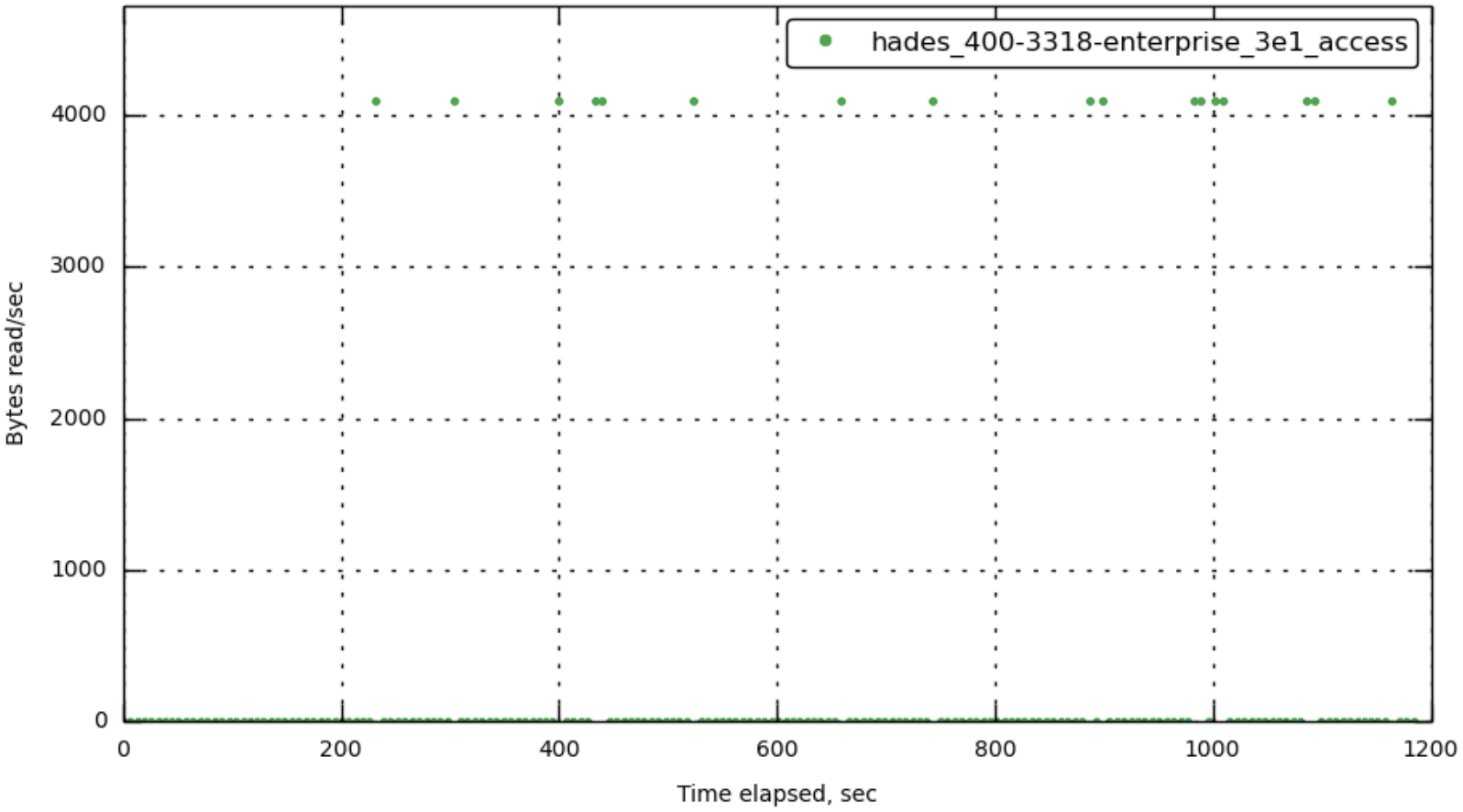
[172.23.100.72] data_rbps
