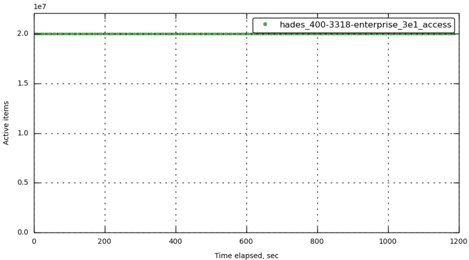
[bucket-1] curr_items
