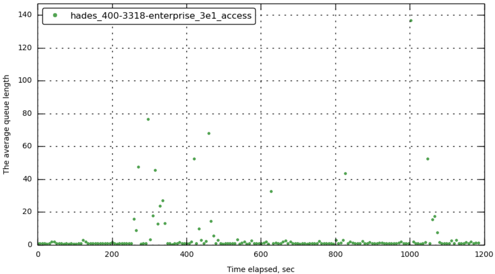
[172.23.100.71] data_avgqusz
