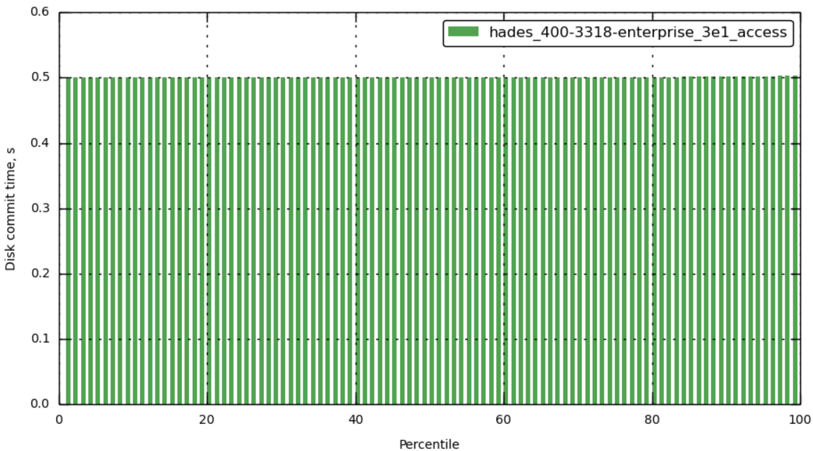
[bucket-1] avg_disk_commit_time
