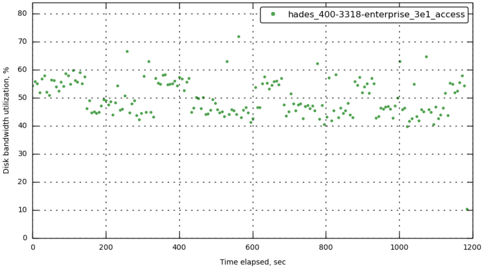
[172.23.100.70] data_util
