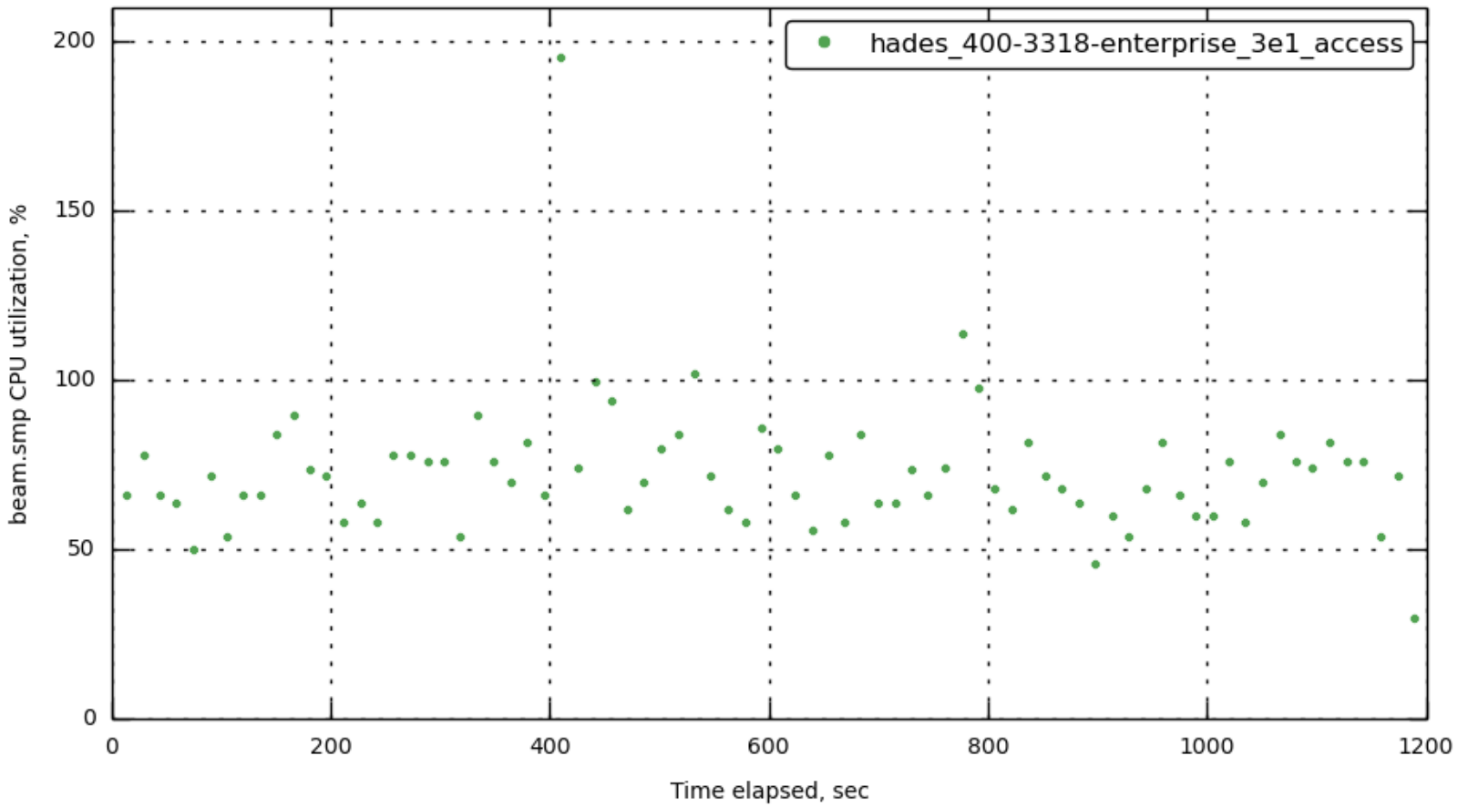
[172.23.100.73] beam.smp_cpu
