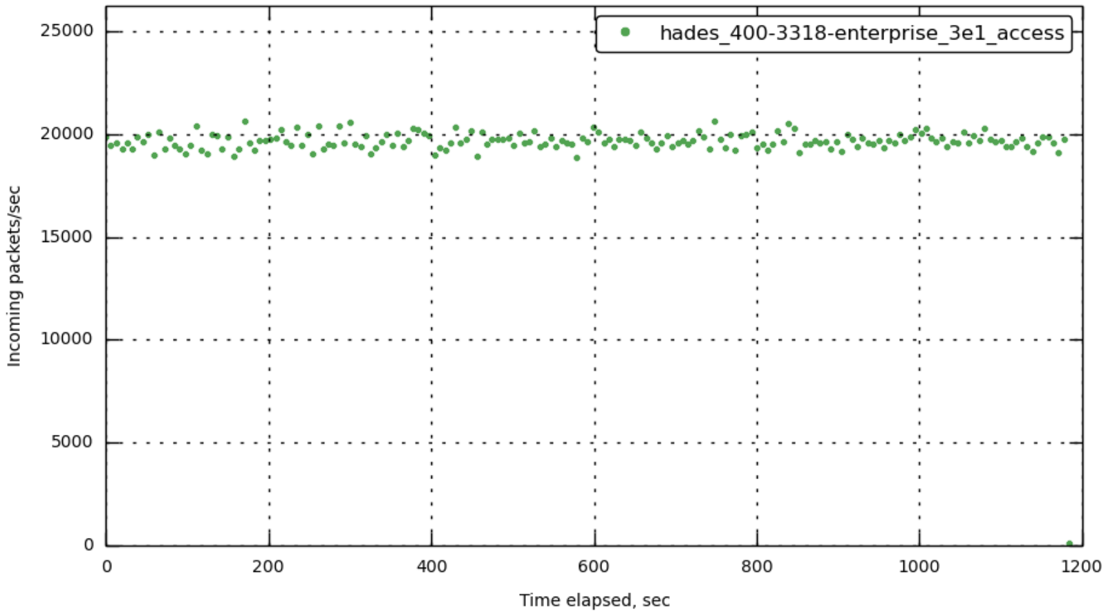
[172.23.100.72] in_packets_per_sec
