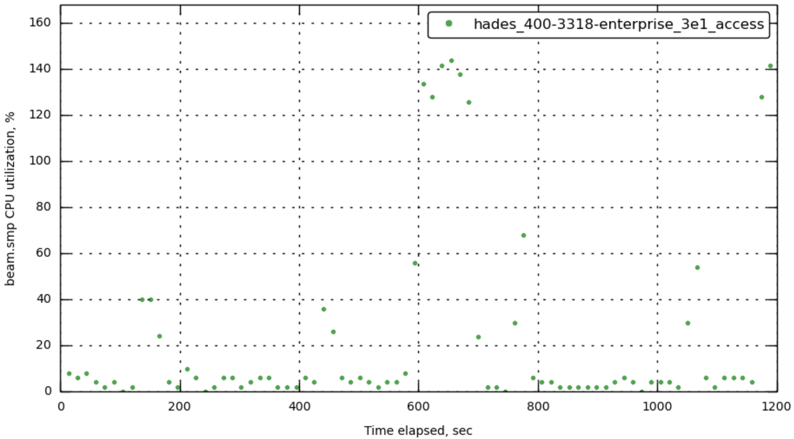
[172.23.100.45] beam.smp_cpu
