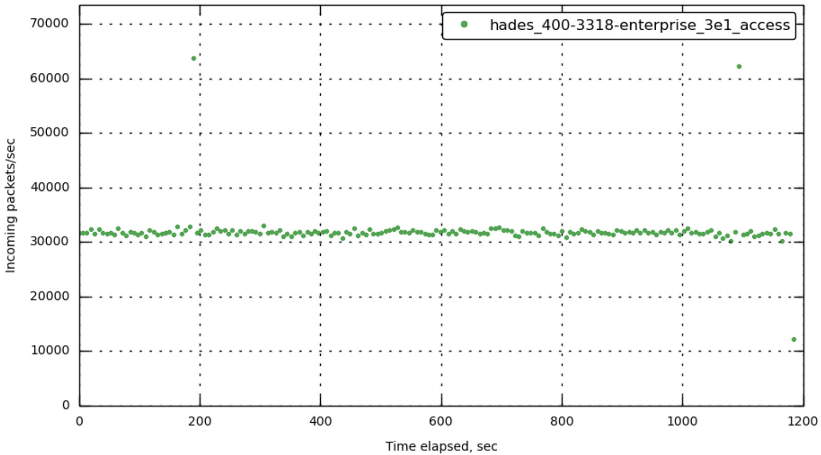
[172.23.100.71] in_packets_per_sec
