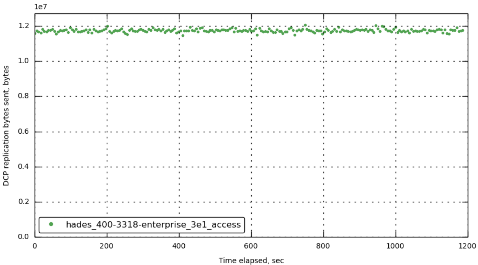
[bucket-1] ep_dcp_replica_total_bytes
