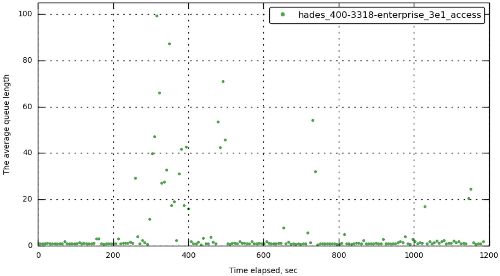
[172.23.100.72] data_avgqusz
