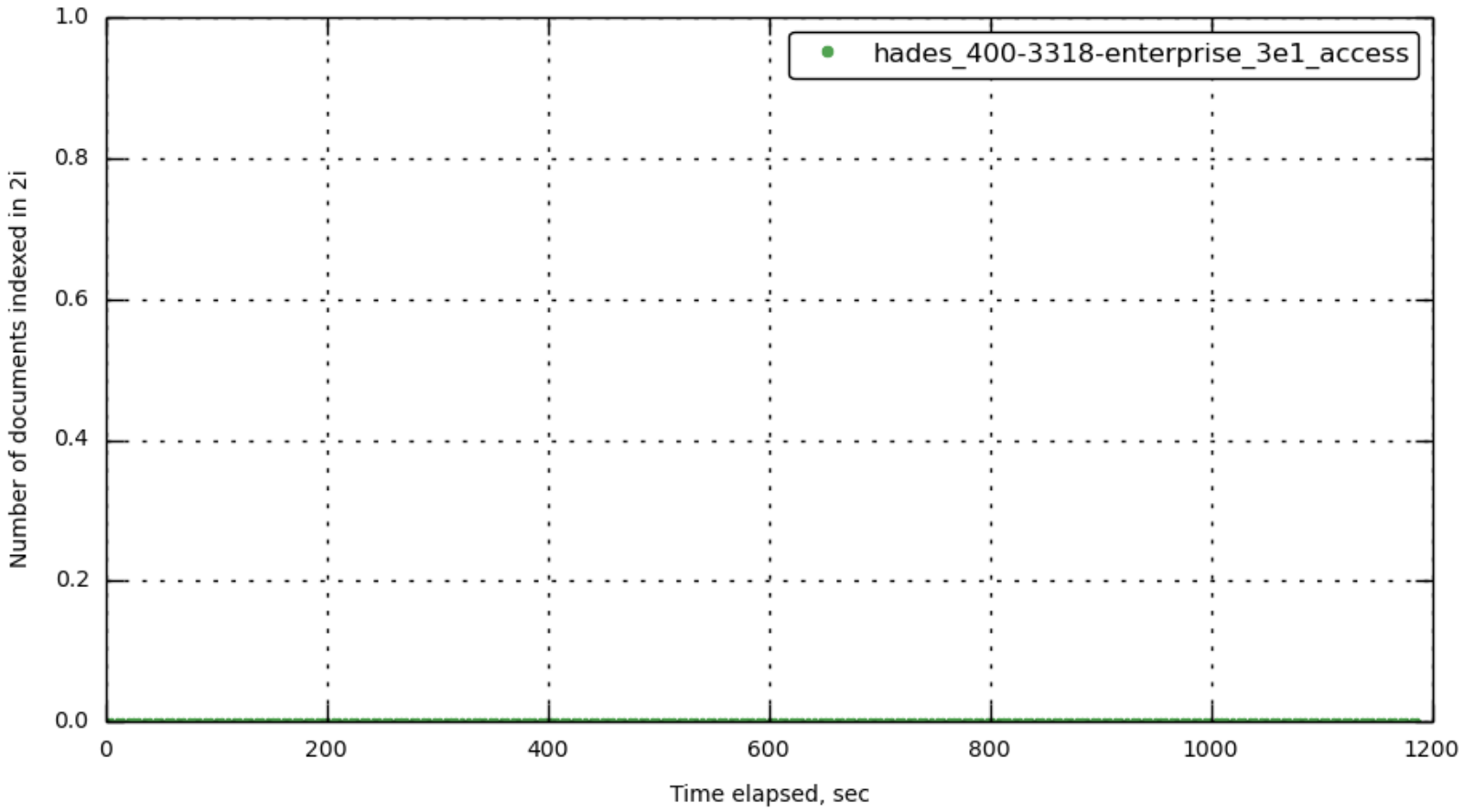
[bucket-1] index_num_docs_indexed
