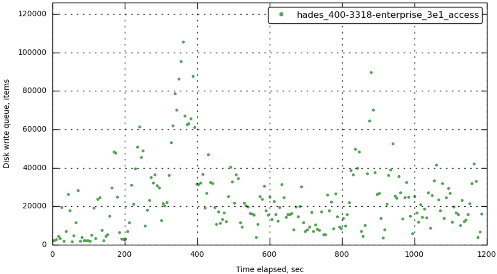
[bucket-1] disk_write_queue
