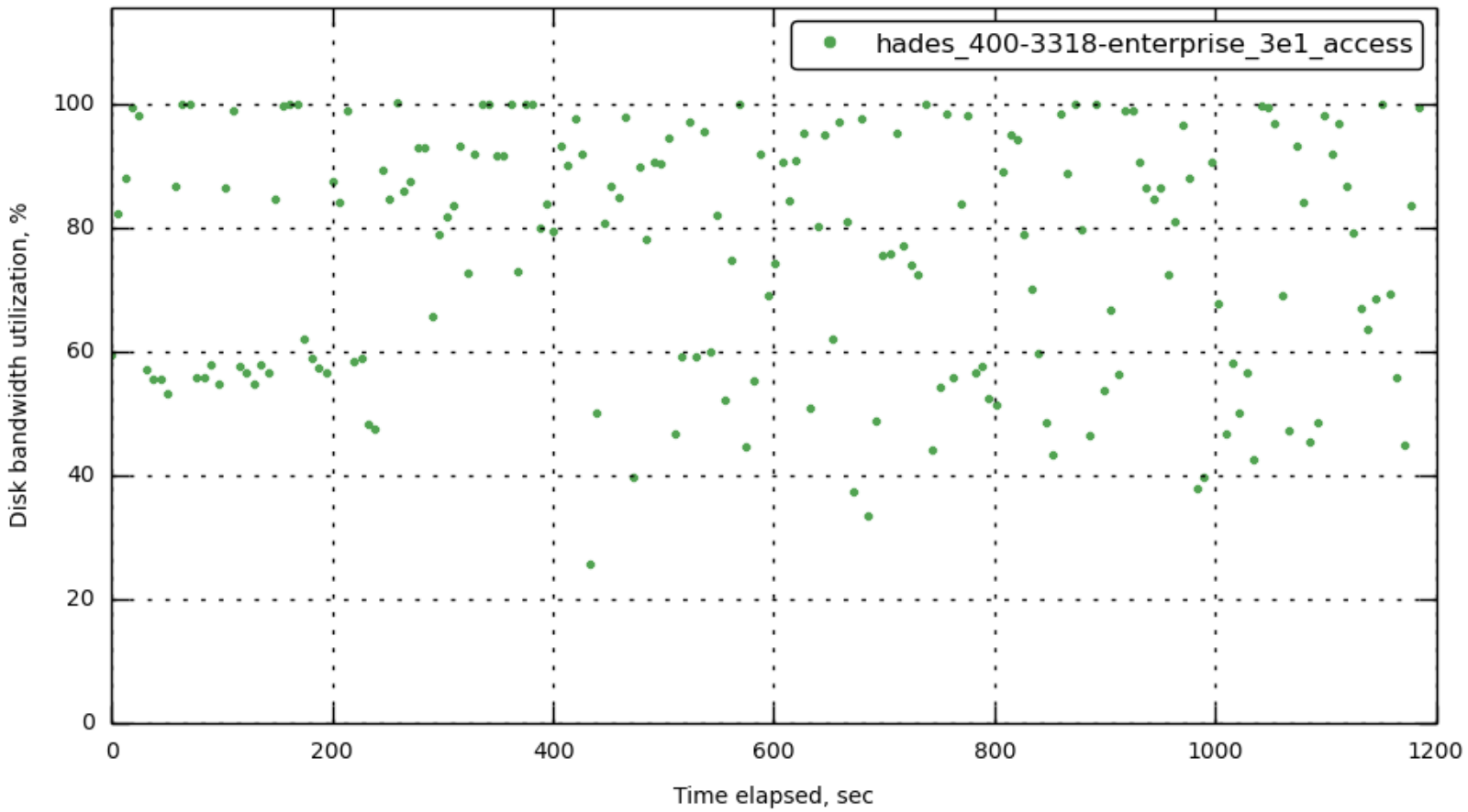
[172.23.100.72] data_util
