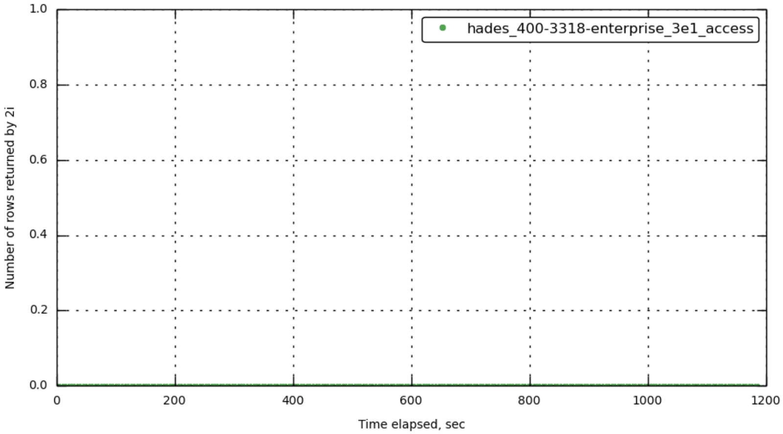
[bucket-1] index_num_rows_returned
