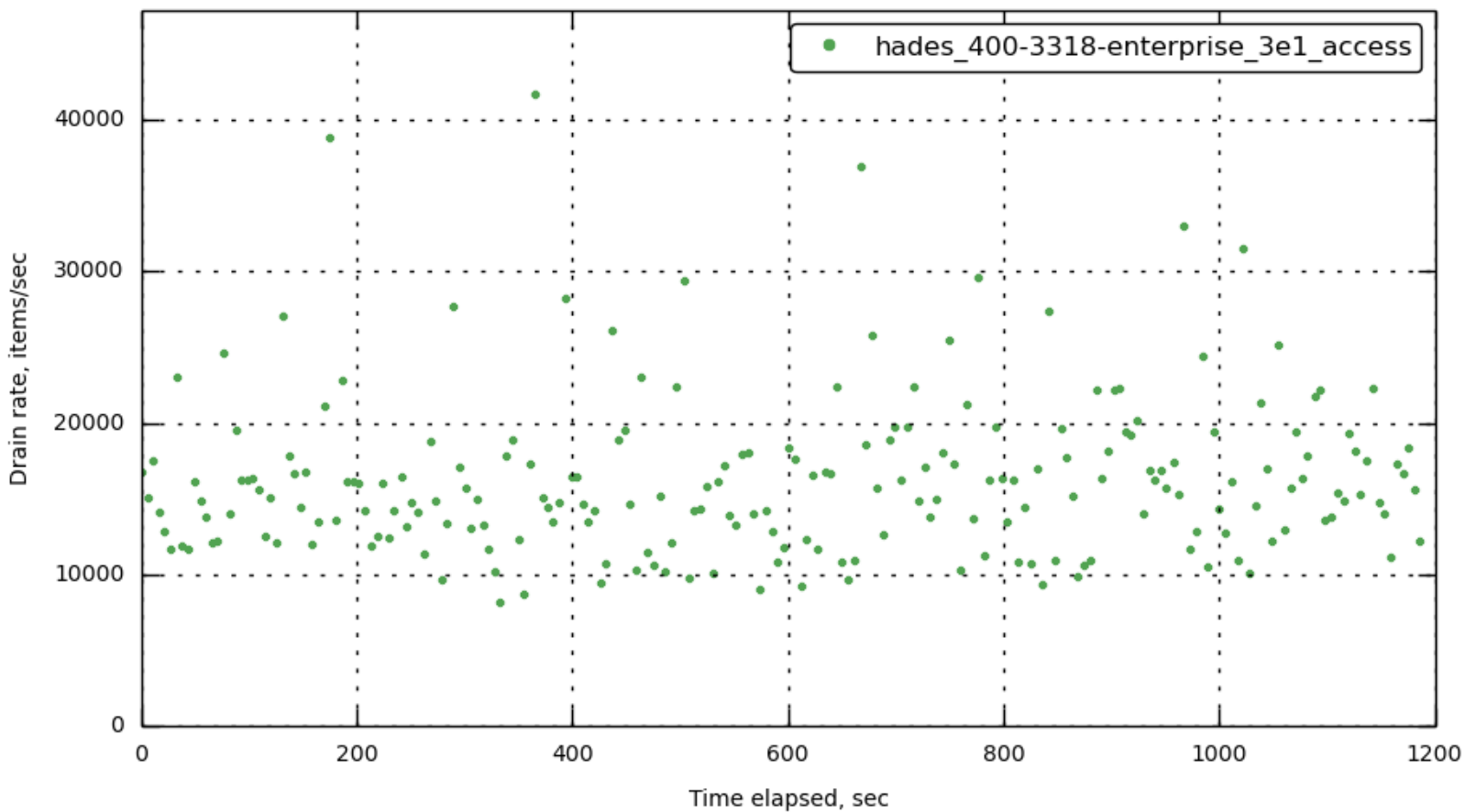
[bucket-1] ep_diskqueue_drain
