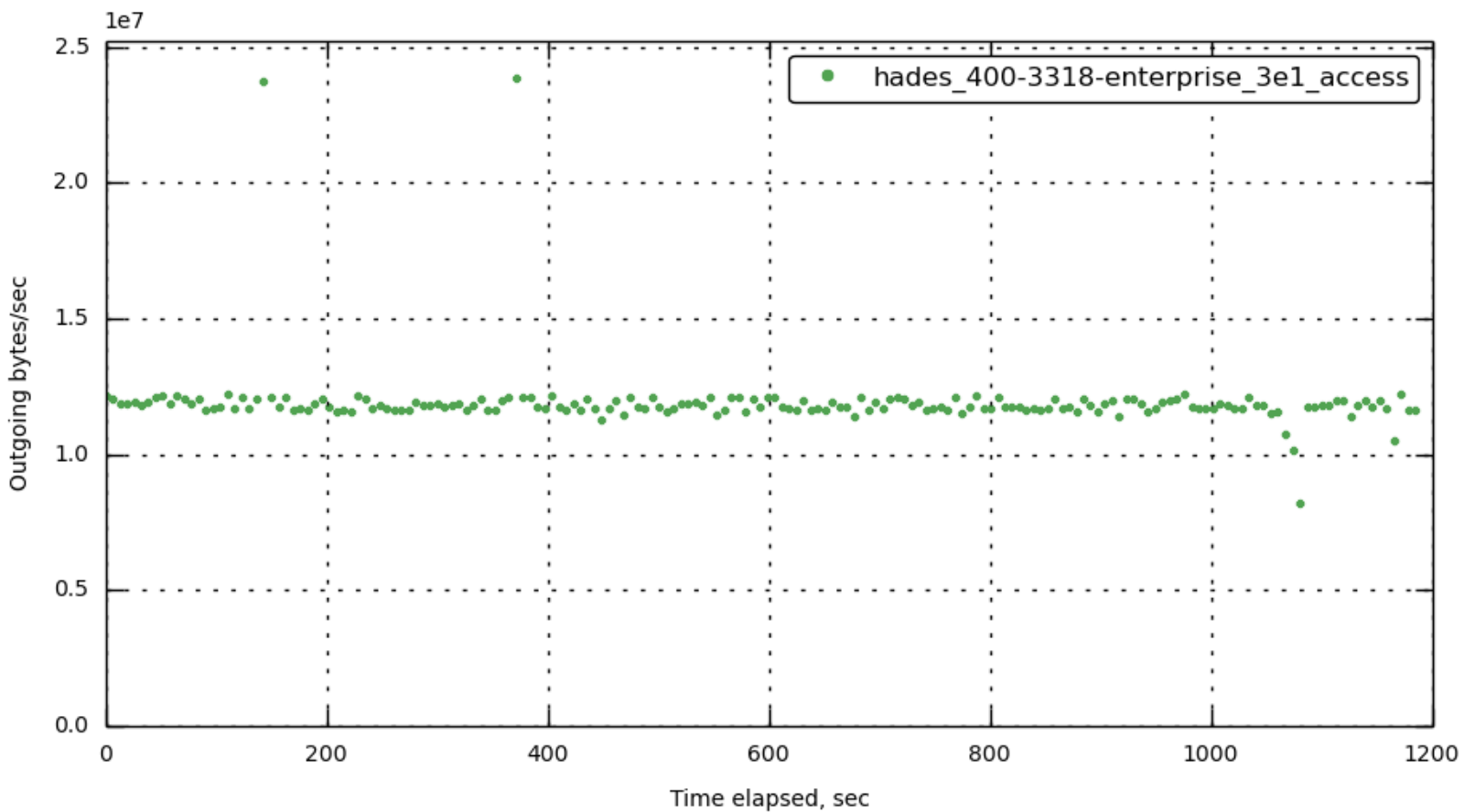
[172.23.100.55] out_bytes_per_sec
