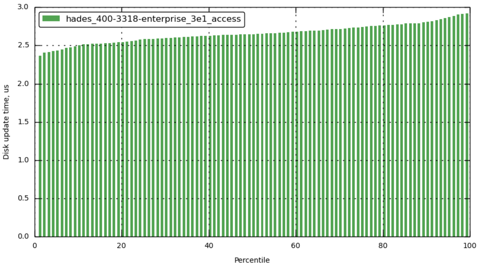
[bucket-1] avg_disk_update_time
