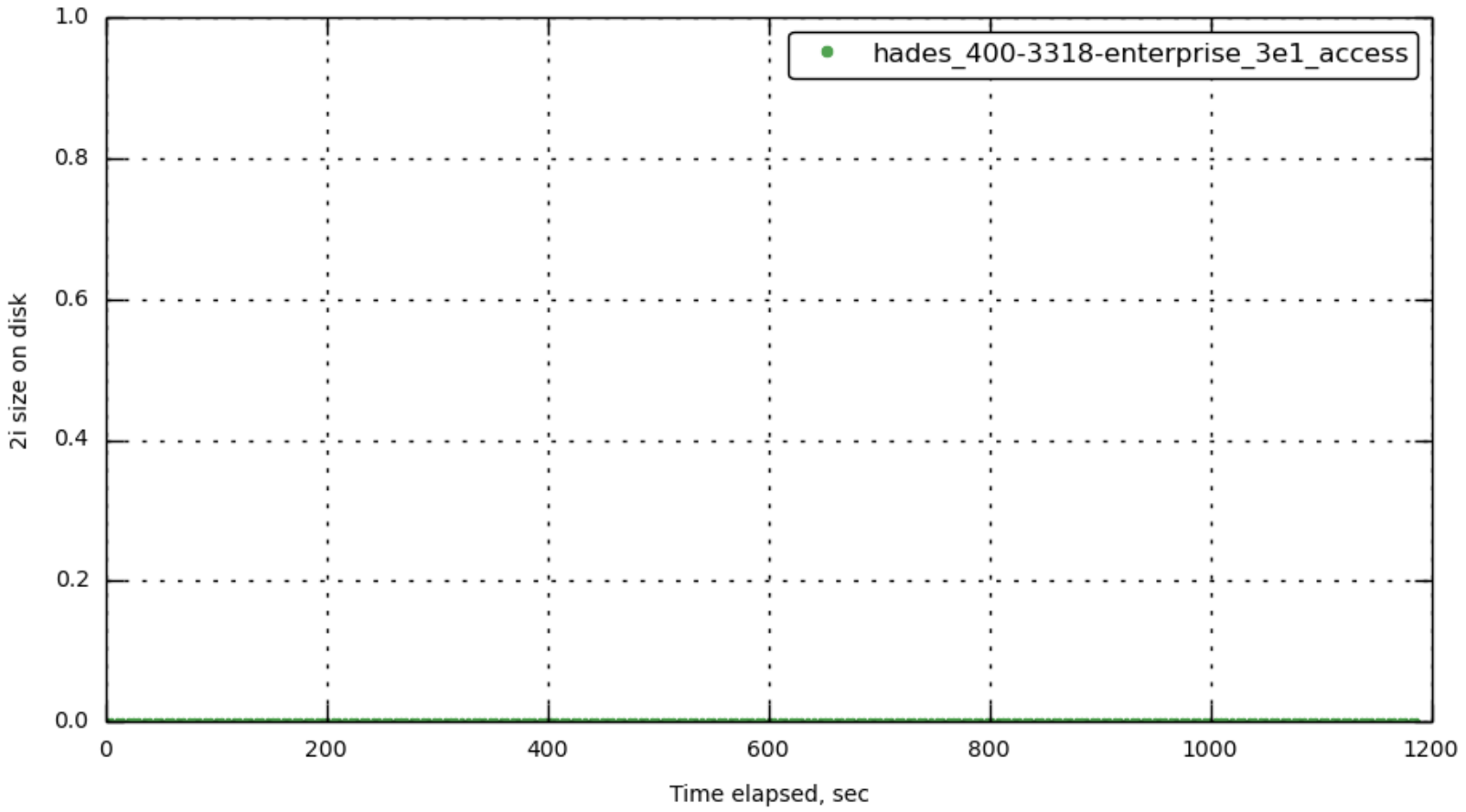
[bucket-1] index_disk_size
