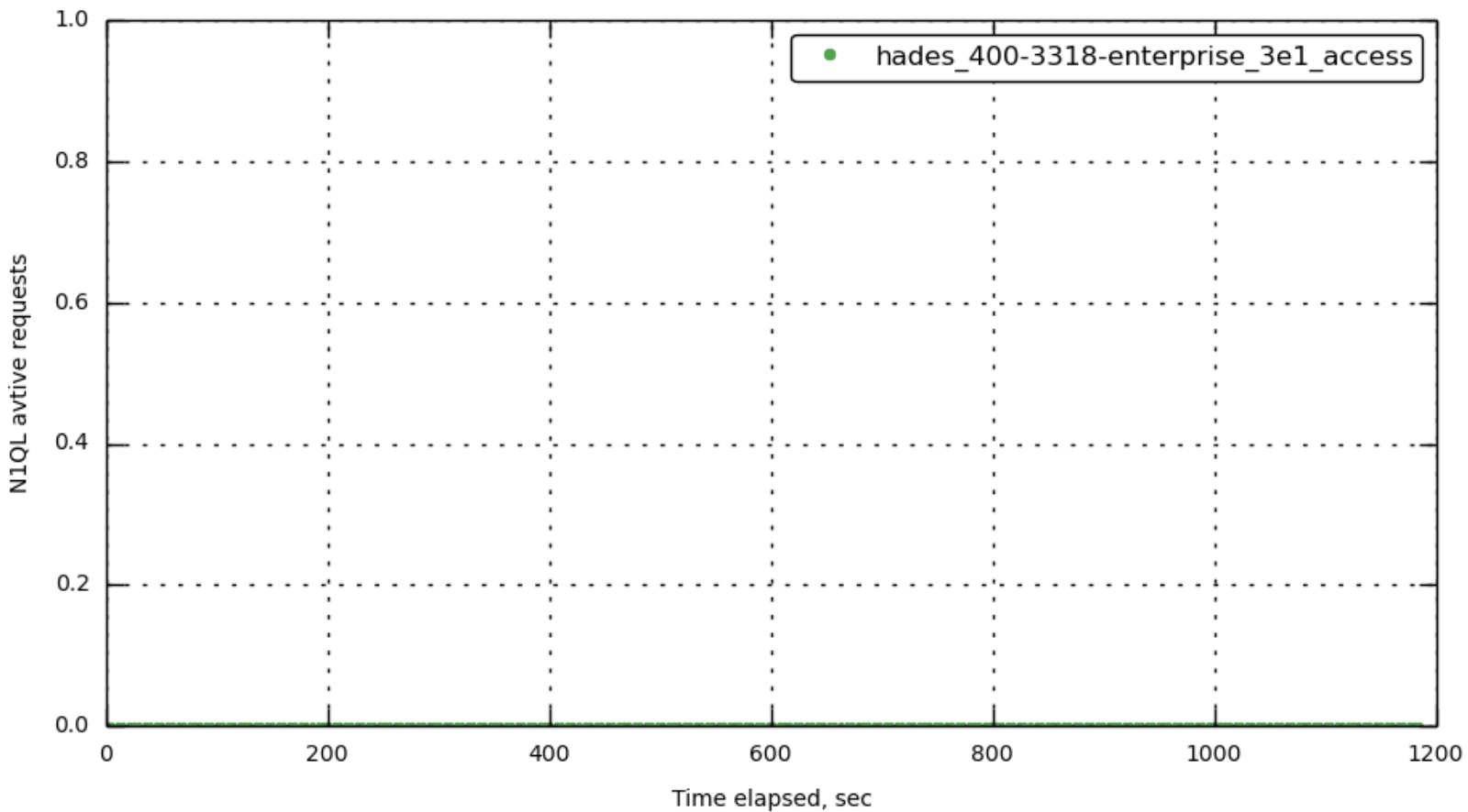
query_active_requests
