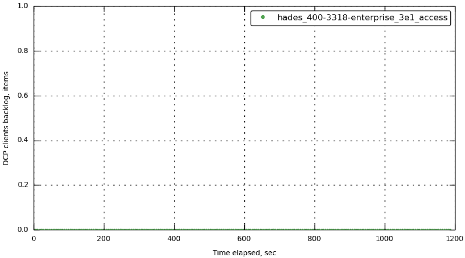
[bucket-1] ep_dcp_other_items_remaining
