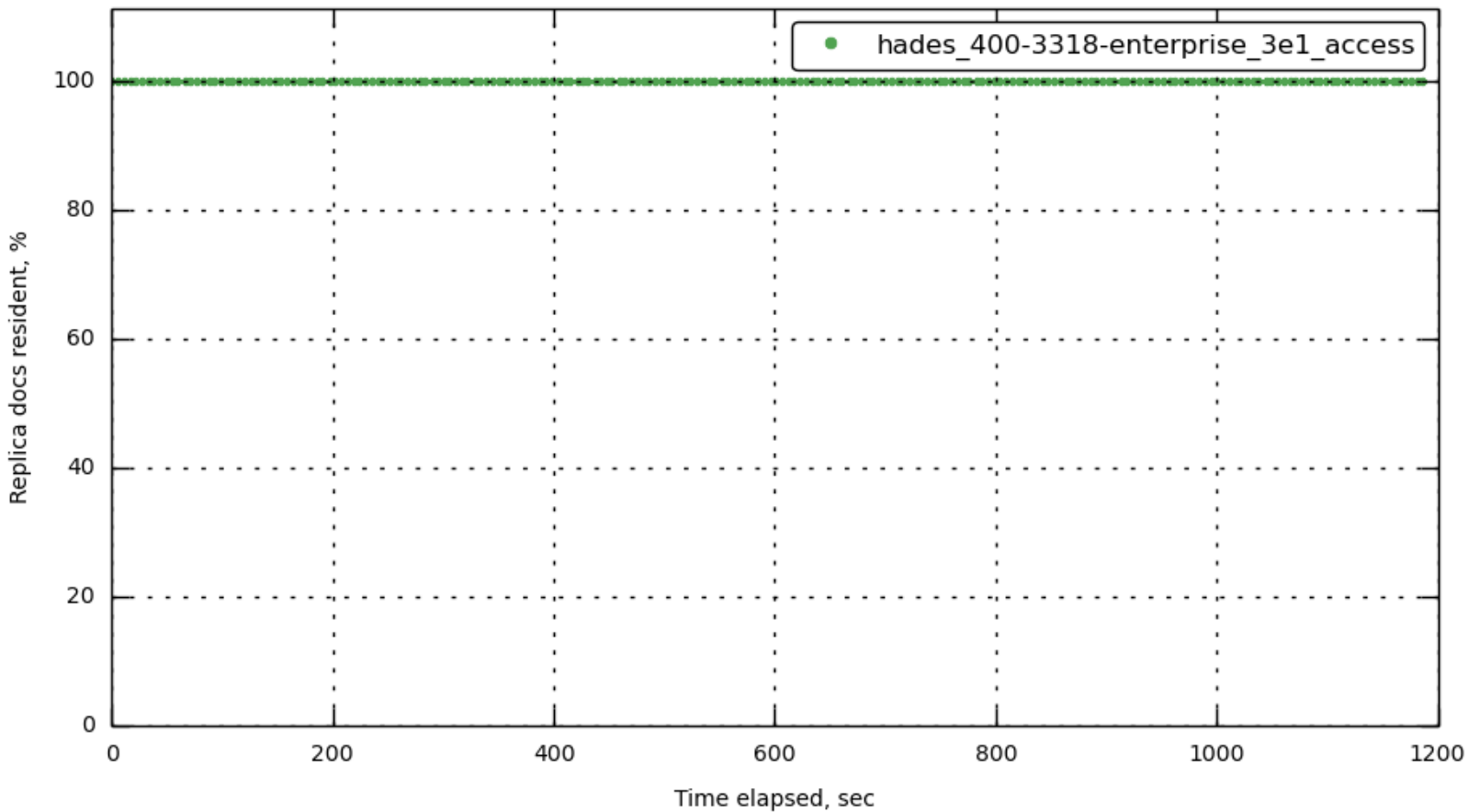
[bucket-1] vb_replica_resident_items_ratio
