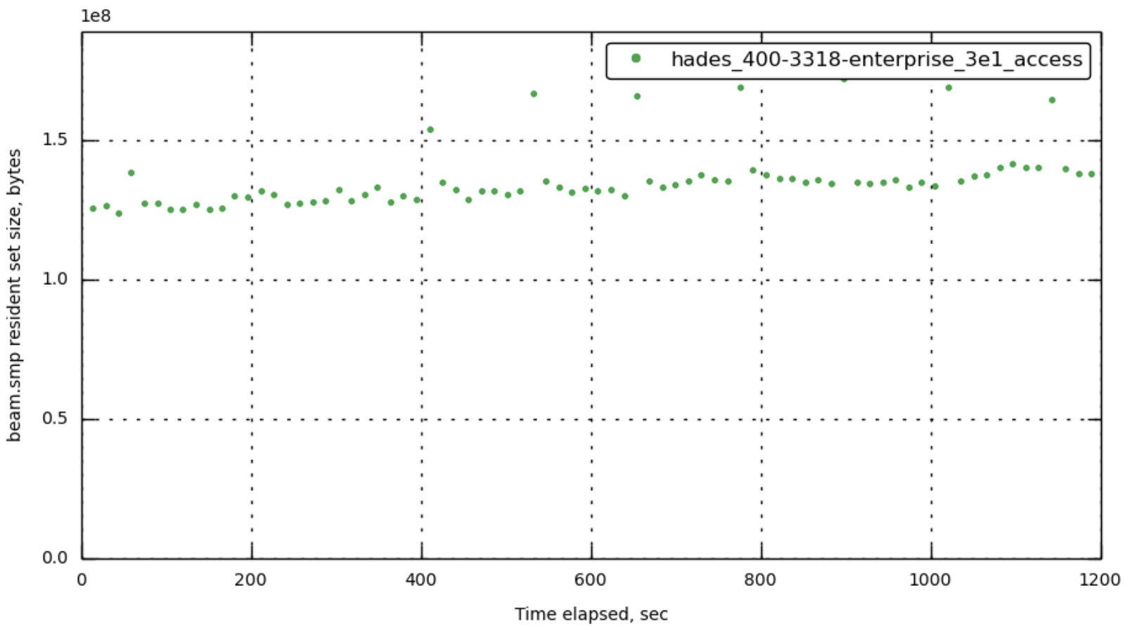
[172.23.100.45] beam.smp_rss
