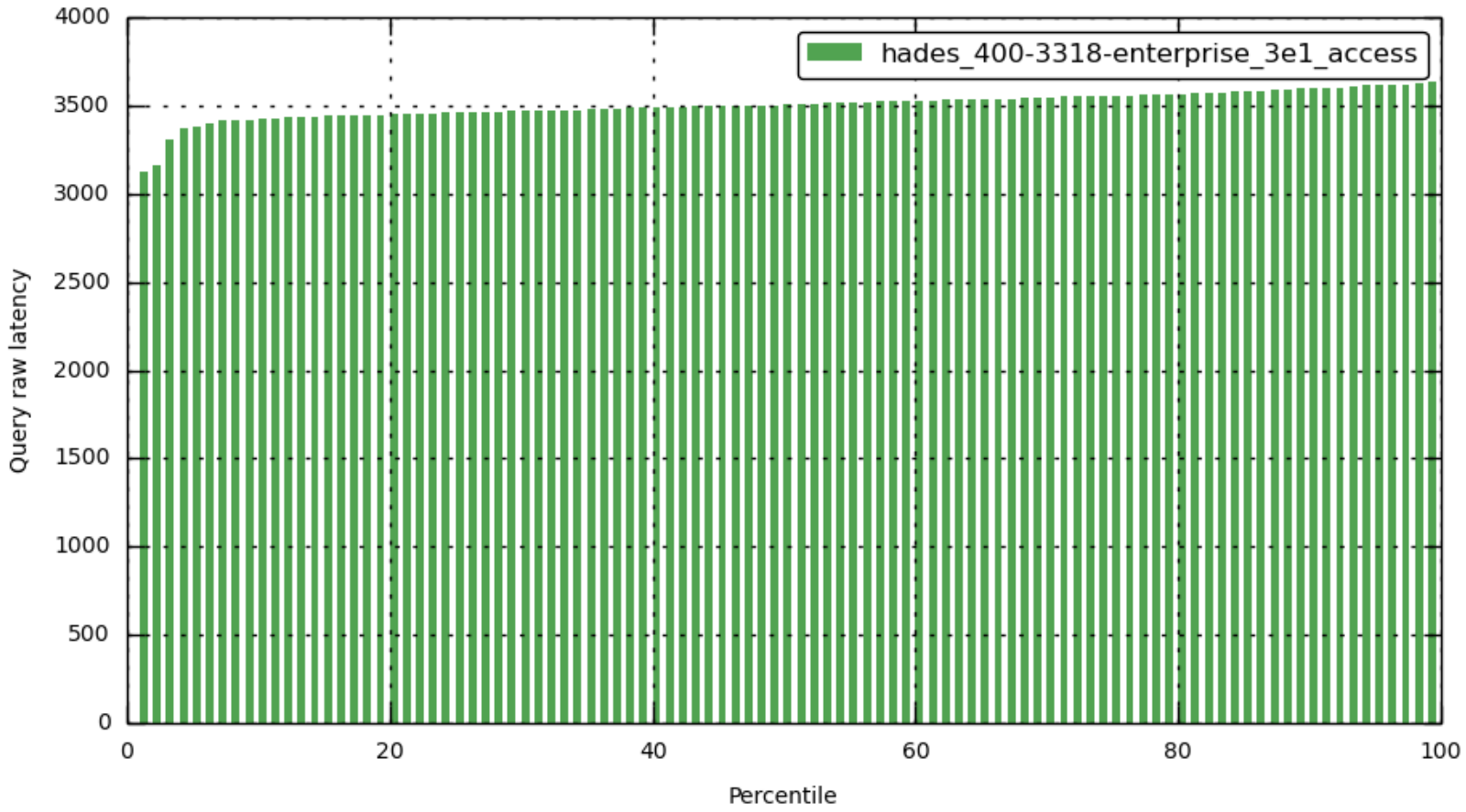
query_requests
