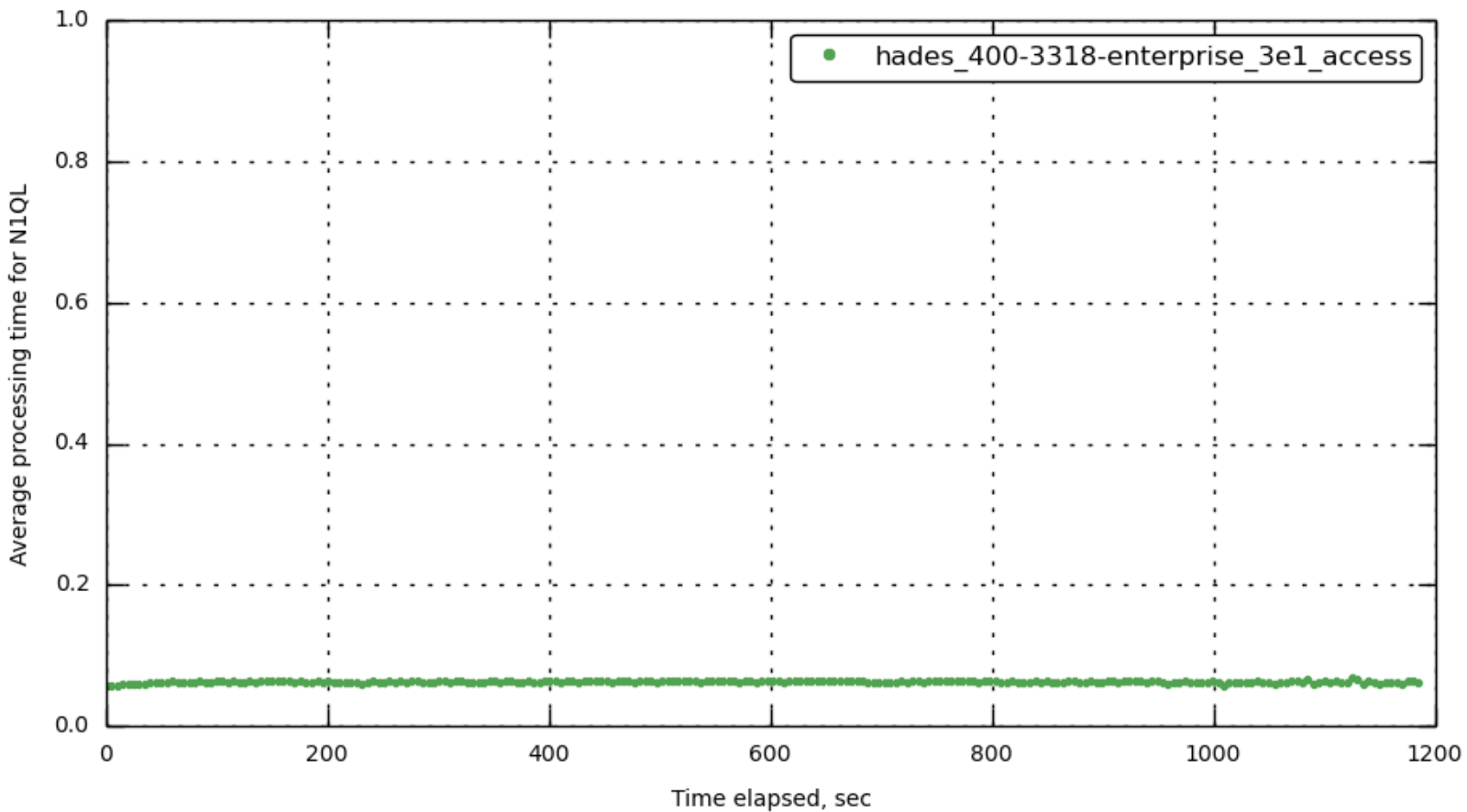
query_avg_req_time
