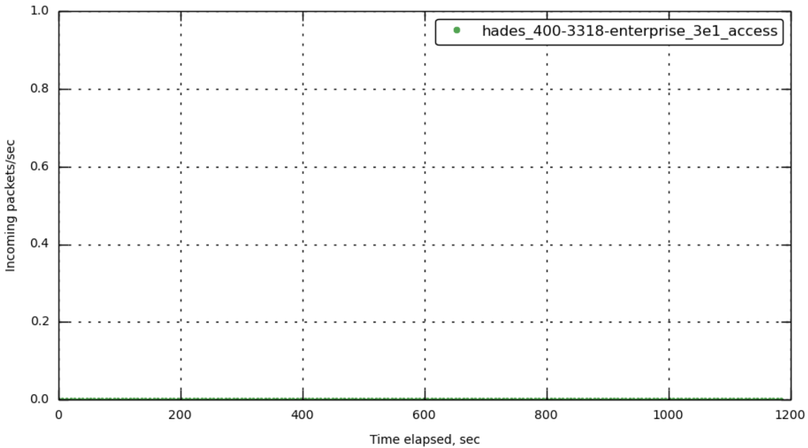
[172.23.100.73] in_packets_per_sec
