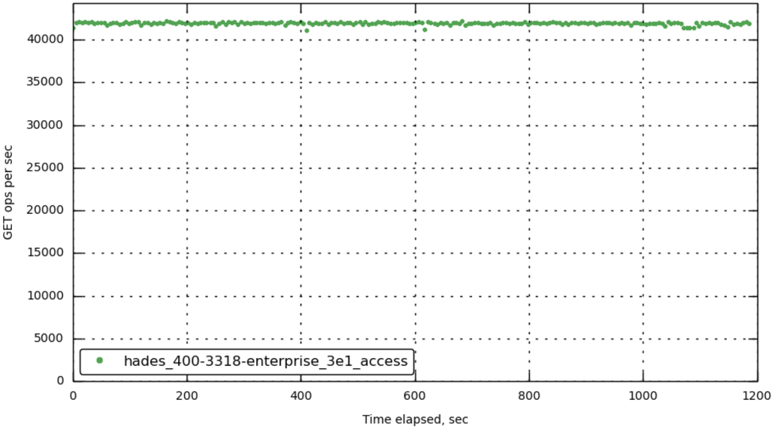
[bucket-1] cmd_get
