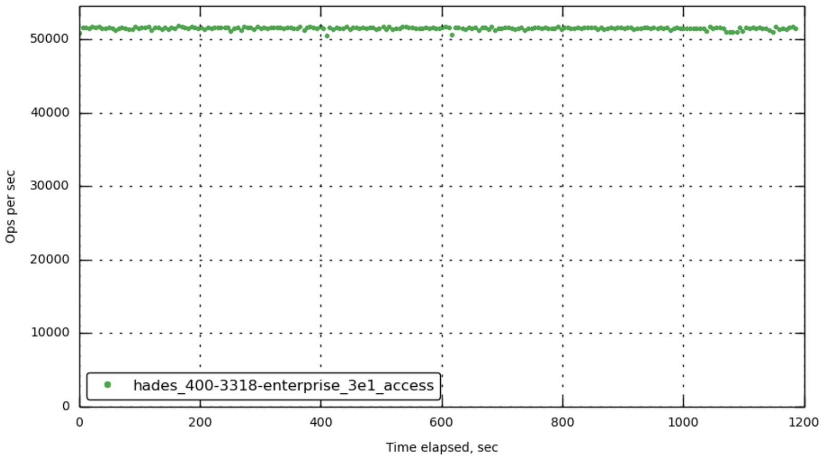
[bucket-1] ops
