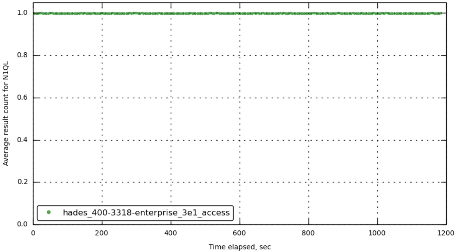
query_avg_result_count
