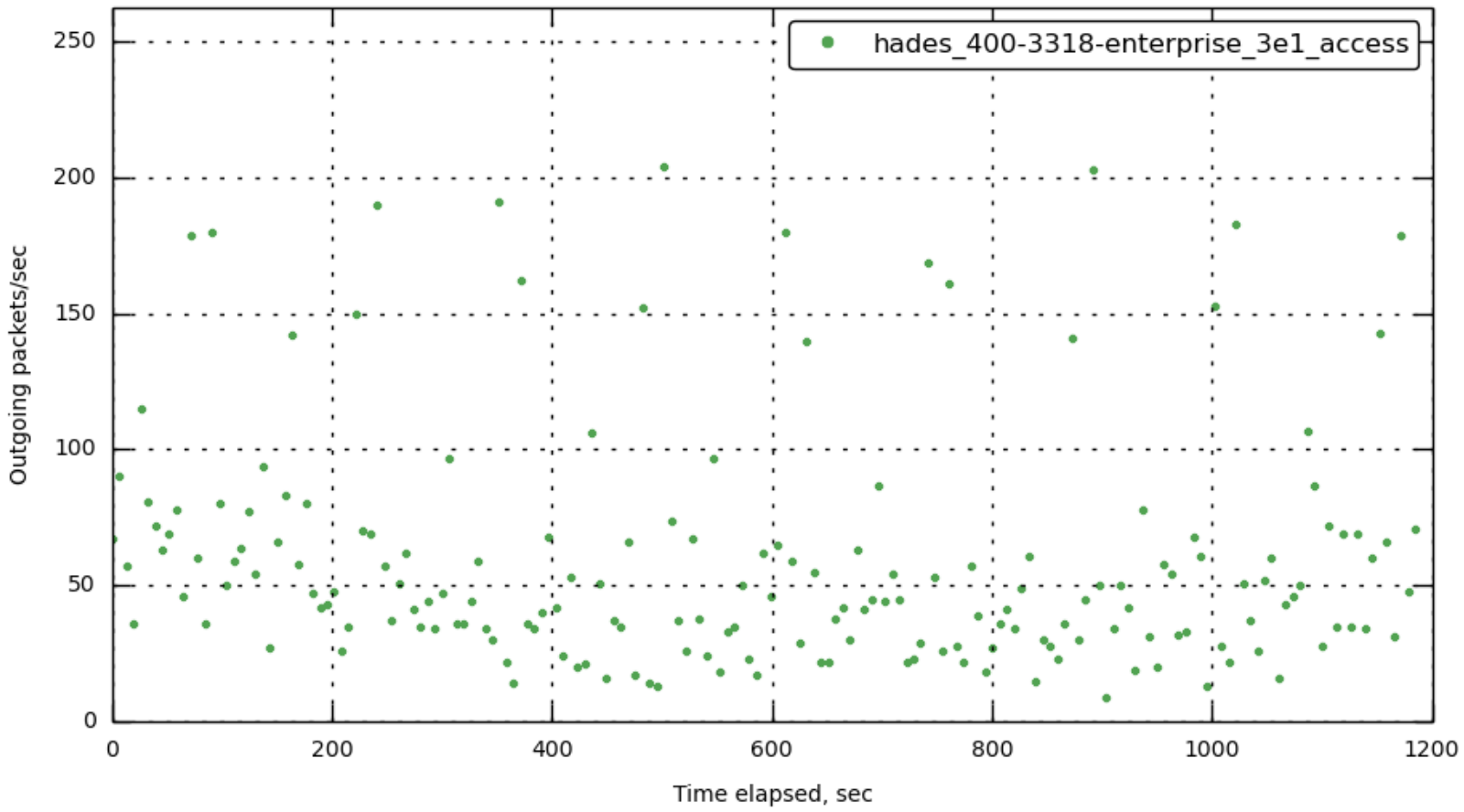
[172.23.100.45] out_packets_per_sec
