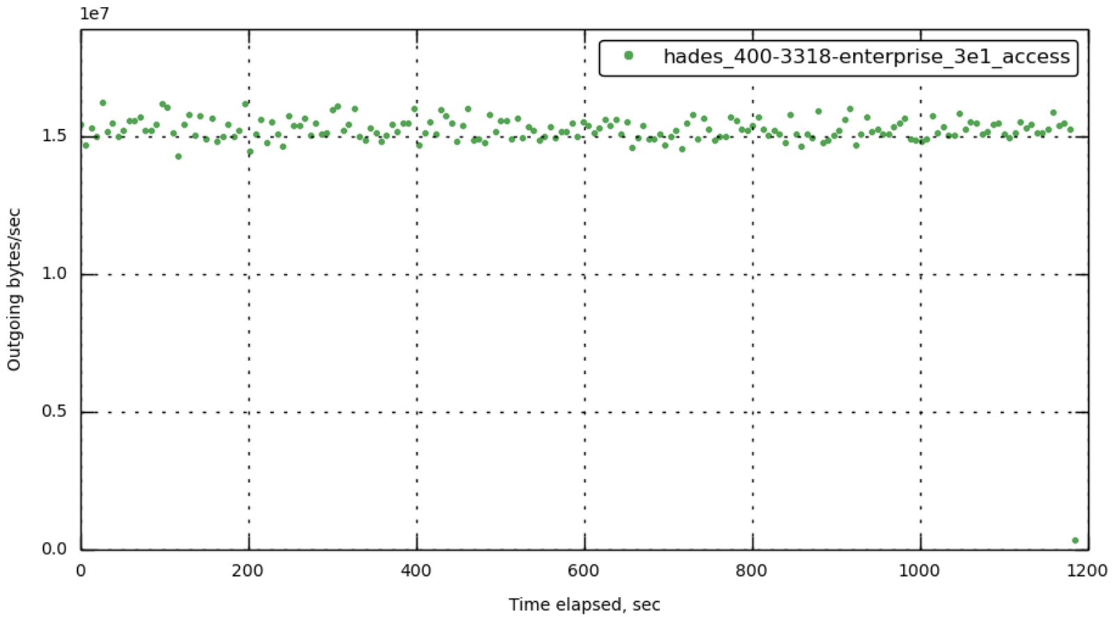
[172.23.100.70] out_bytes_per_sec
