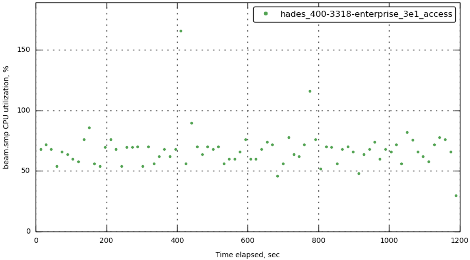
[172.23.100.71] beam.smp_cpu
