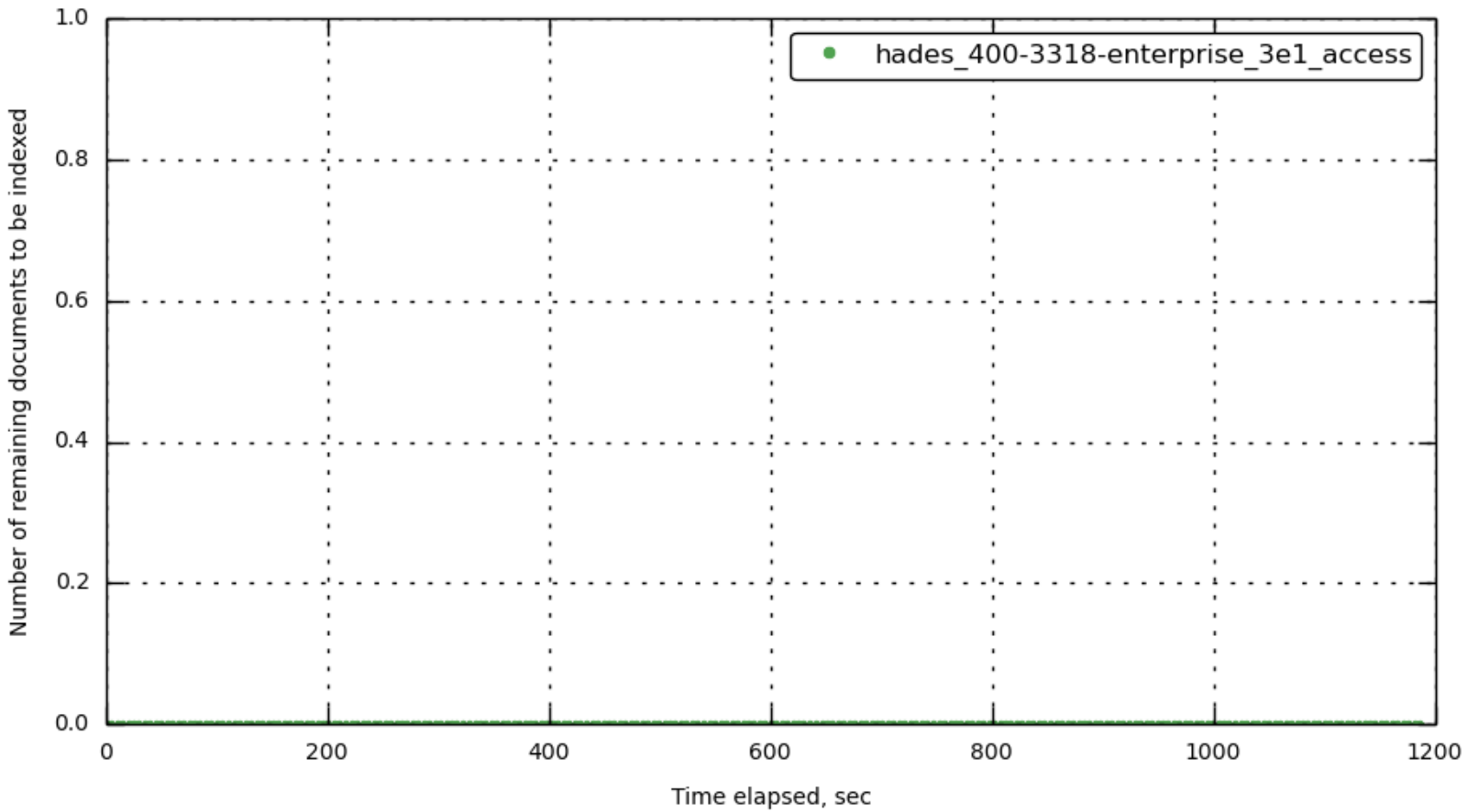
[bucket-1] index_num_docs_pending
