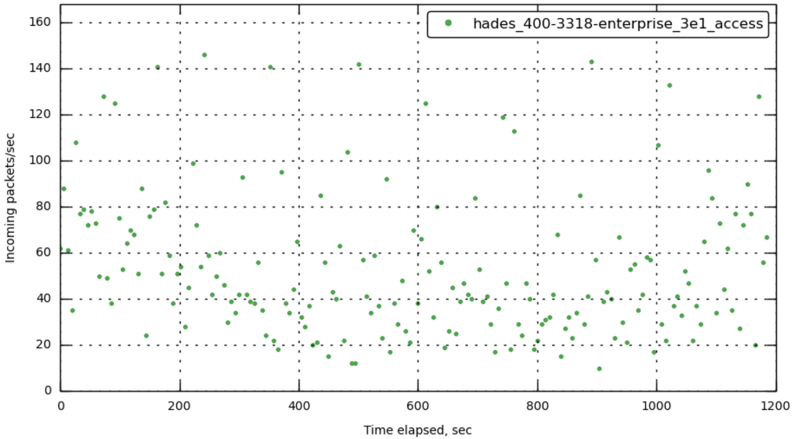
[172.23.100.45] in_packets_per_sec
