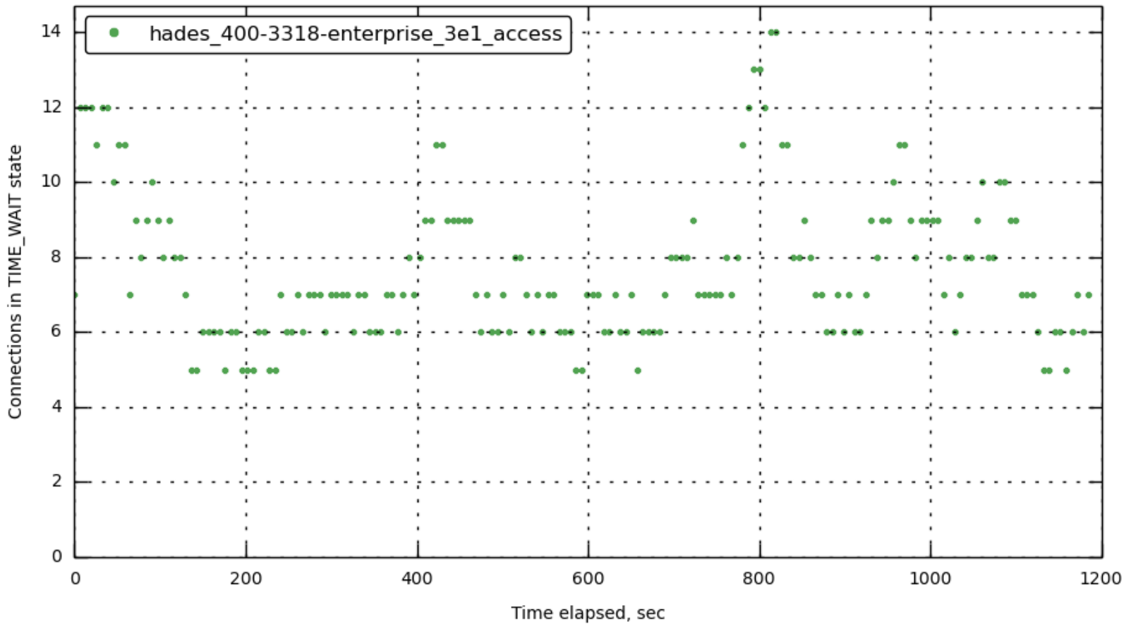
[172.23.100.72] TIME_WAIT
