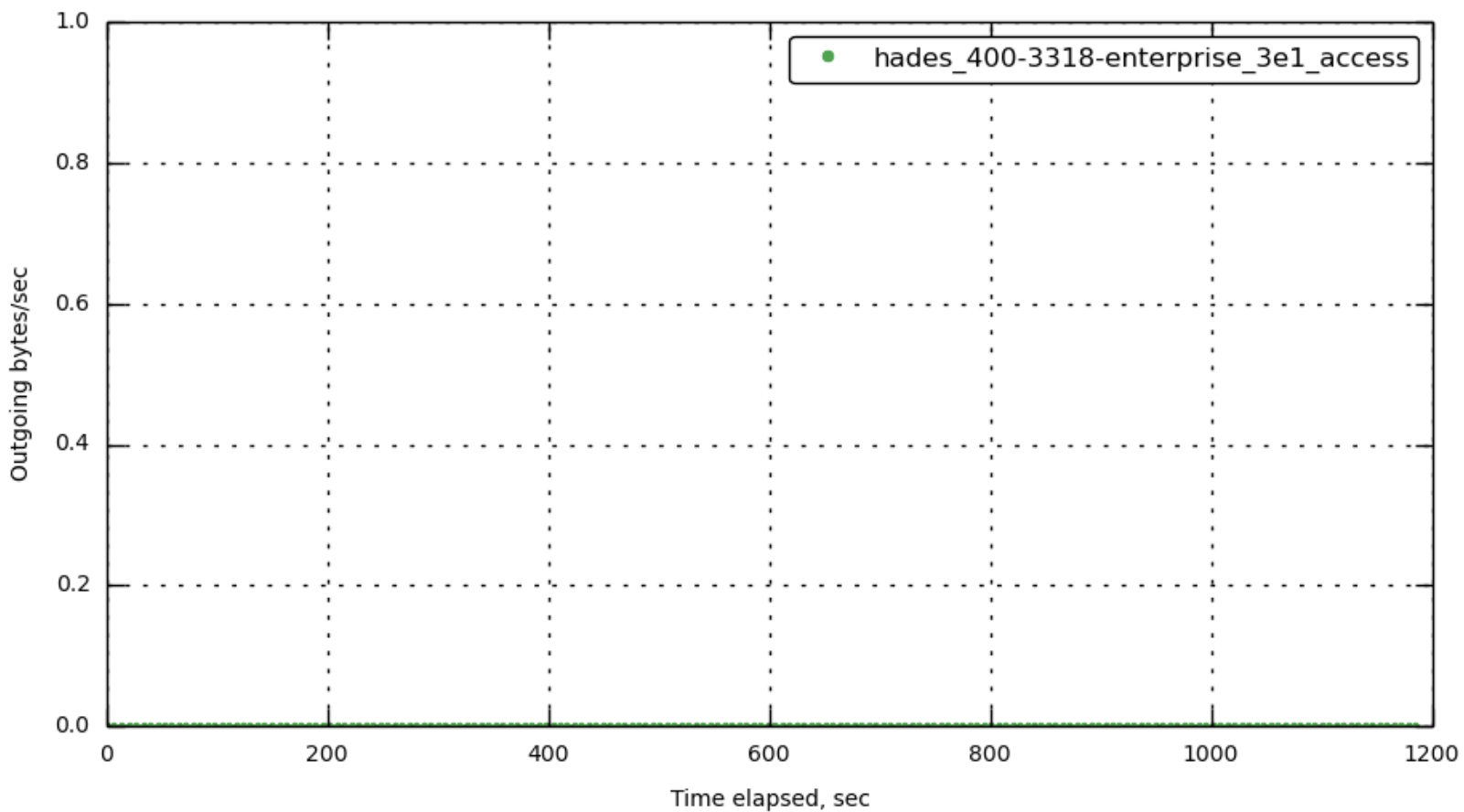
[172.23.100.73] out_bytes_per_sec
