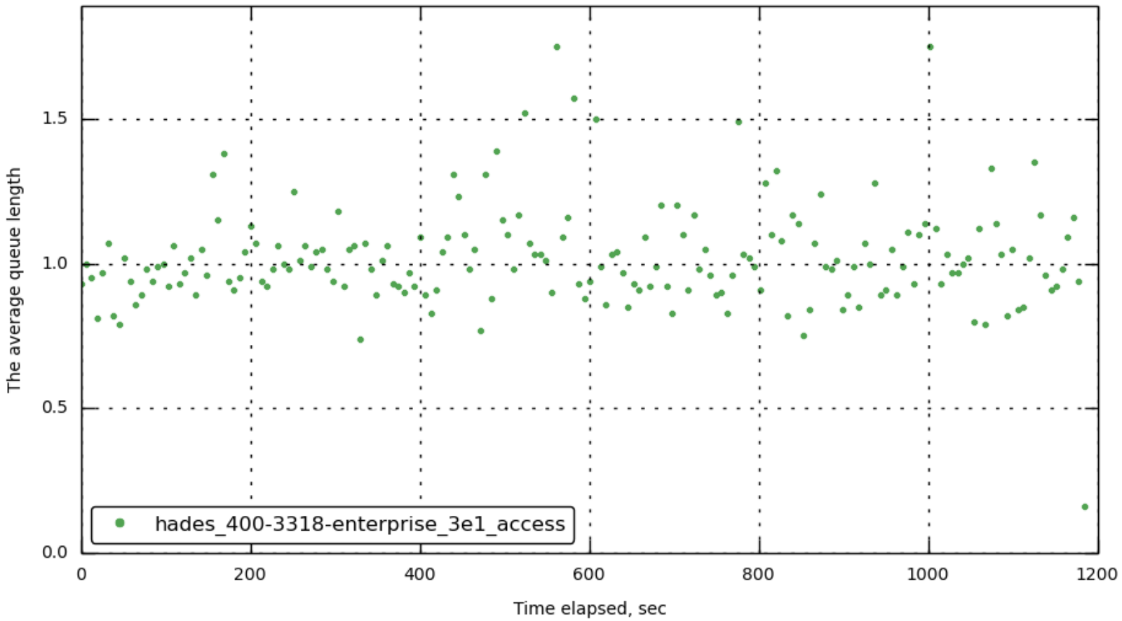
[172.23.100.70] data_avgqusz
