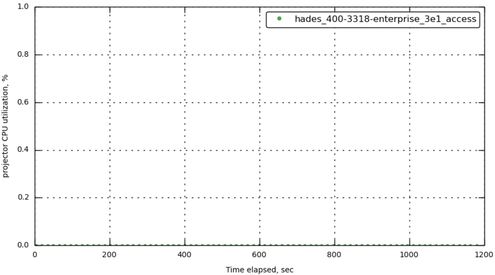
[172.23.100.72] projector_cpu
