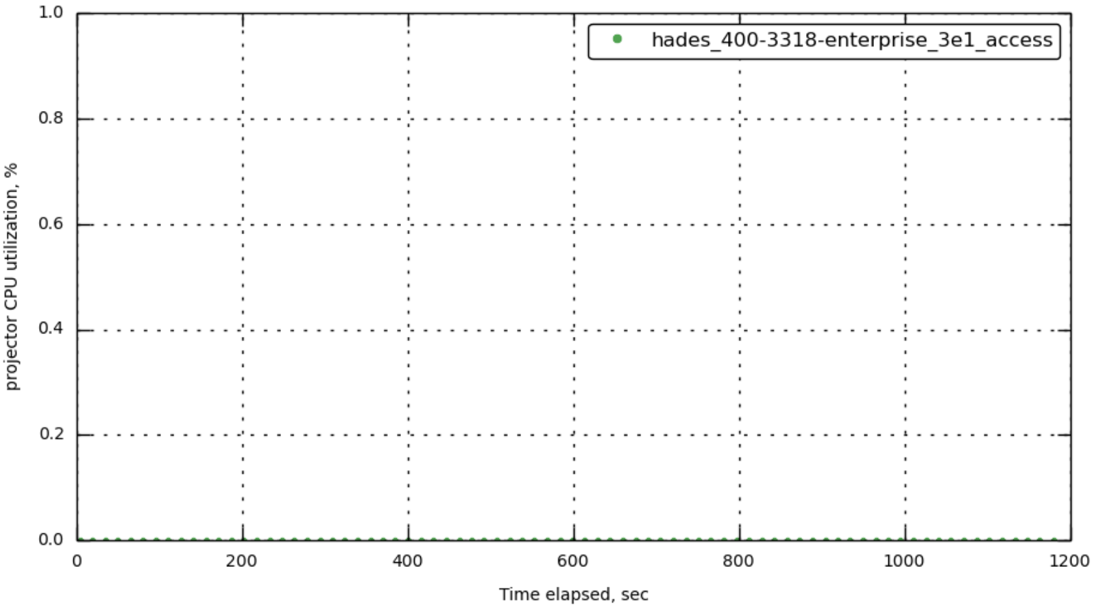
[172.23.100.71] projector_cpu
