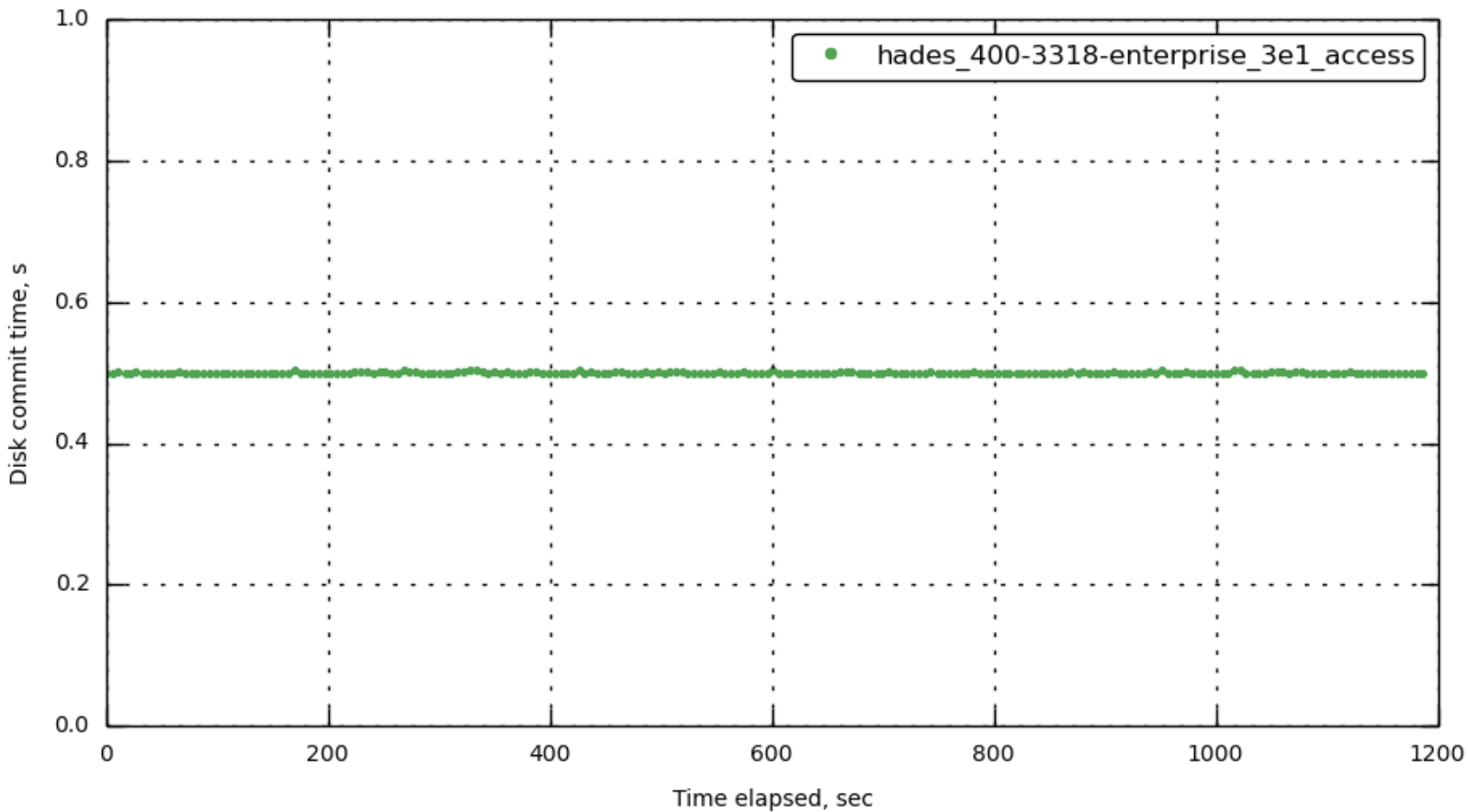
[bucket-1] avg_disk_commit_time
