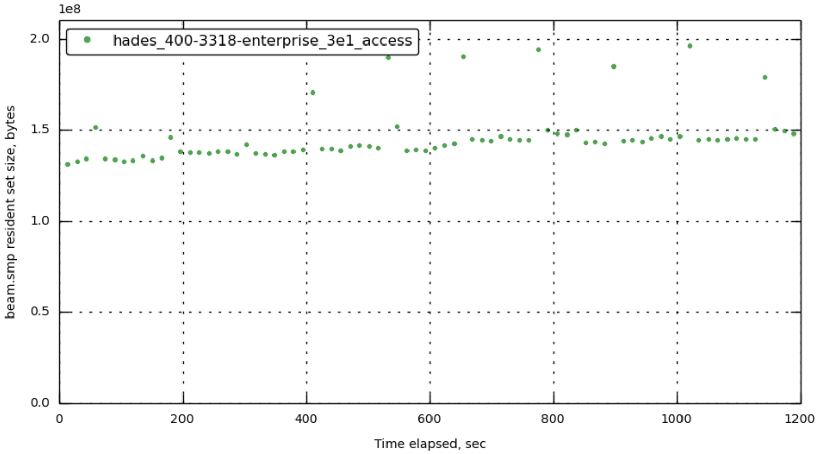
[172.23.100.71] beam.smp_rss
