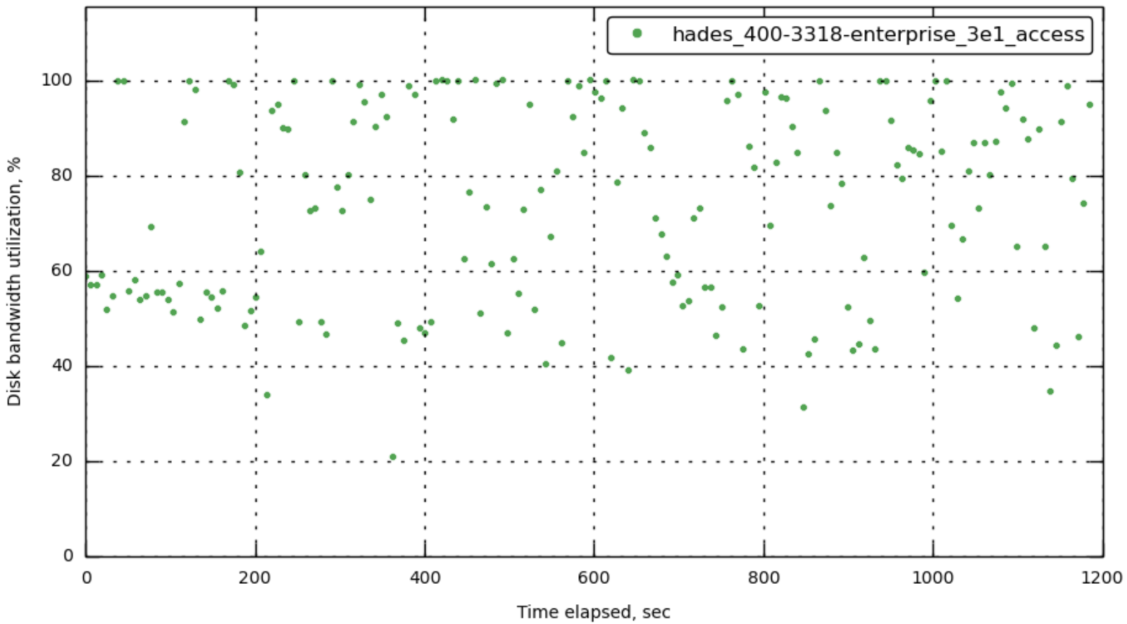
[172.23.100.71] data_util
