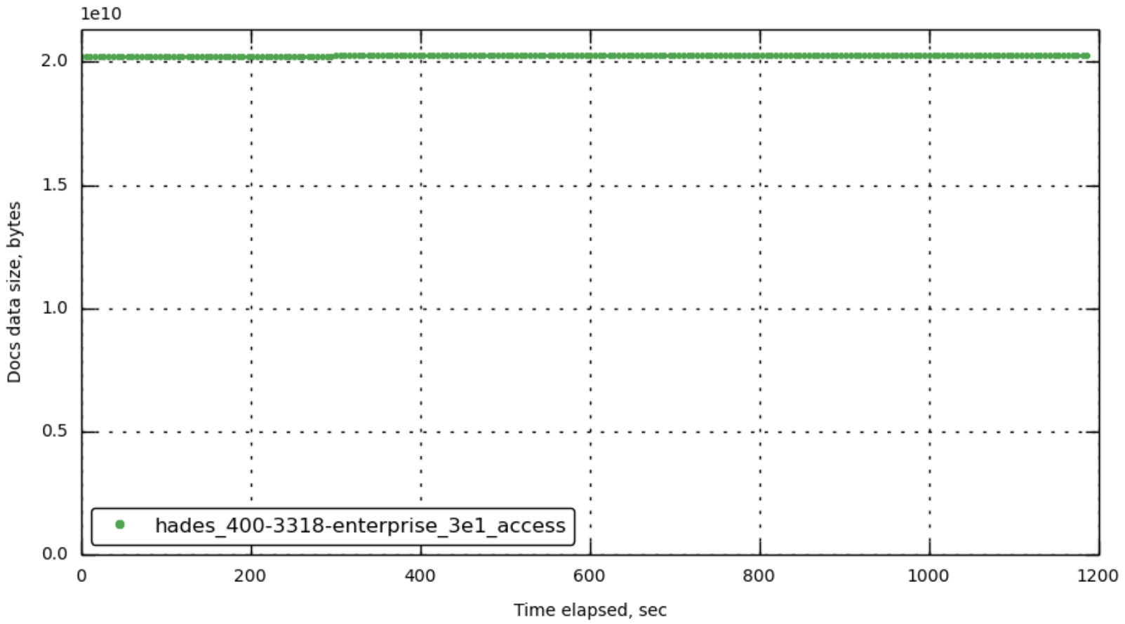
[bucket-1] couch_docs_data_size
