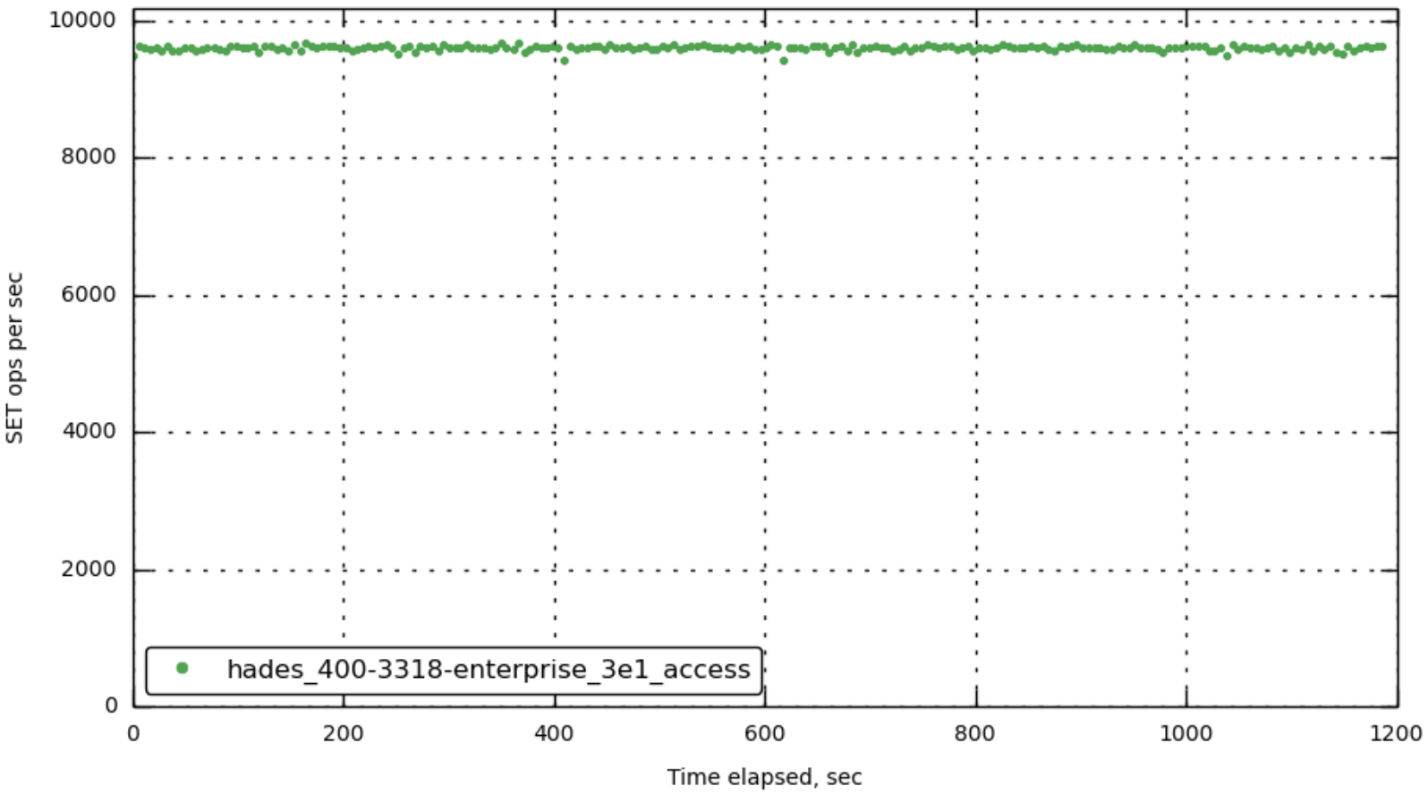
[bucket-1] cmd_set
