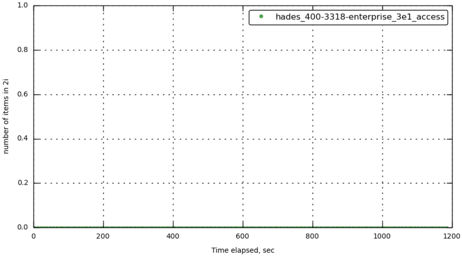
[bucket-1] index_items_count
