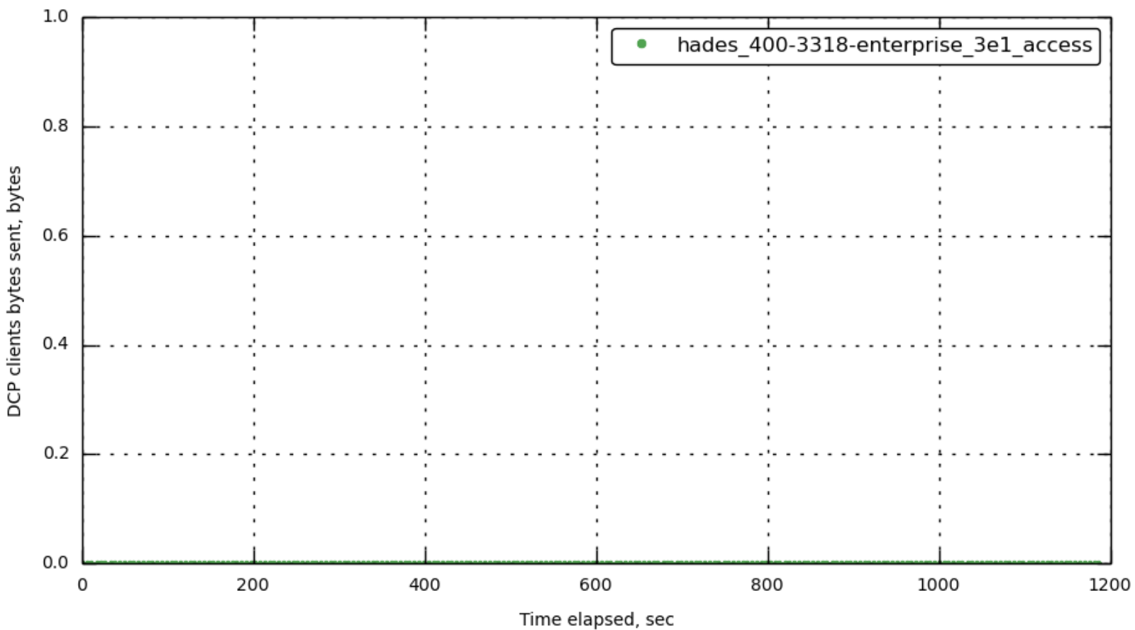
[bucket-1] ep_dcp_other_total_bytes
