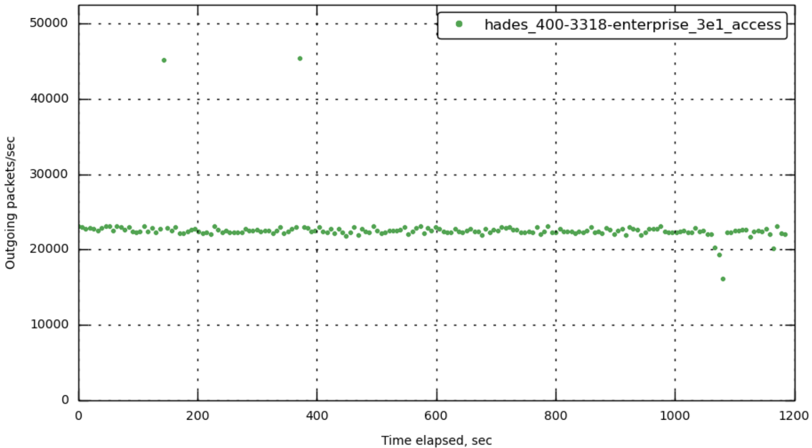
[172.23.100.55] out_packets_per_sec
