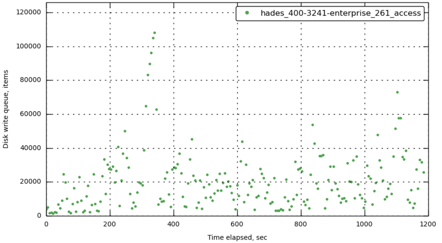
[bucket-1] disk_write_queue
