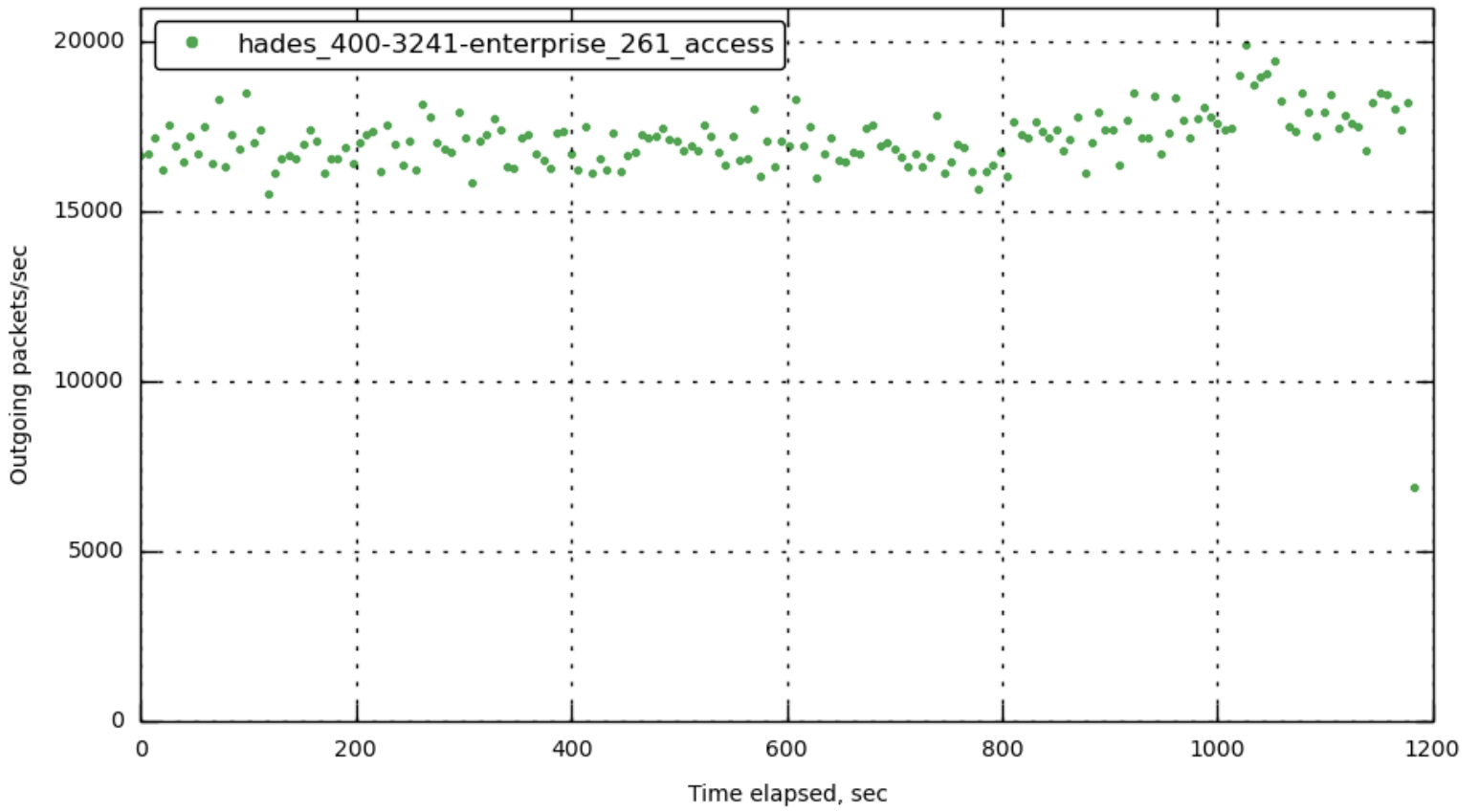
[172.23.100.71] out_packets_per_sec
