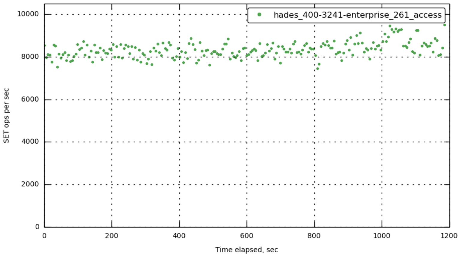
[bucket-1] cmd_set
