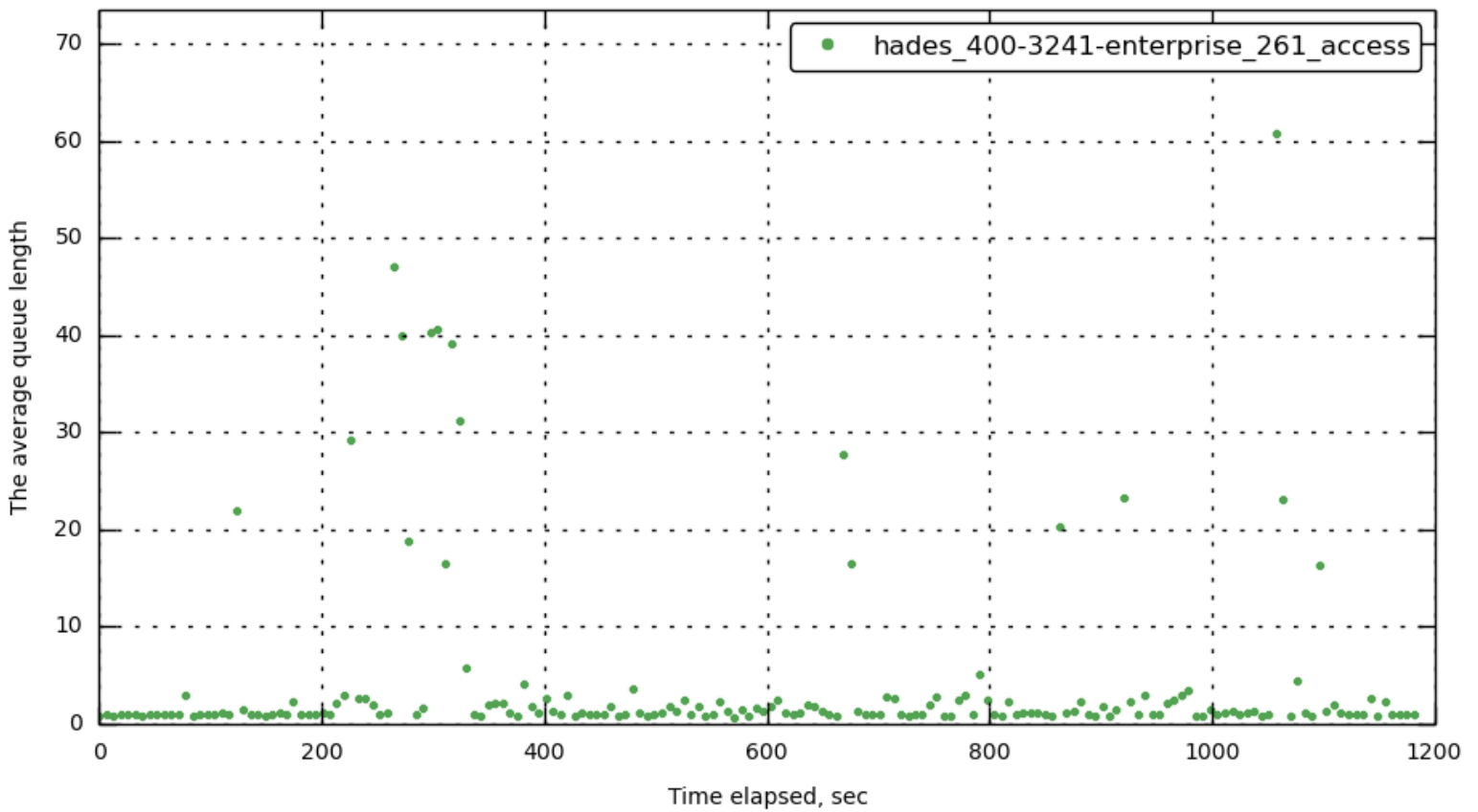
[172.23.100.72] data_avgqsz
