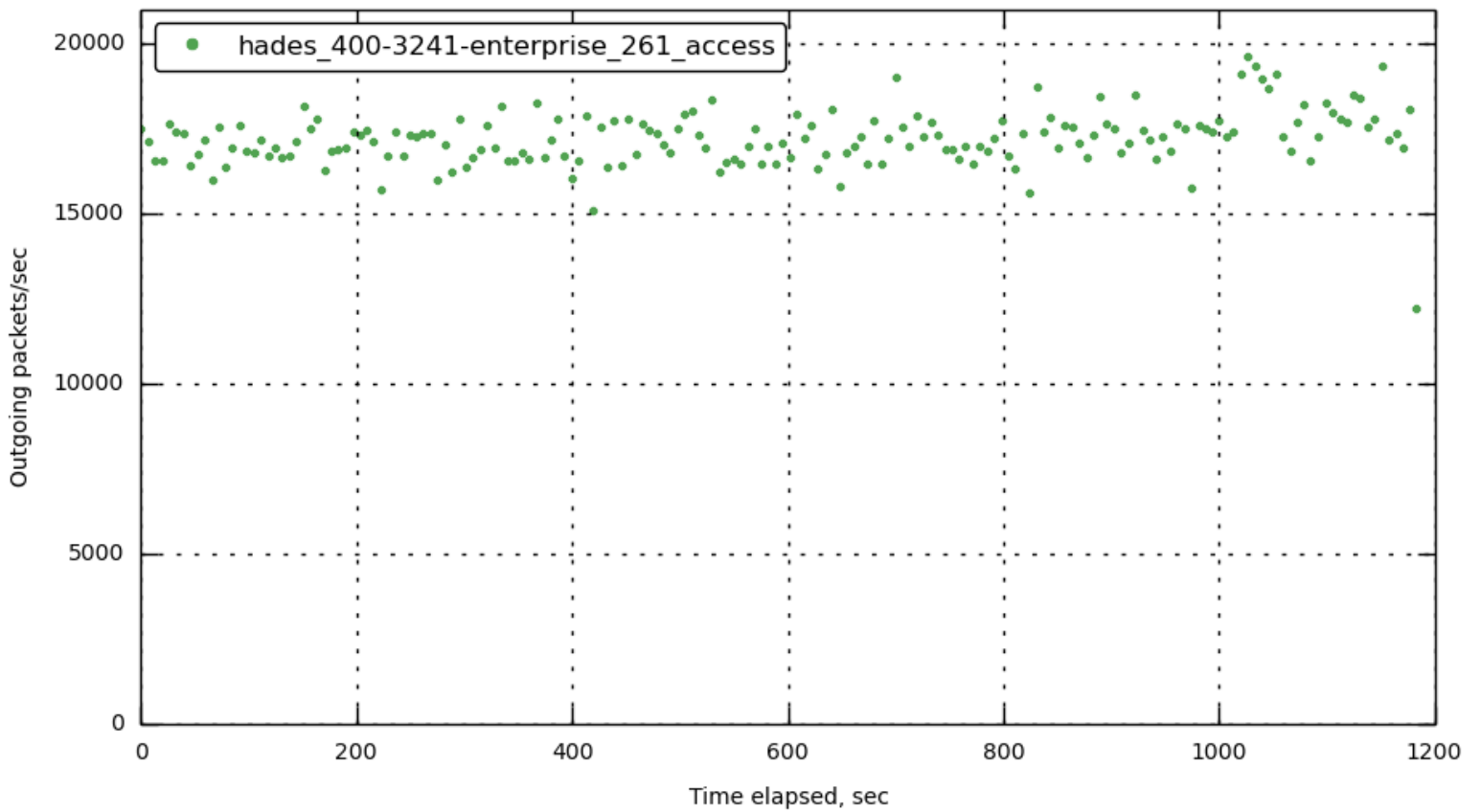
[172.23.100.72] out_packets_per_sec
