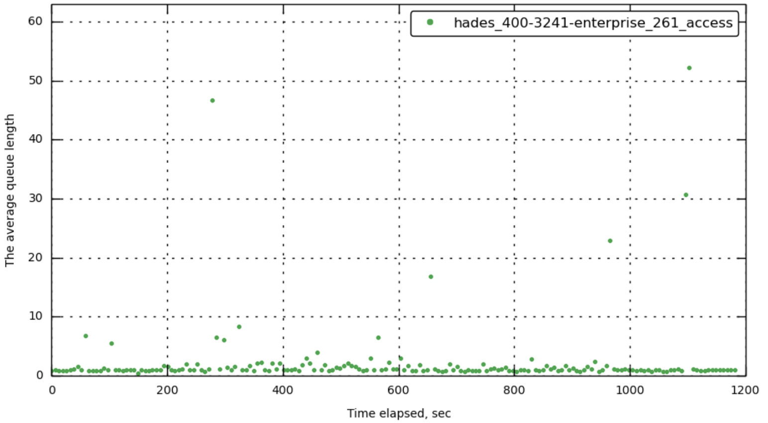
[172.23.100.71] data_avgqsz
