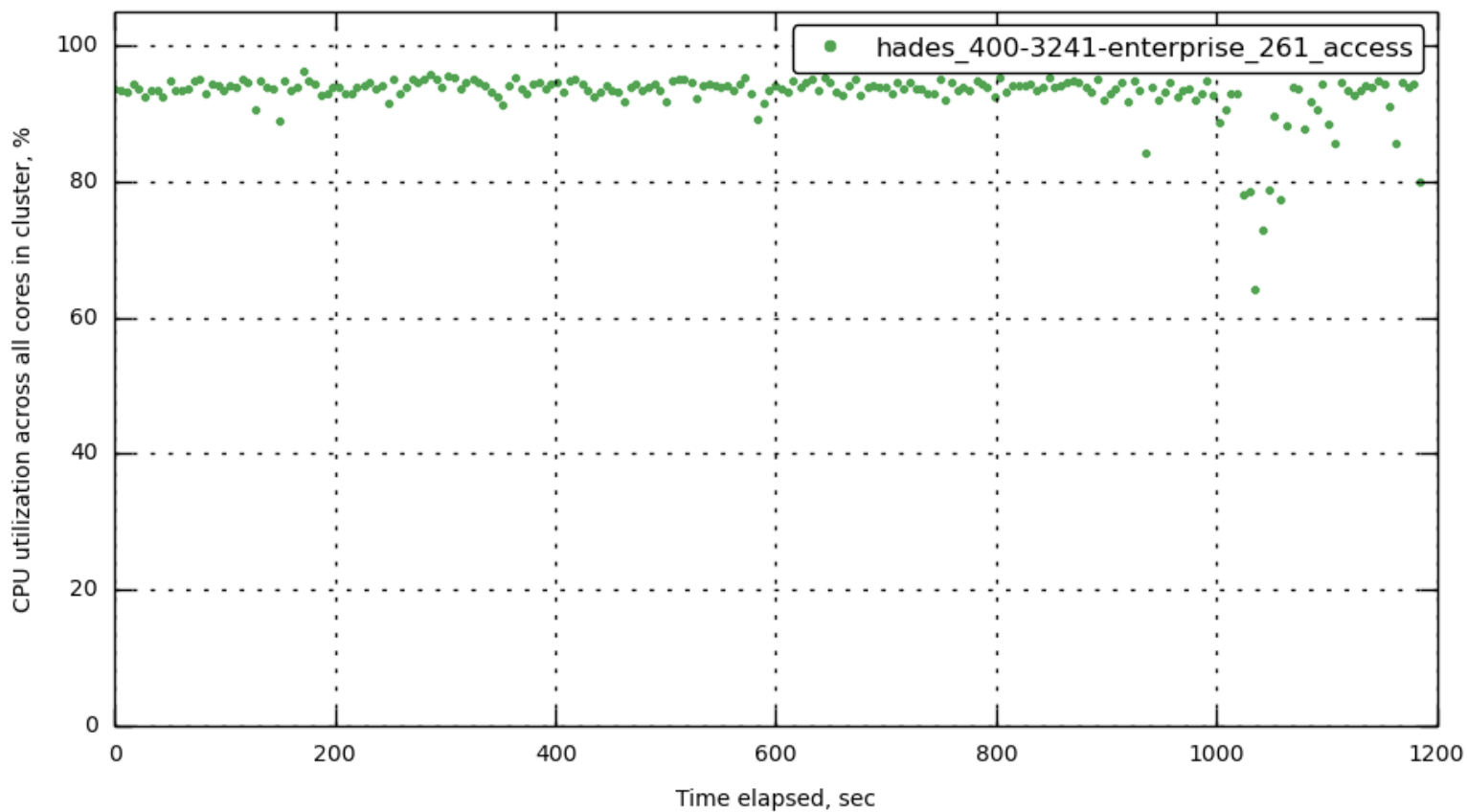
[bucket-1] cpu_utilization_rate
