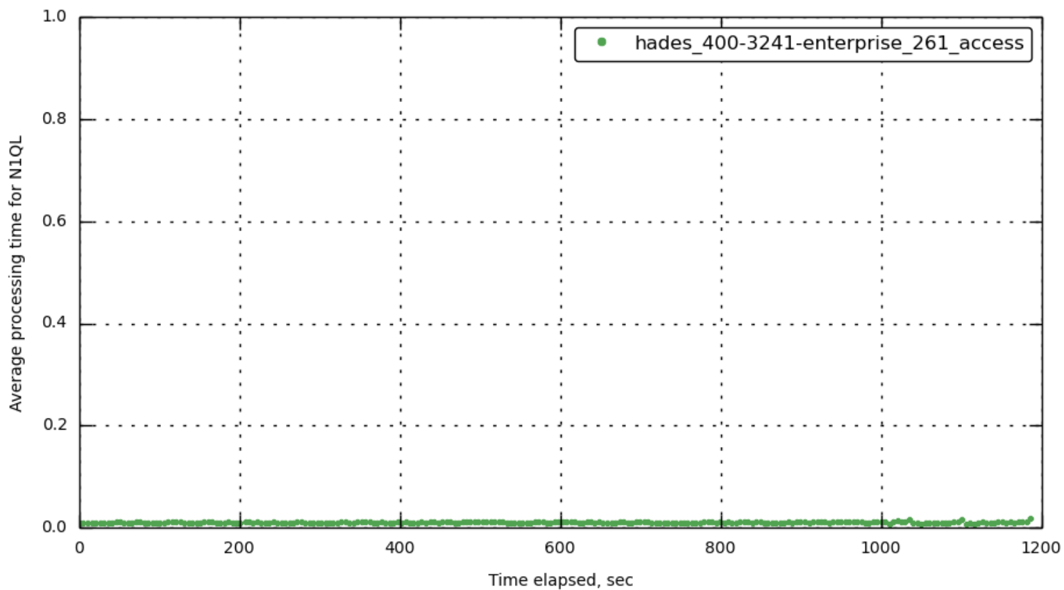
query_avg_req_time
