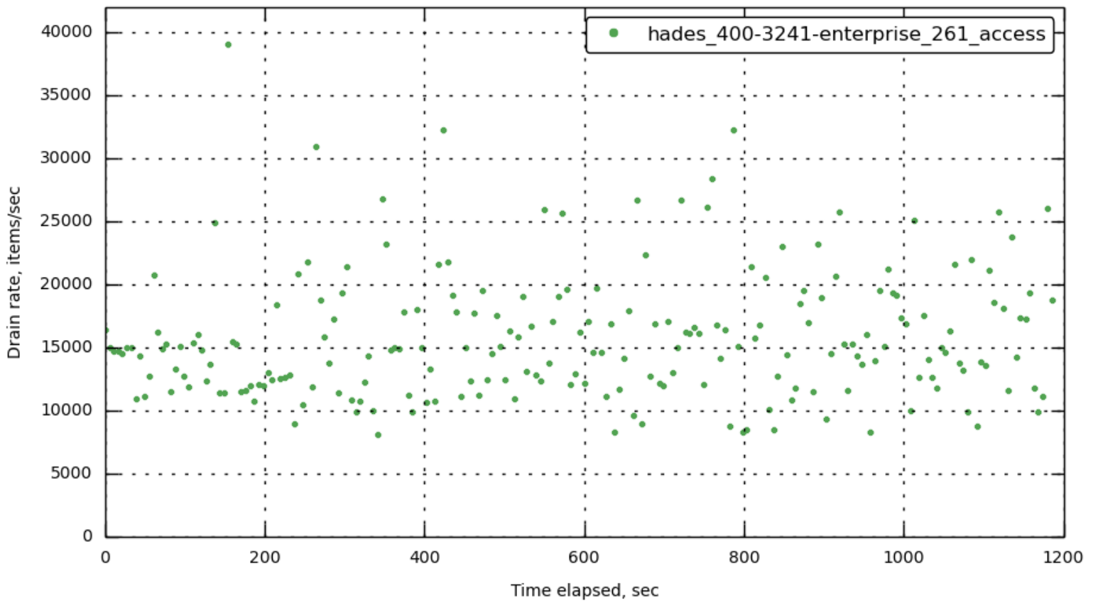
[bucket-1] ep_diskqueue_drain
