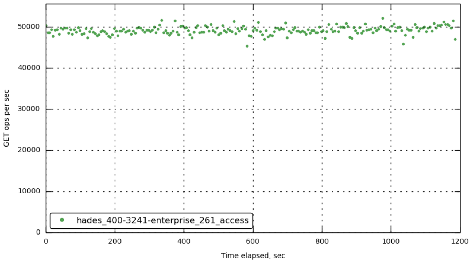
[bucket-1] cmd_get
