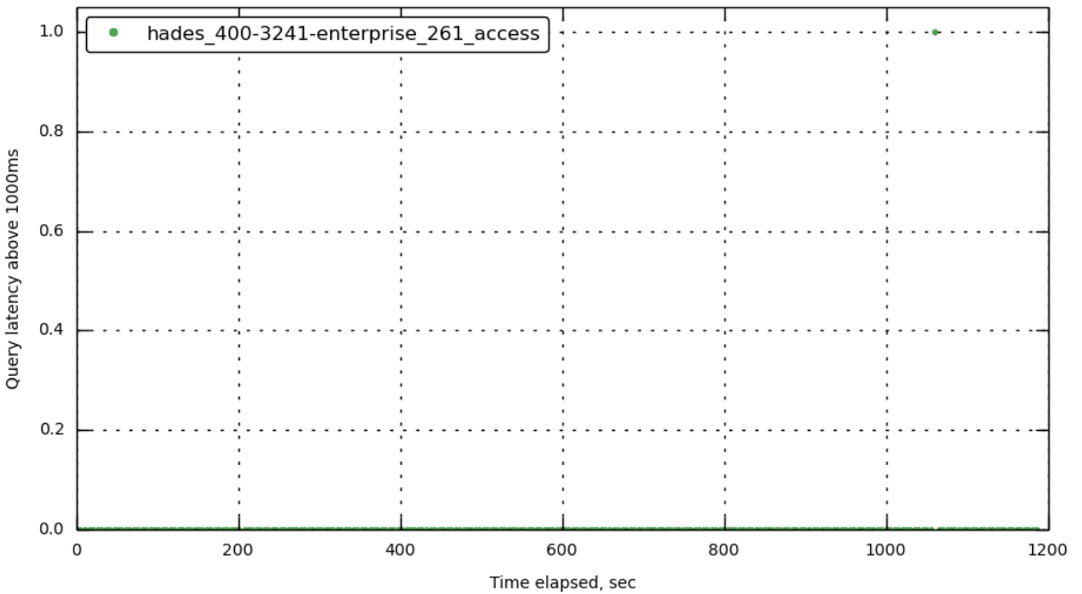
query_requests_1000ms
